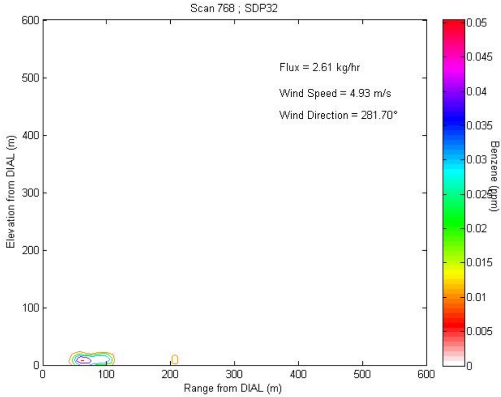
Figure 3.11a1 Contour plot of concentration profile for Scan 768 representing LOS1.
