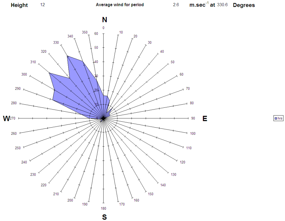
Figure A3.30 Wind rose for 12 th February during measurements from SDP28, 10:40 - 17:26
