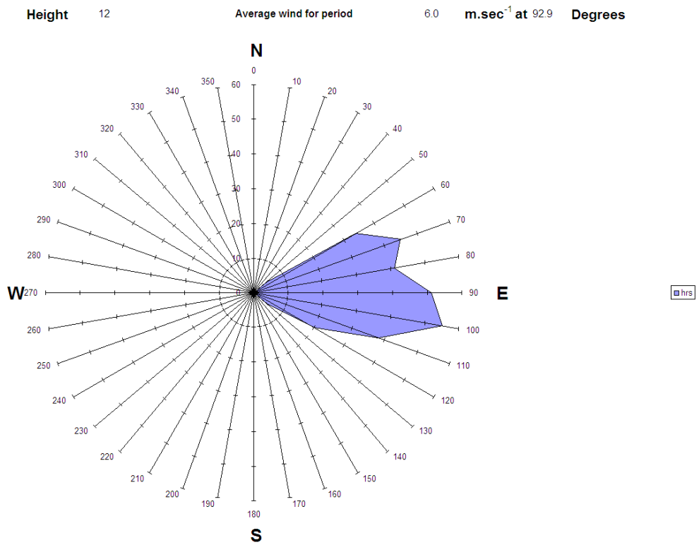
Figure A3.29 Wind rose for 11 th February during measurements from SDP27, 11:22 - 16:47
