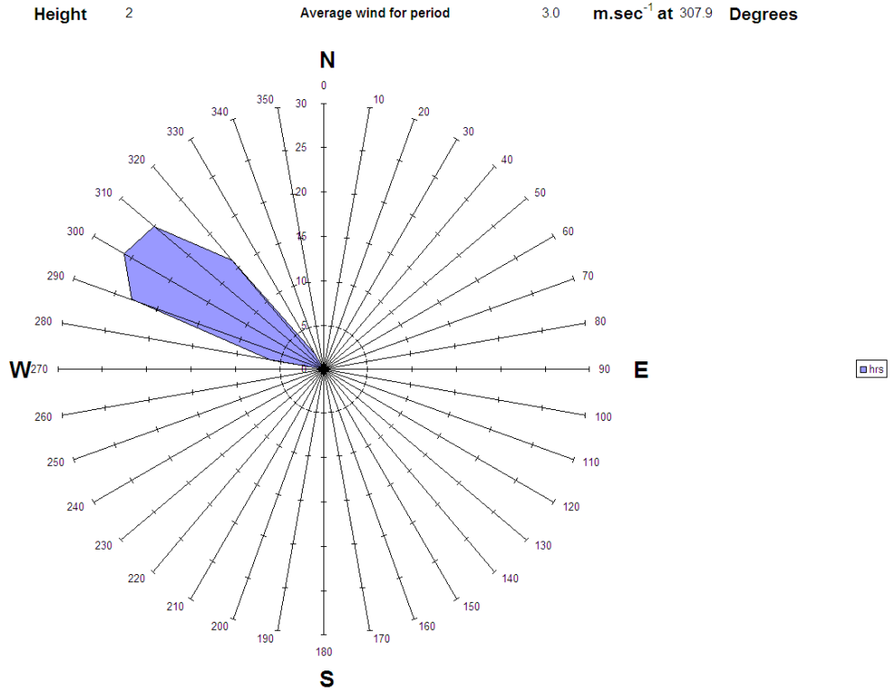
Figure A3.24 Wind rose for 5 th February during measurements from SDP22, 14:47 - 16:56
