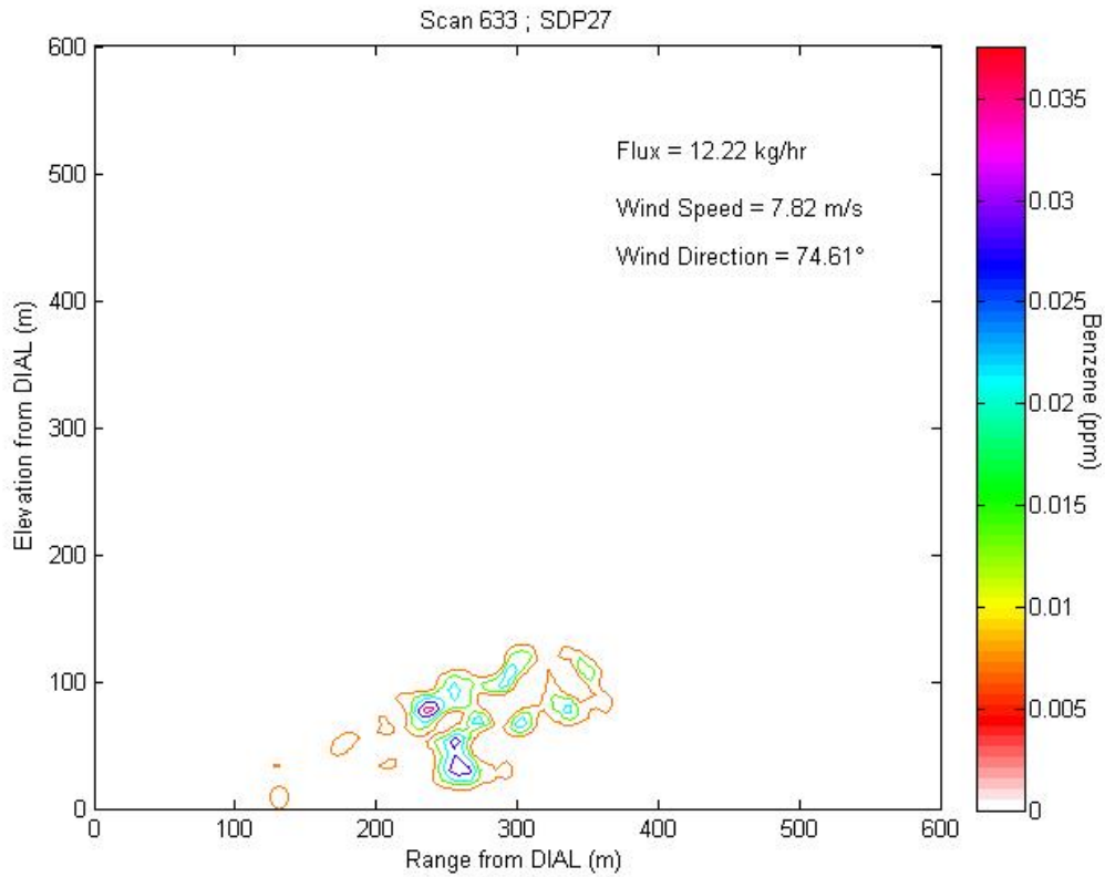
Figure 3.5b1 Contour plot of concentration profile for Scan 633 representing LOS2.
