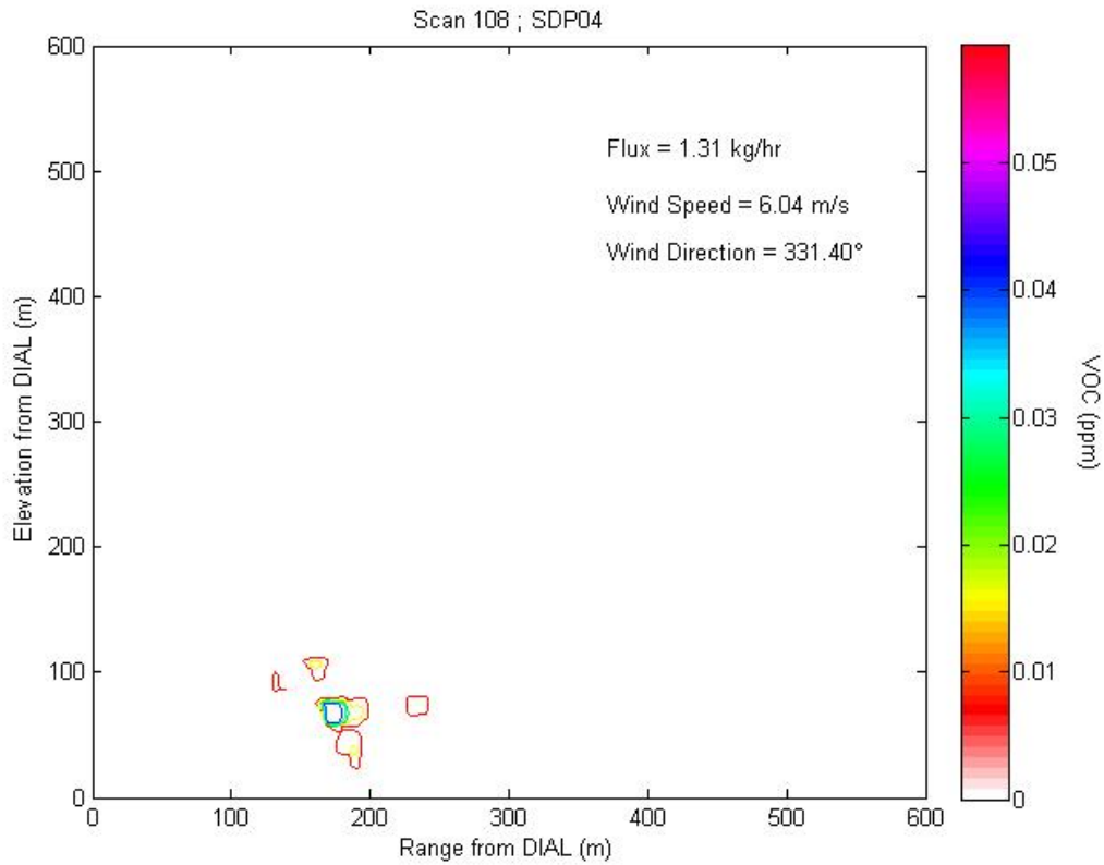
Figure 2.4b1 Contour plot of concentration profile for Scan 108 representing LOS4.
