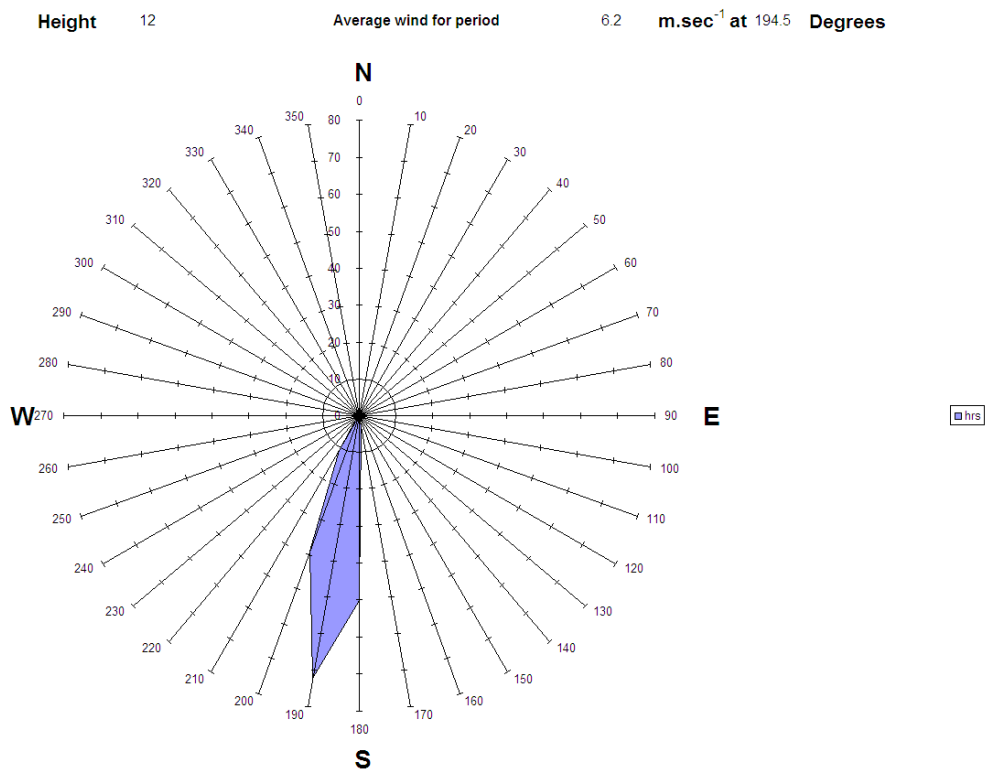
Figure A3.7 Wind rose for 19 th January during measurements from SDP6, 10:27 - 14:18
