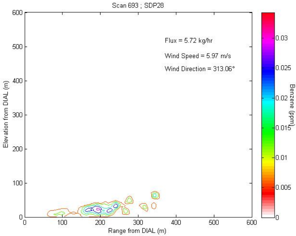
Figure 3.8a1 Contour plot of concentration profile for Scan 693 representing LOS1.
