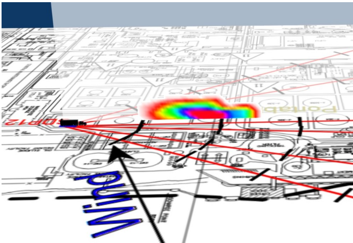
Figure 2.17c2 Visualisation of emission rate measured for Scan 415 representing LOS5.
