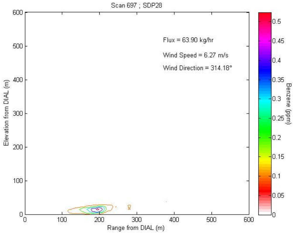
Figure 3.8b1 Contour plot of concentration profile for Scan 697 representing LOS2.
