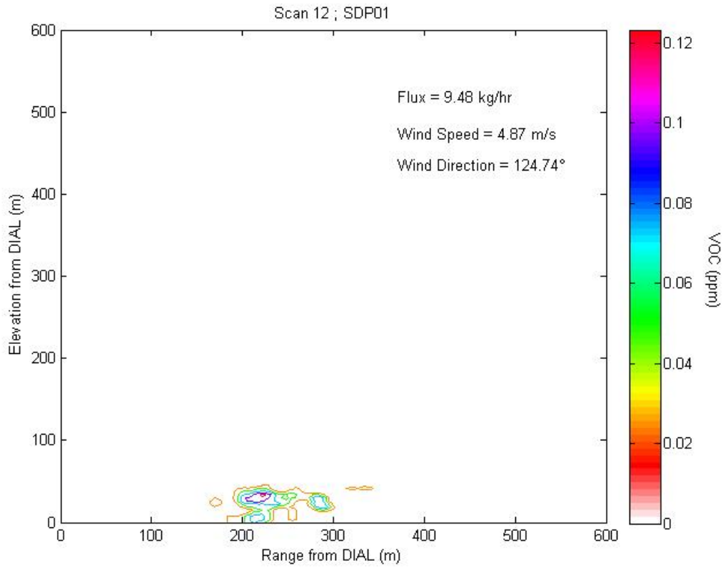
Figure 2.1a1 Contour plot of concentration profile for Scan 12 representing LOS1.
