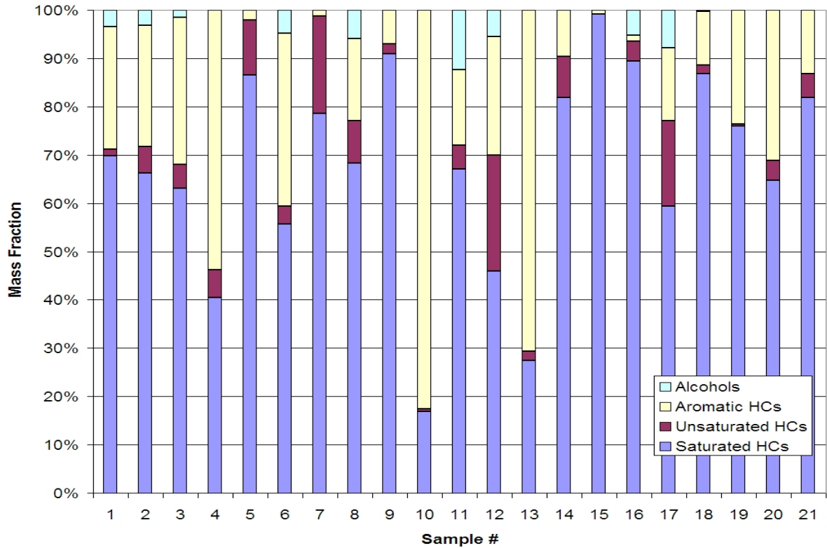
Figure A2.2 Percentage by mass of main types of VOCs in ATD samples
