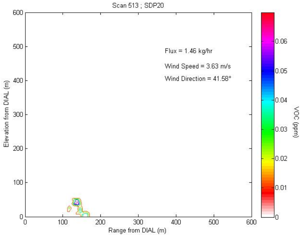
Figure 2.21a1 Contour plot of concentration profile for Scan 513 representing LOS2.
