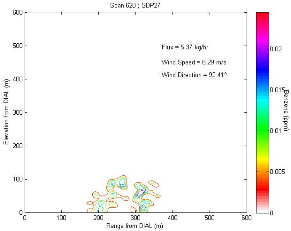
Figure 3.5a1 Contour plot of concentration profile for Scan 620 representing LOS1.
