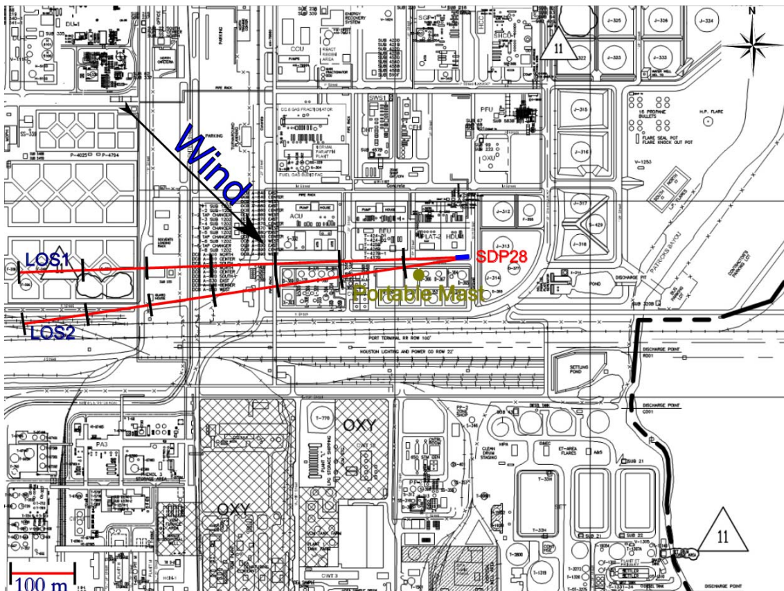
Figure 3.8 Measurement configuration for location SDP28 on 15 th of February.
