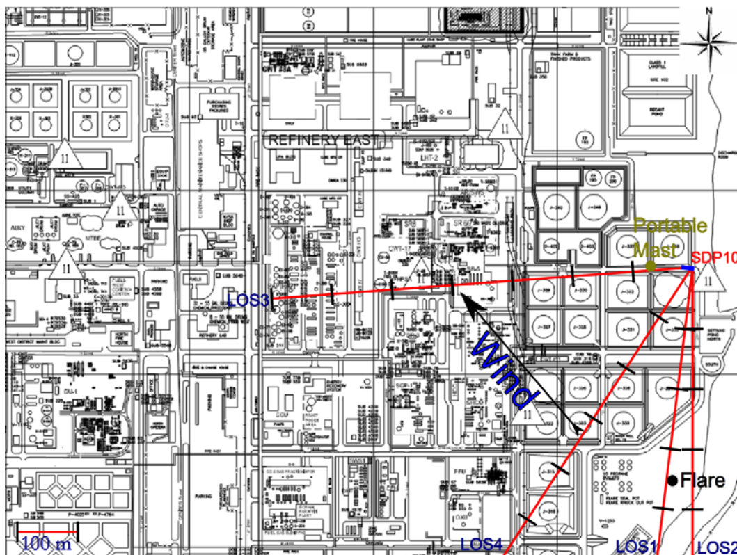
Figure 2.10 Measurement configuration for location SDP10 on 22 nd of January.
