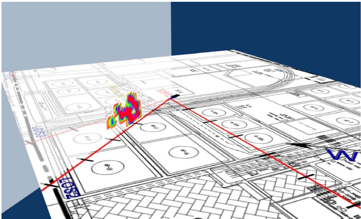
Figure 2.3b2 Visualisation of emission rate measured for Scan 73 representing LOS2.
