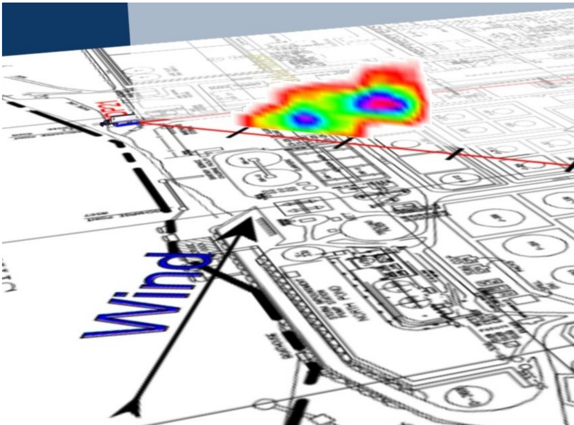
Figure 2.22a2 Visualisation of emission rate measured for Scan 529 representing LOS1.
