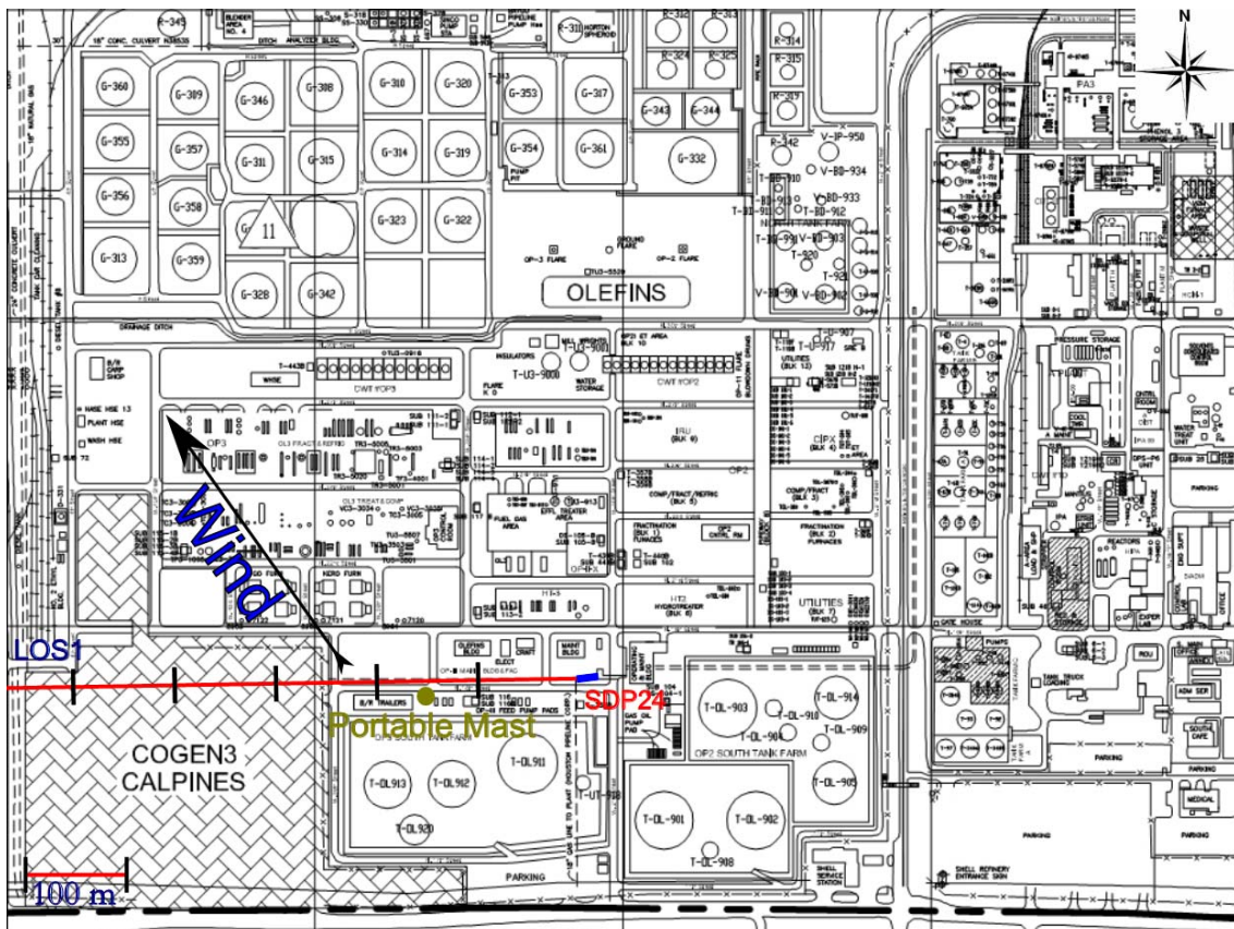
Figure 3.2 Measurement configuration for location SDP24 on 8 th of February.
