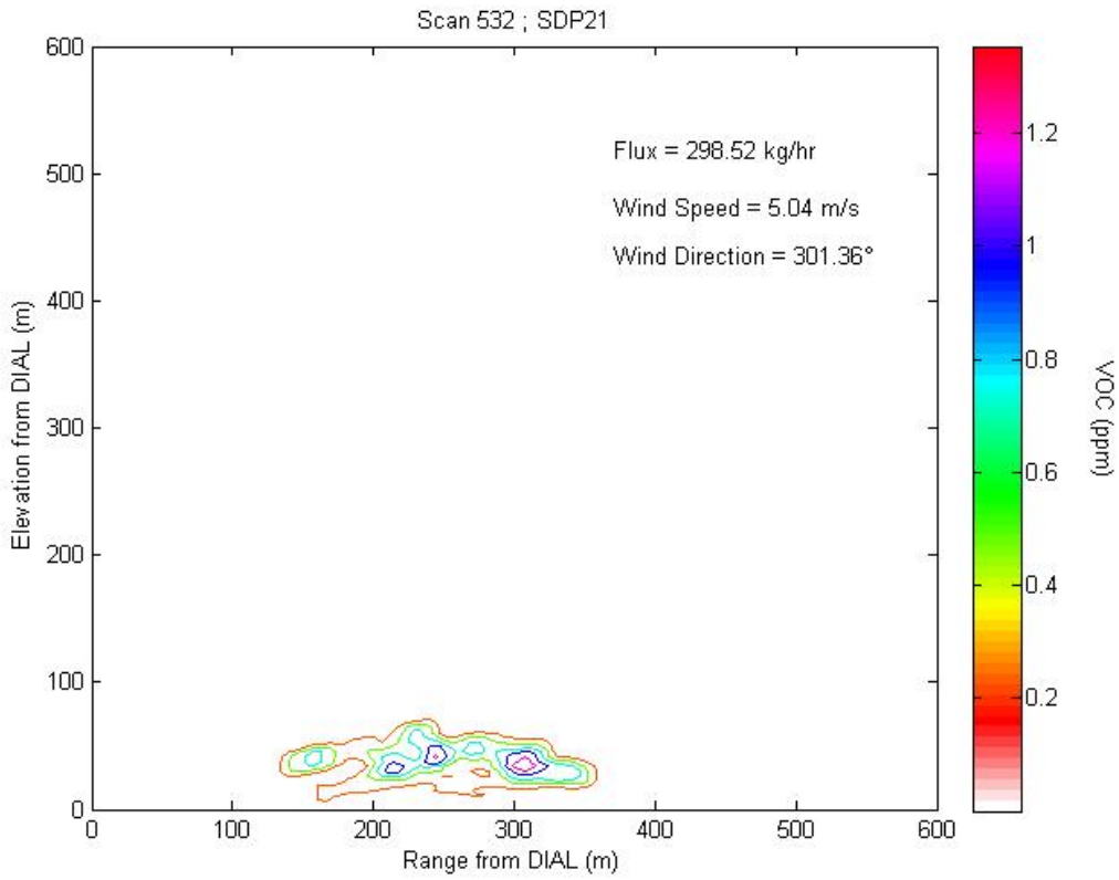
Figure 2.22b1 Contour plot of concentration profile for Scan 532 representing LOS2.
