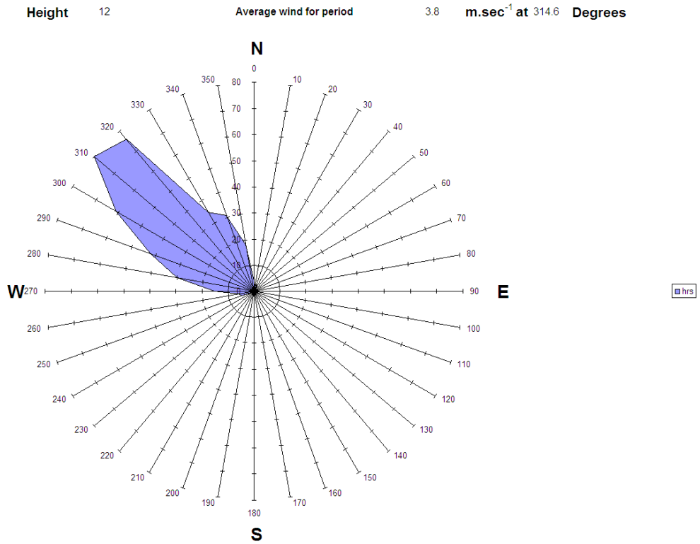
Figure A3.32 Wind rose for 15 th February during measurements from SDP28, 10:18 - 17:13
