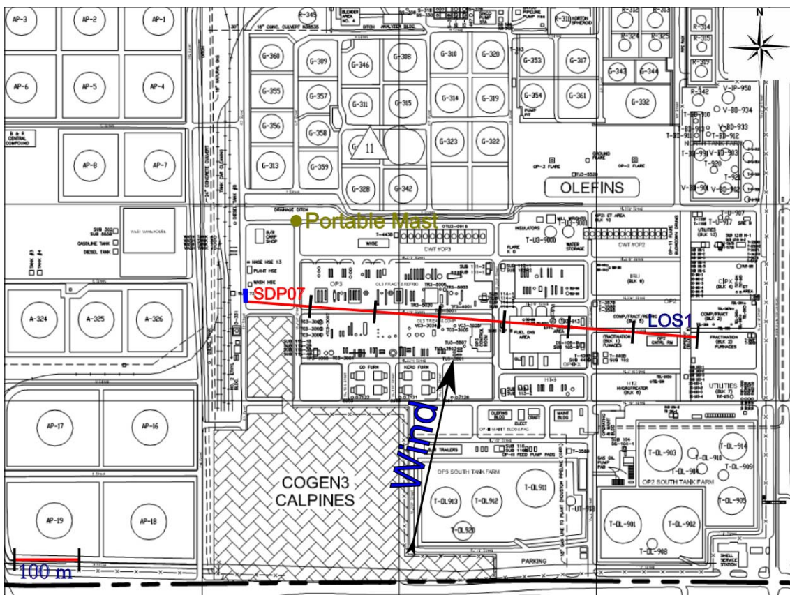
Figure 2.7 Measurement configuration for location SDP07 on 19 th of January.
