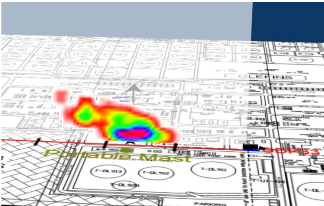
Figure 3.12a2 Visualisation of emission rate measured for Scan 778 representing LOS1.
