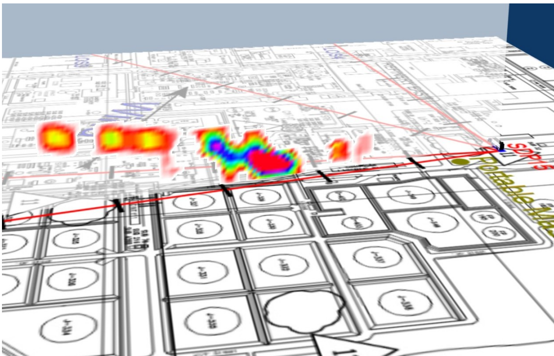
Figure 2.15a2 Visualisation of emission rate measured for Scan 365 representing LOS2.
