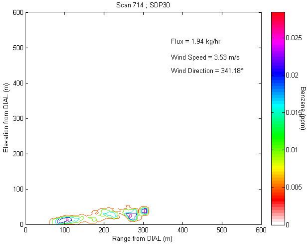
Figure 3.9a1 Contour plot of concentration profile for Scan 714 representing LOS1.
