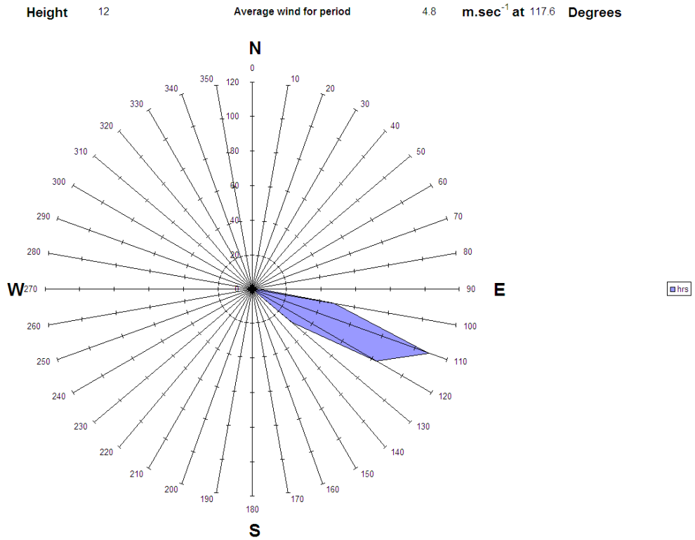
Figure A3.2 Wind rose for 13 th January during measurements from SDP1, 12:24 - 17:36
