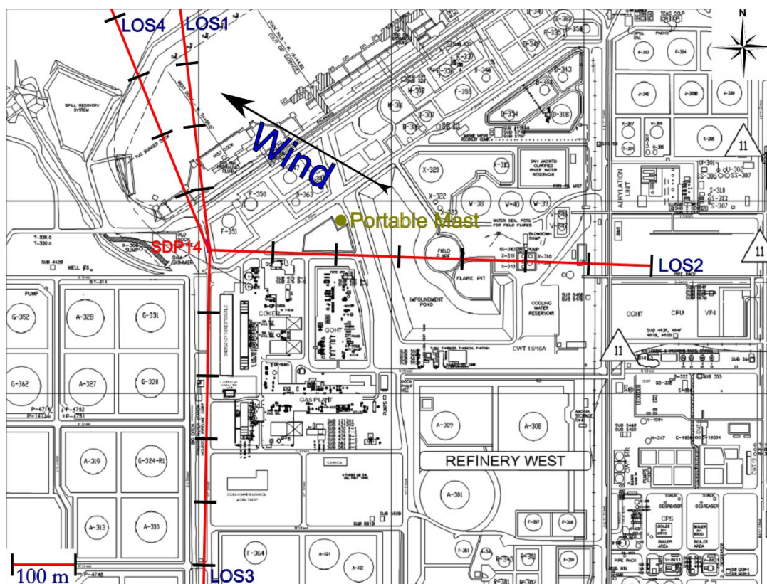
Figure 2.14 Measurement configuration for location SDP14 on 27 th of January.
