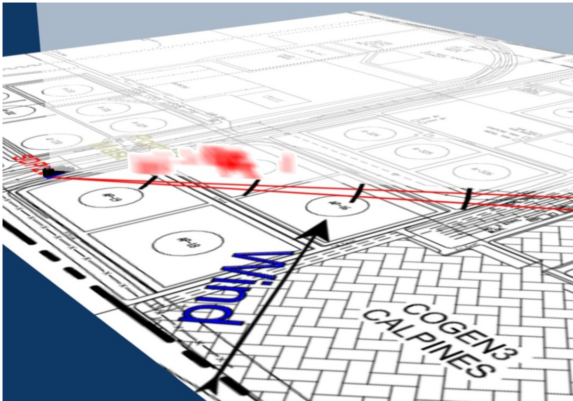
Figure 3.1a2 Visualisation of emission rate measured for Scan 545 representing LOS1.
