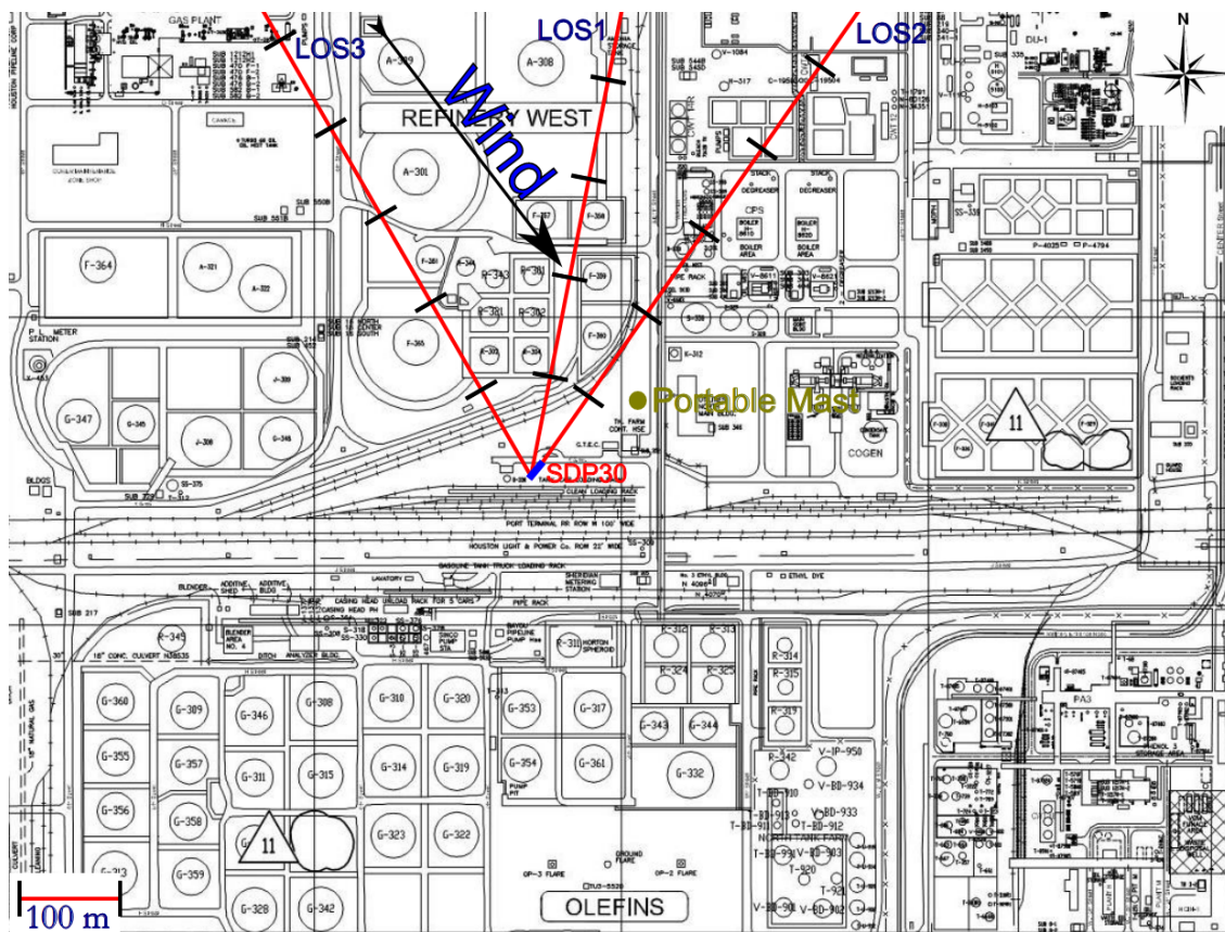
Figure 3.9 Measurement configuration for location SDP30 on 16 th of February.
