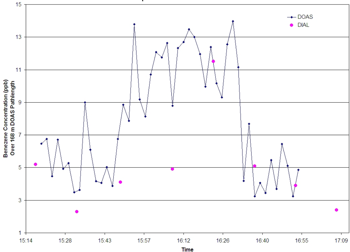
Figure 5.1 DIAL and DOAS measurements comparison on the 8 th of February.
