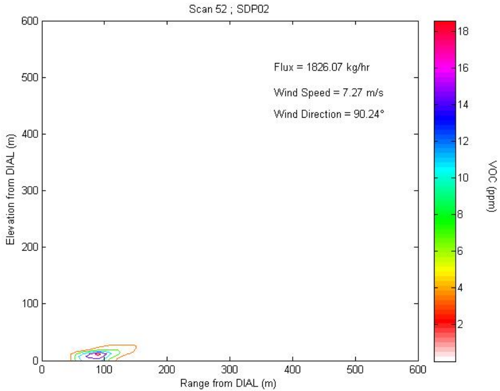
Figure 2.2c1 Contour plot of concentration profile for Scan 52 representing LOS2.
