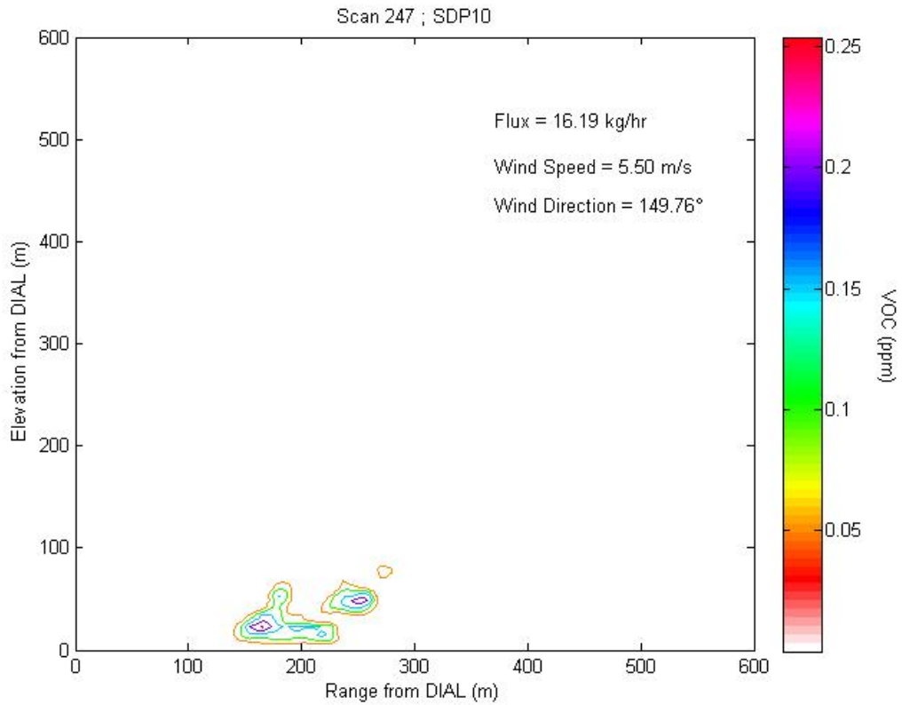
Figure 2.10a1 Contour plot of concentration profile for Scan 247 representing LOS3.
