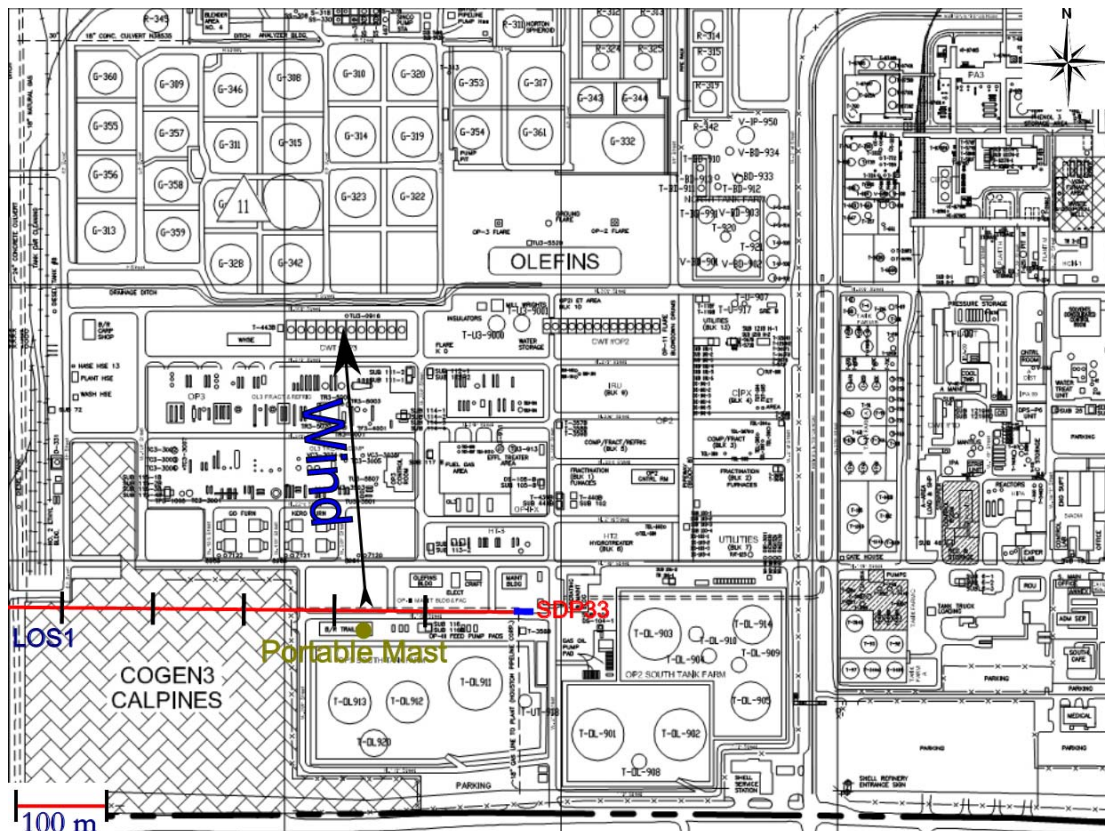
Figure 3.12 Measurement configuration for location SDP33 on 23 rd of March.
