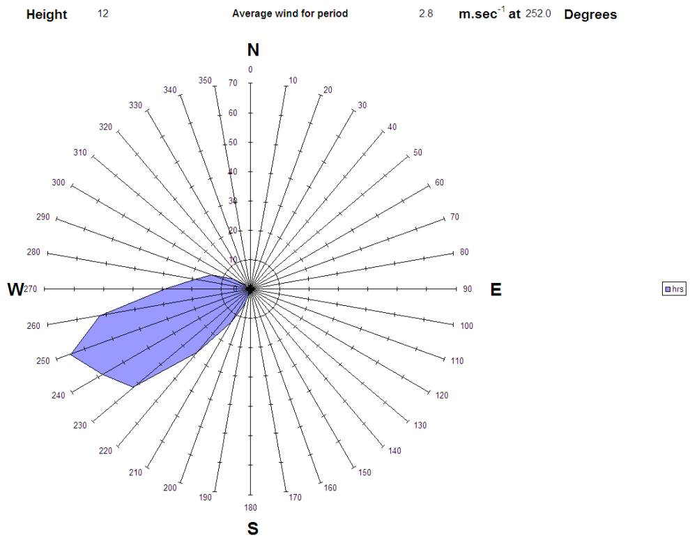
Figure A3.31 Wind rose for 13 th February during measurements from SDP29, 10:53 - 16:42
