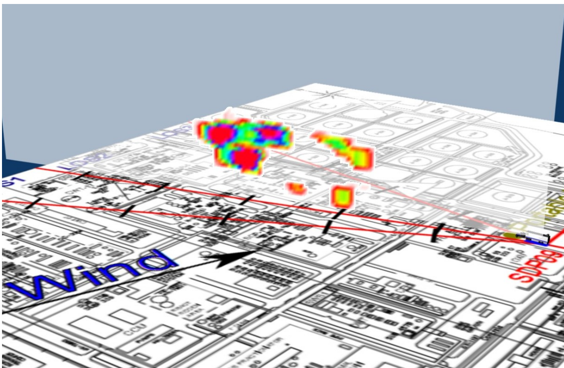
Figure 2.9a2 Visualisation of emission rate measured for Scan 209 representing LOS2.
