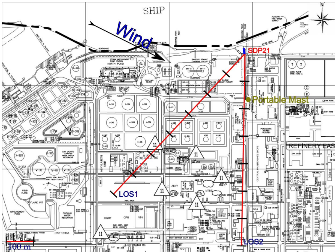
Figure 2.22 Measurement configuration for location SDP21 on 5 th of February.
