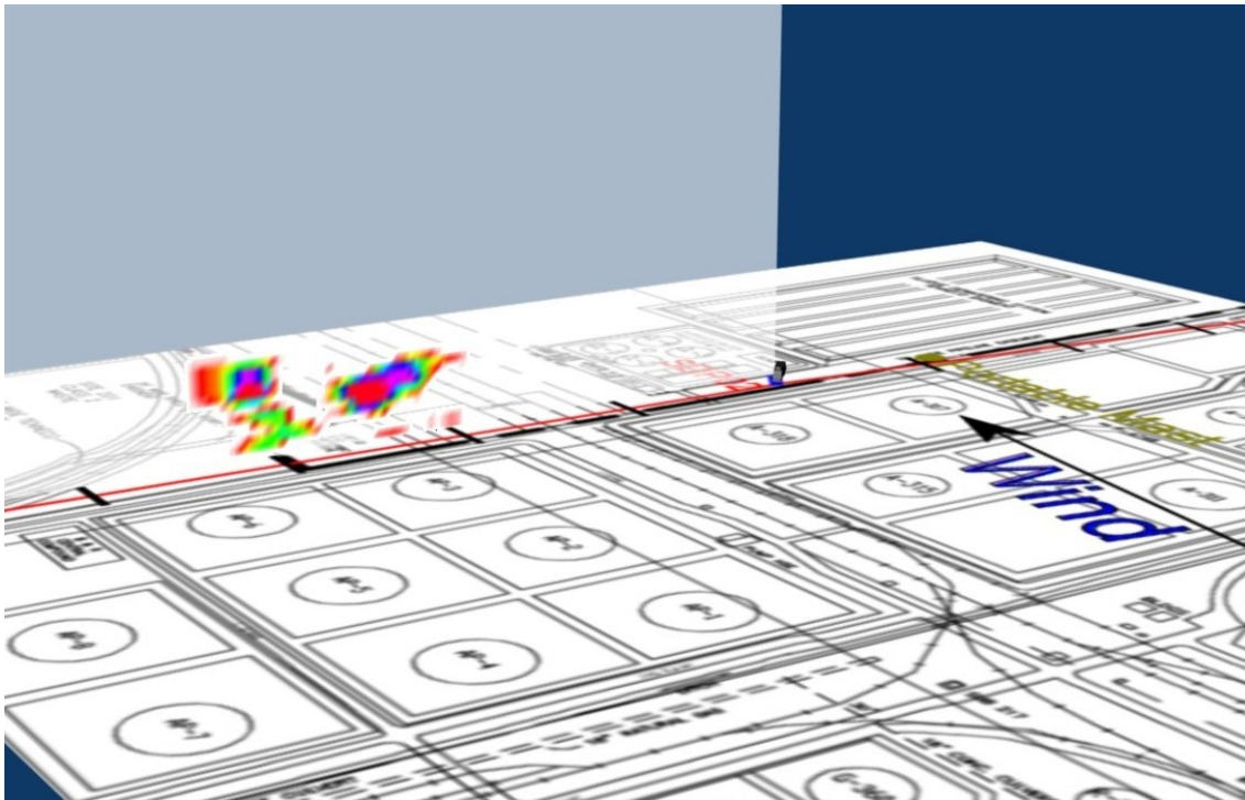
Figure 2.2b2 Visualisation of emission rate measured for Scan 44 representing LOS2.
