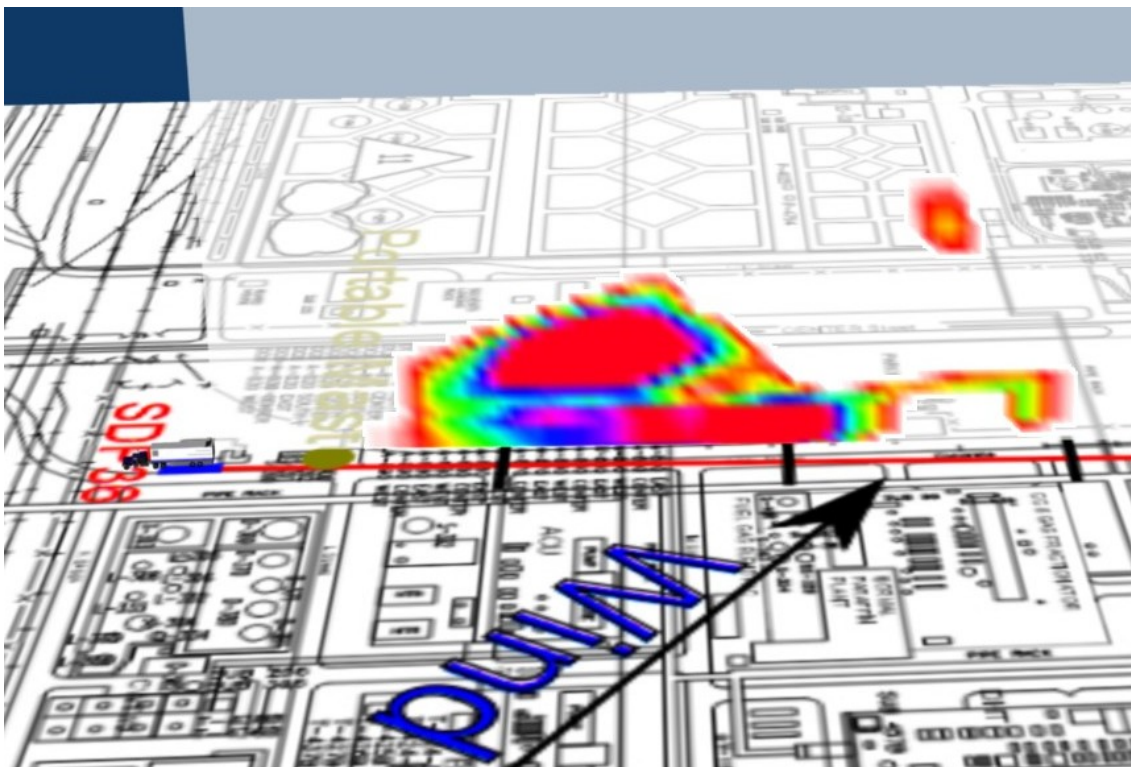
Figure 2.26a2 Visualisation of emission rate measured for Scan 836 representing LOS1.
