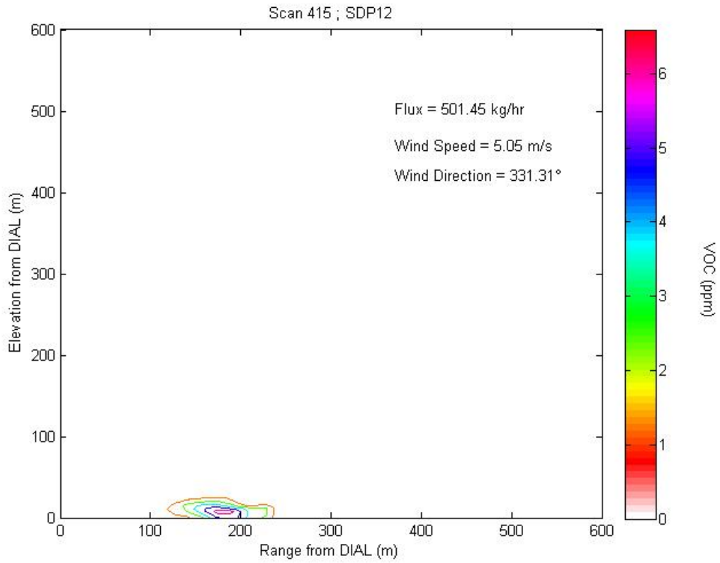
Figure 2.17c1 Contour plot of concentration profile for Scan 415 representing LOS5.
