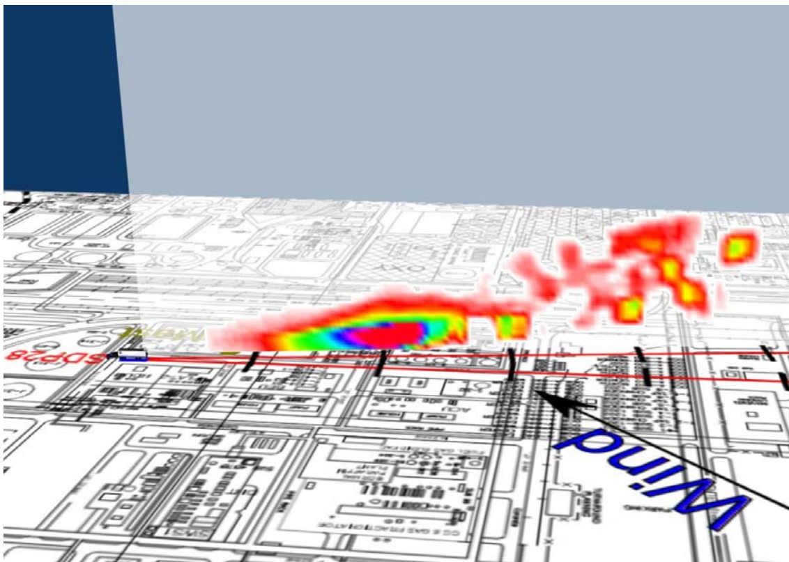
Figure 3.8b2 Visualisation of emission rate measured for Scan 697 representing LOS2.
