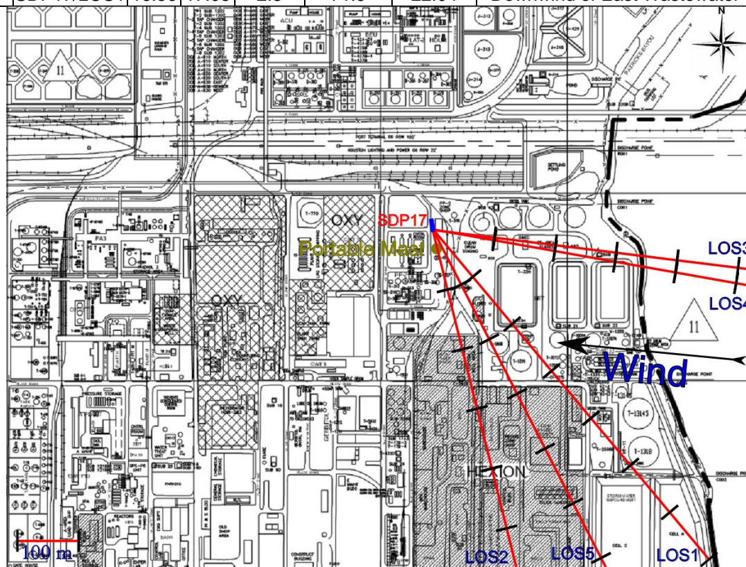
Figure 2.18 Measurement configuration for location SDP17 on 1 st of February.
