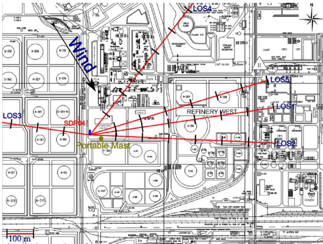
Figure 2.4 Measurement configuration for location SDP04 on 16 th of January.
