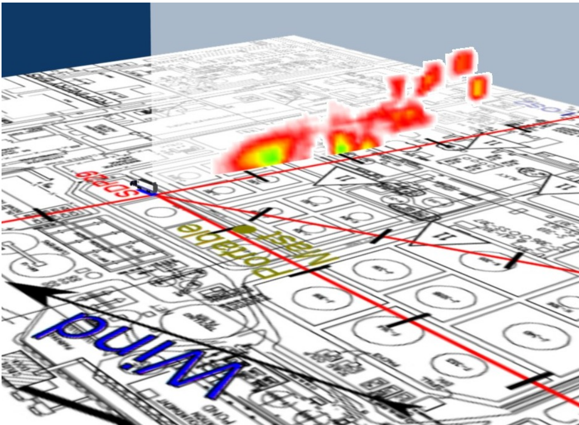
Figure 3.7a2 Visualisation of emission rate measured for Scan 669 representing LOS2.
