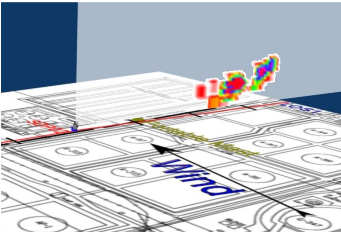
Figure 2.2a2 Visualisation of emission rate measured for Scan 39 representing LOS1.
