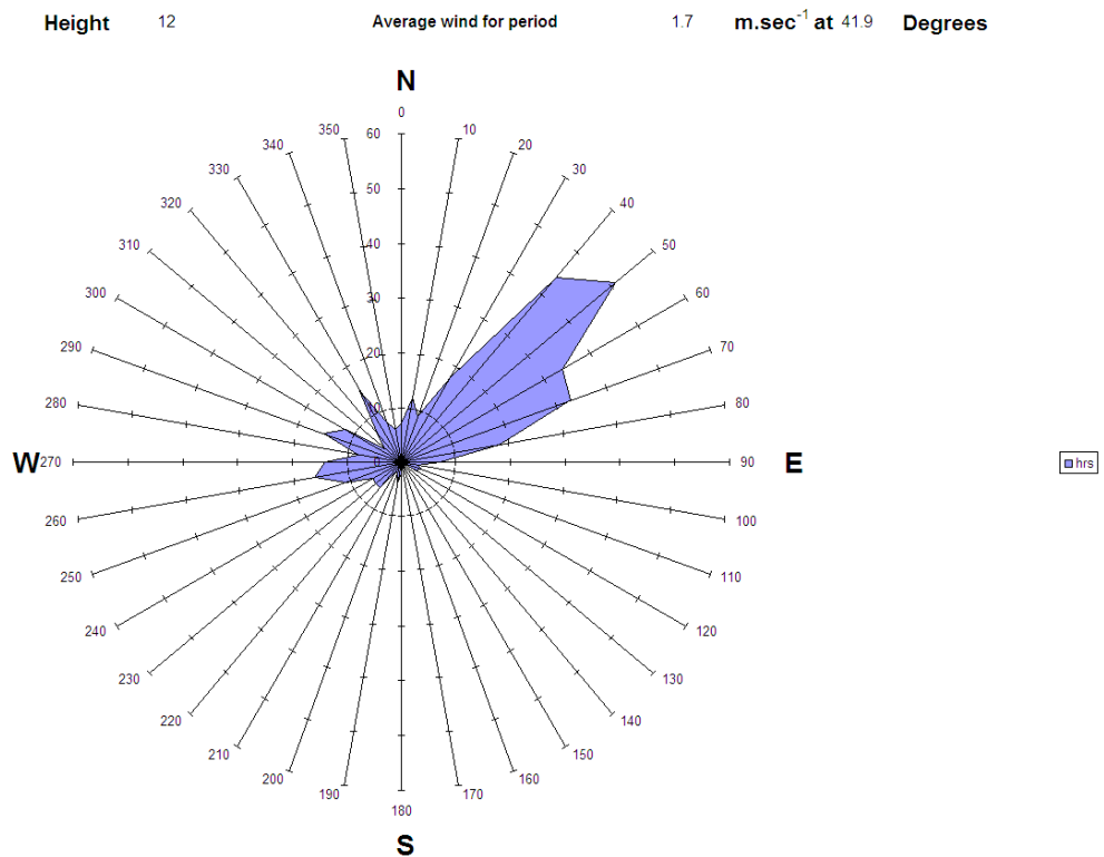
Figure A3.40 Wind rose for 29 th March during the last day of the campaign, 9:00 - 16:30
