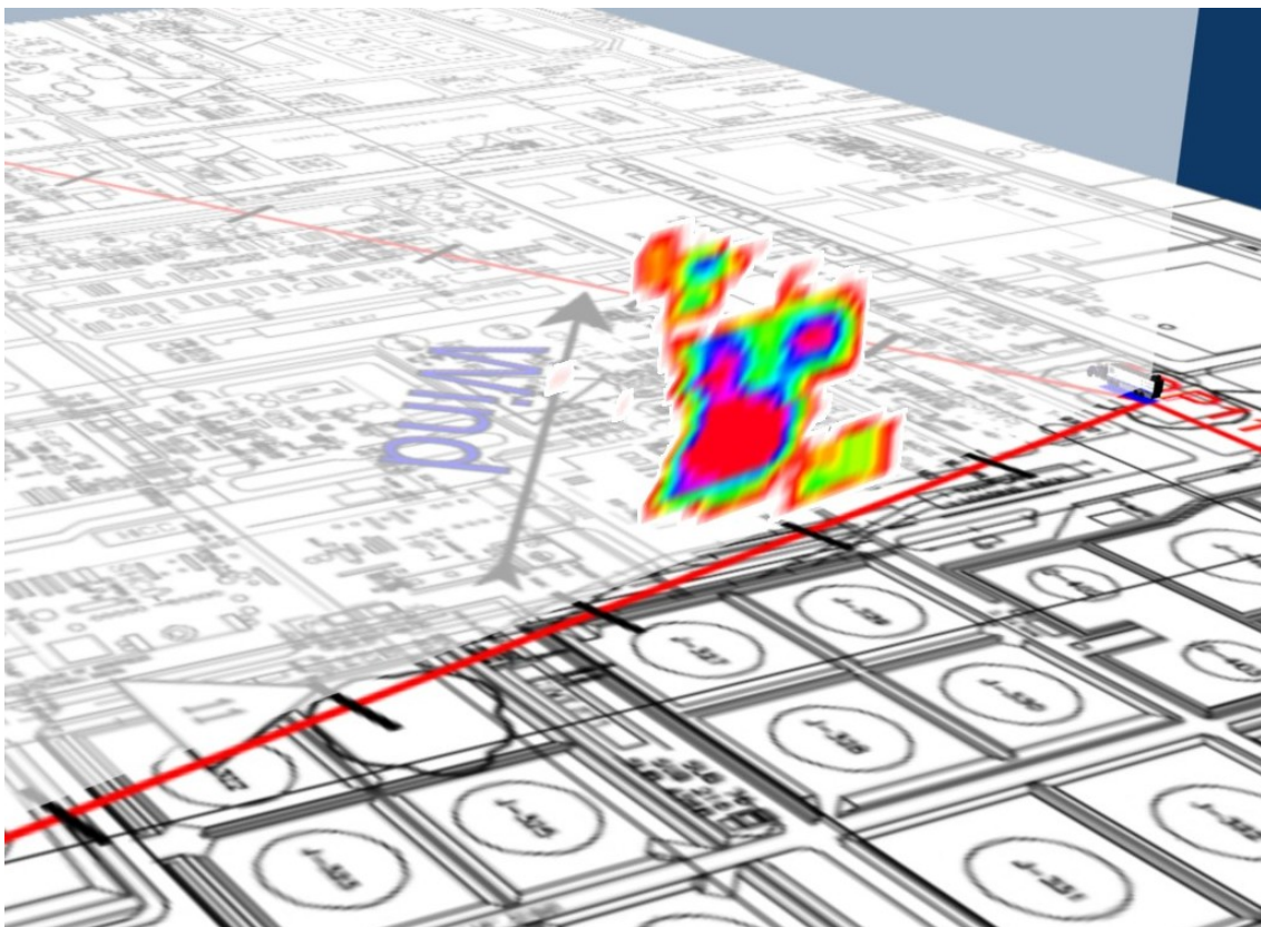
Figure 2.11a2 Visualisation of emission rate measured for Scan 263 representing LOS2.
