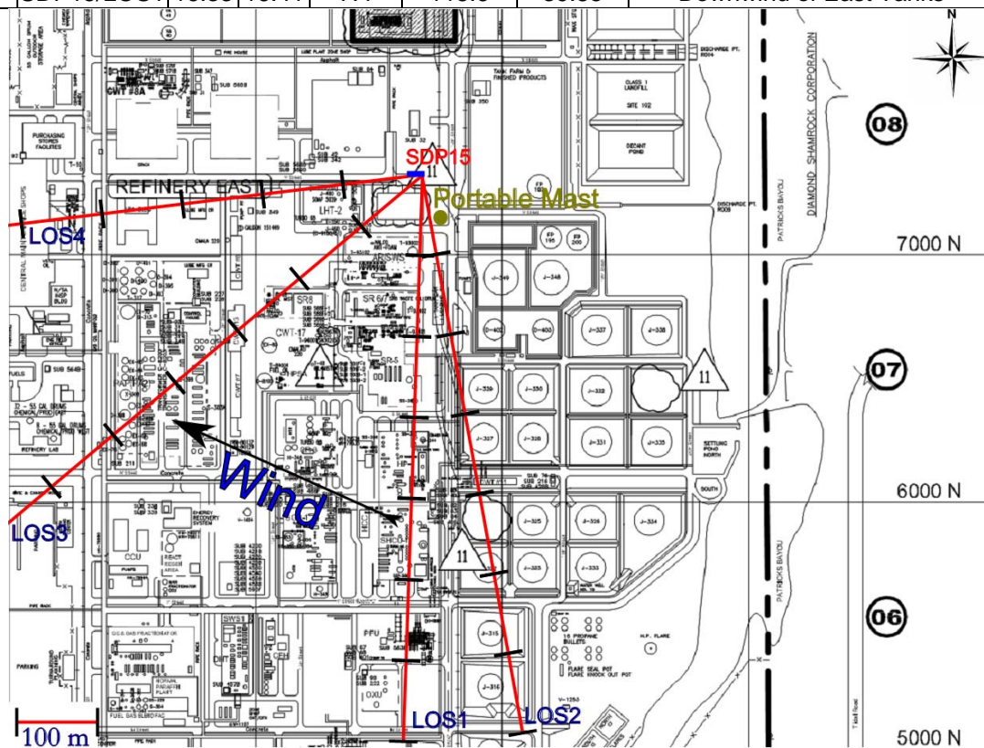
Figure 2.15 Measurement configuration for location SDP15 on 28 th of January.
