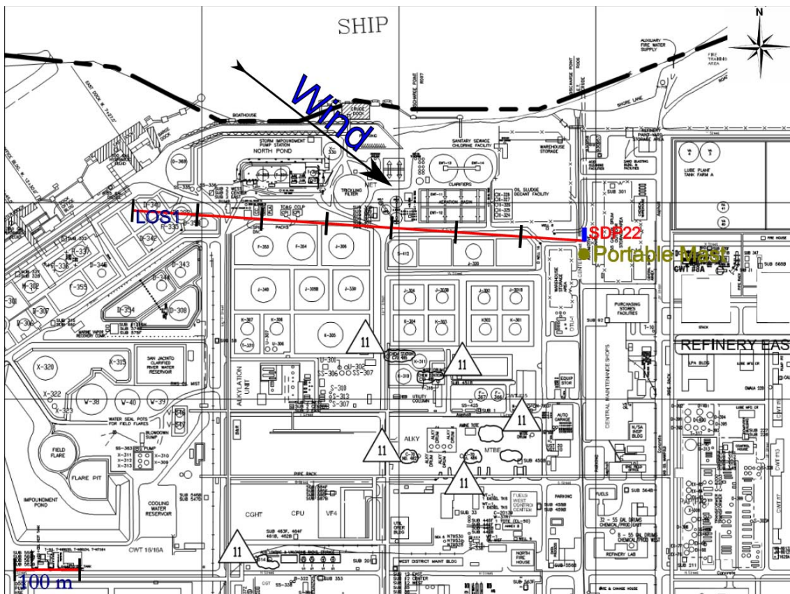
Figure 2.23 Measurement configuration for location SDP22 on 5 th of February.
