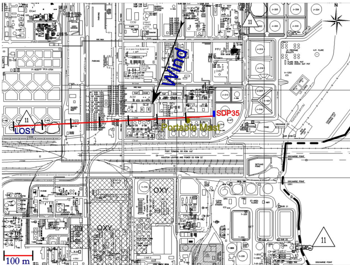
Figure 2.25 Measurement configuration for location SDP35 on 26 th of March.
