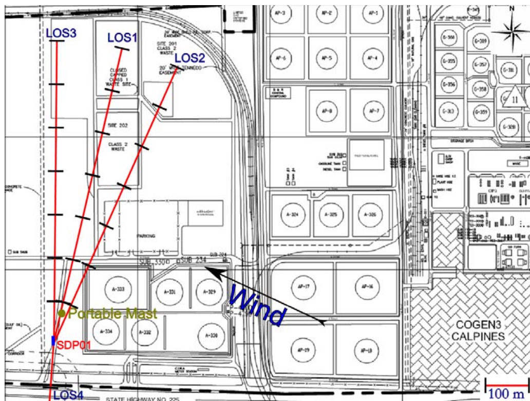
Figure 2.1 Measurement configuration for location SDP01 on 13 th of January.
