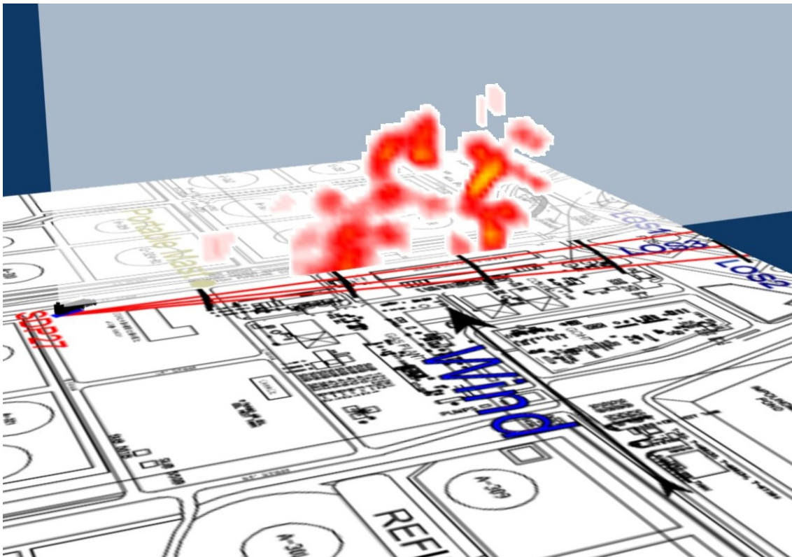
Figure 3.5a2 Visualisation of emission rate measured for Scan 620 representing LOS1.
