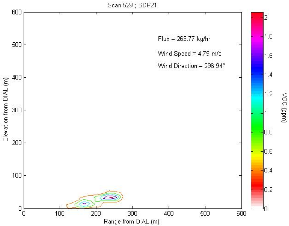
Figure 2.22a1 Contour plot of concentration profile for Scan 529 representing LOS1.
