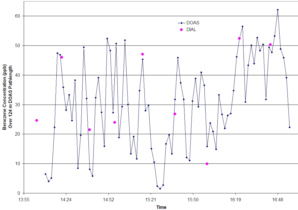
Figure 5.3 DIAL and DOAS measurements comparison on the 10 th of February from 14:00.
