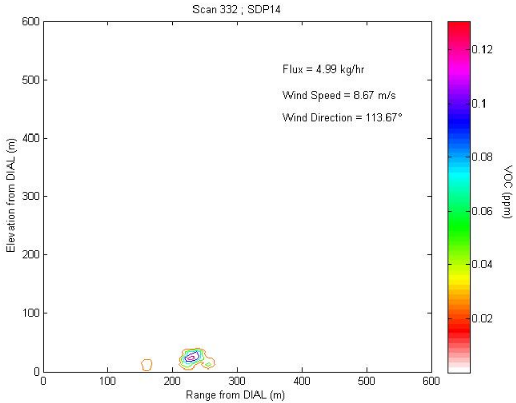
Figure 2.14a1 Contour plot of concentration profile for Scan 332 representing LOS1.
