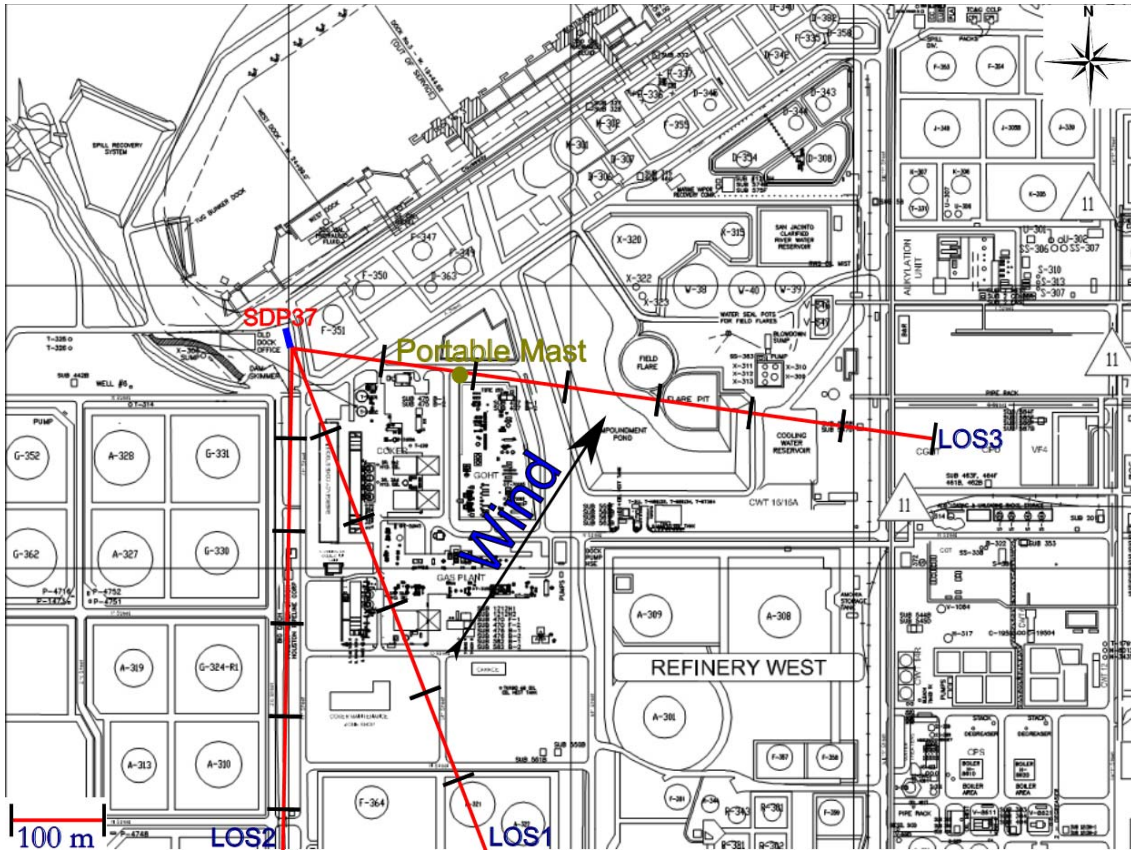
Figure 2.27 Measurement configuration for location SDP37 on 27 th of March.
