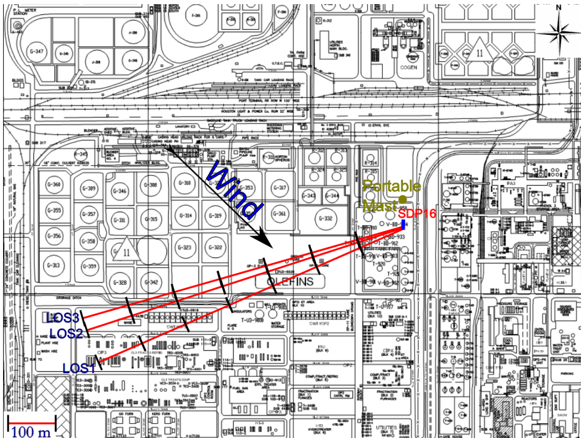
Figure 2.16 Measurement configuration for location SDP16 on 29 th of January.
