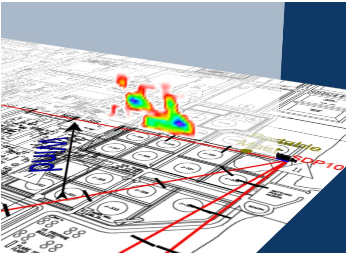
Figure 2.10a2 Visualisation of emission rate measured for Scan 247 representing LOS3.
