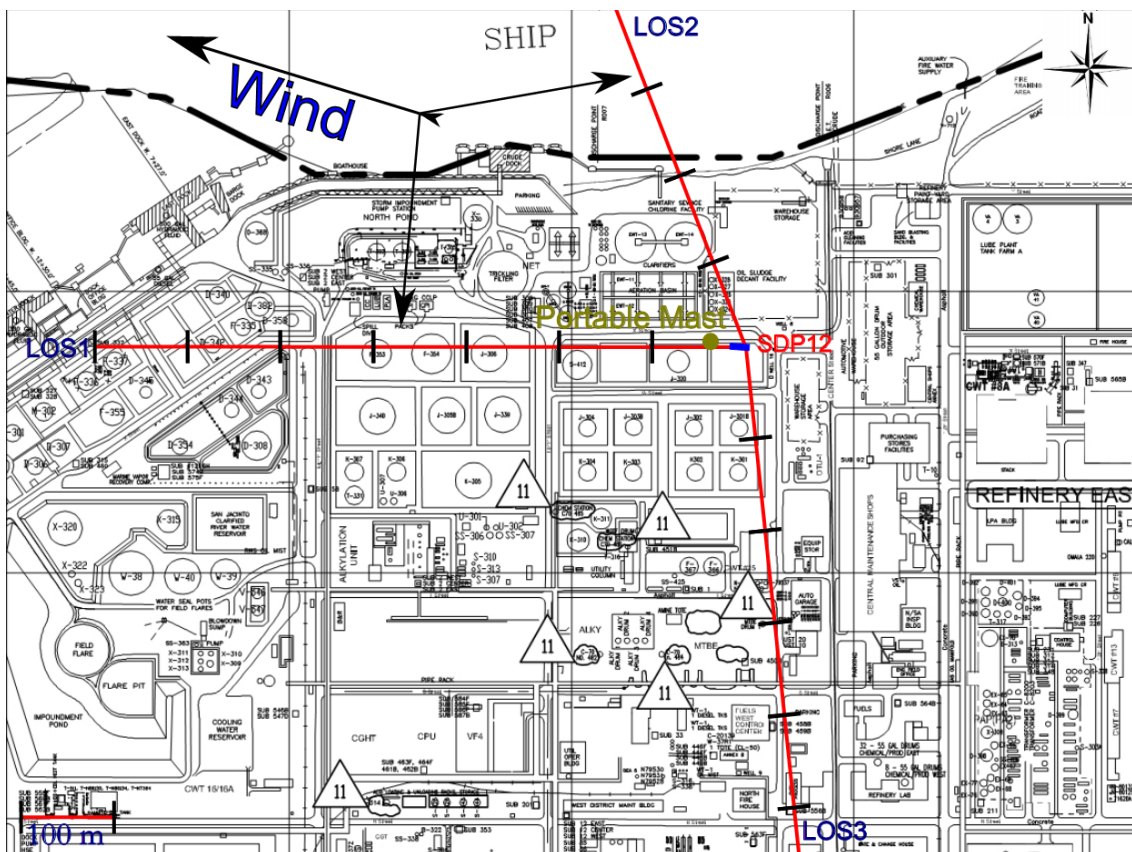
Figure 2.12 Measurement configuration for location SDP12 on 25 th of January.
