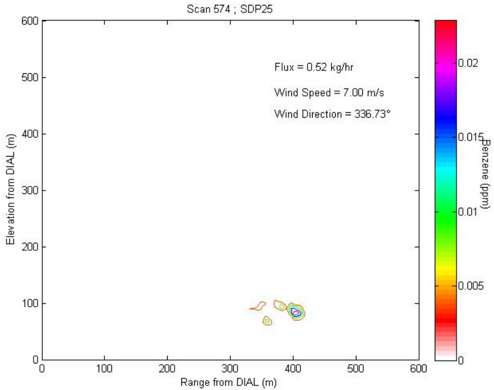
Figure 3.3b1 Contour plot of concentration profile for Scan 574 representing LOS2.
