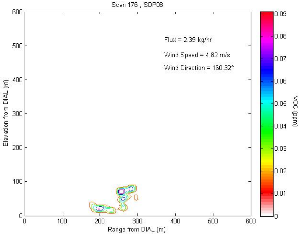
Figure 2.8a1 Contour plot of concentration profile for Scan 176 representing LOS1.
