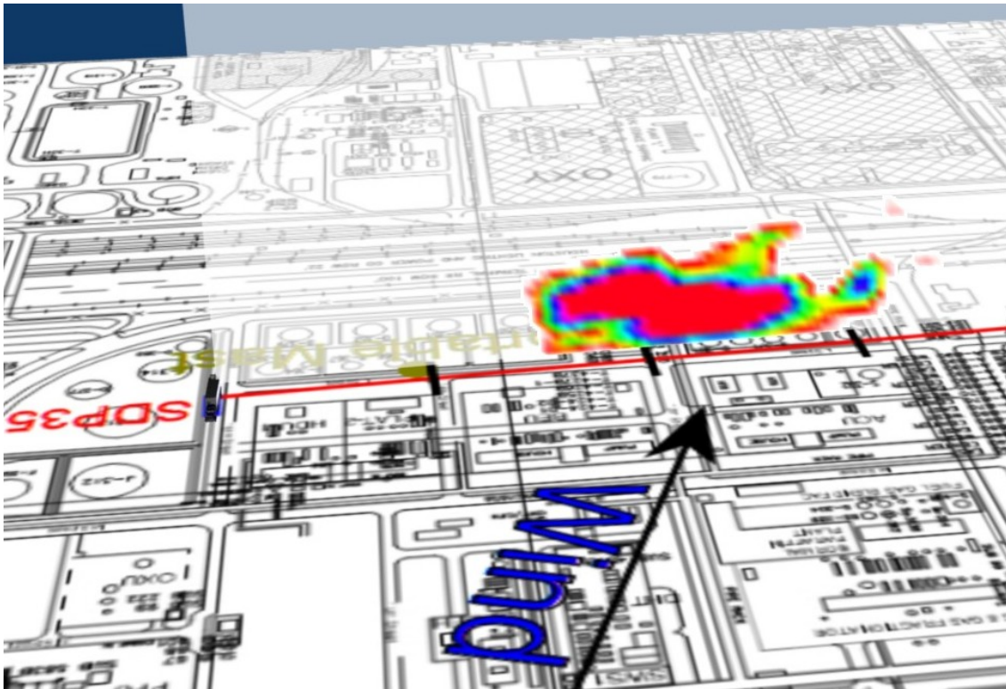
Figure 2.25a2 Visualisation of emission rate measured for Scan 824 representing LOS1.
