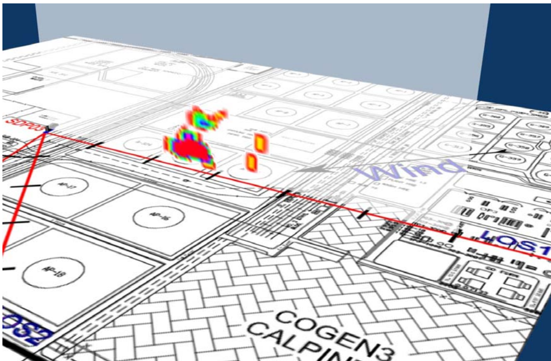
Figure 2.3a2 Visualisation of emission rate measured for Scan 65 representing LOS1.
