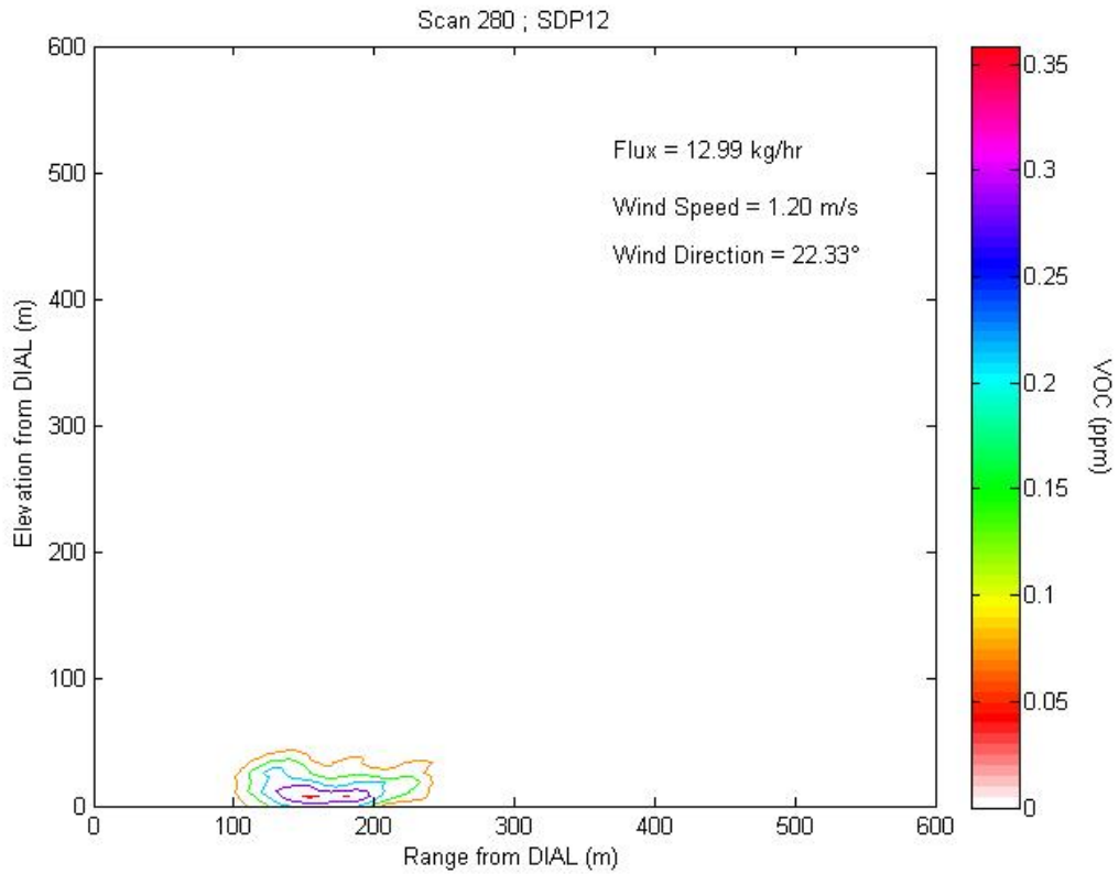
Figure 2.12a1 Contour plot of concentration profile for Scan 280 representing LOS1.
