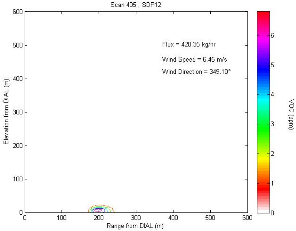
Figure 2.17b1 Contour plot of concentration profile for Scan 405 representing LOS2.
