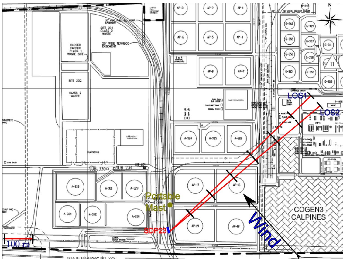
Figure 3.1 Measurement configuration for location SDP23 on 8 th of February.
