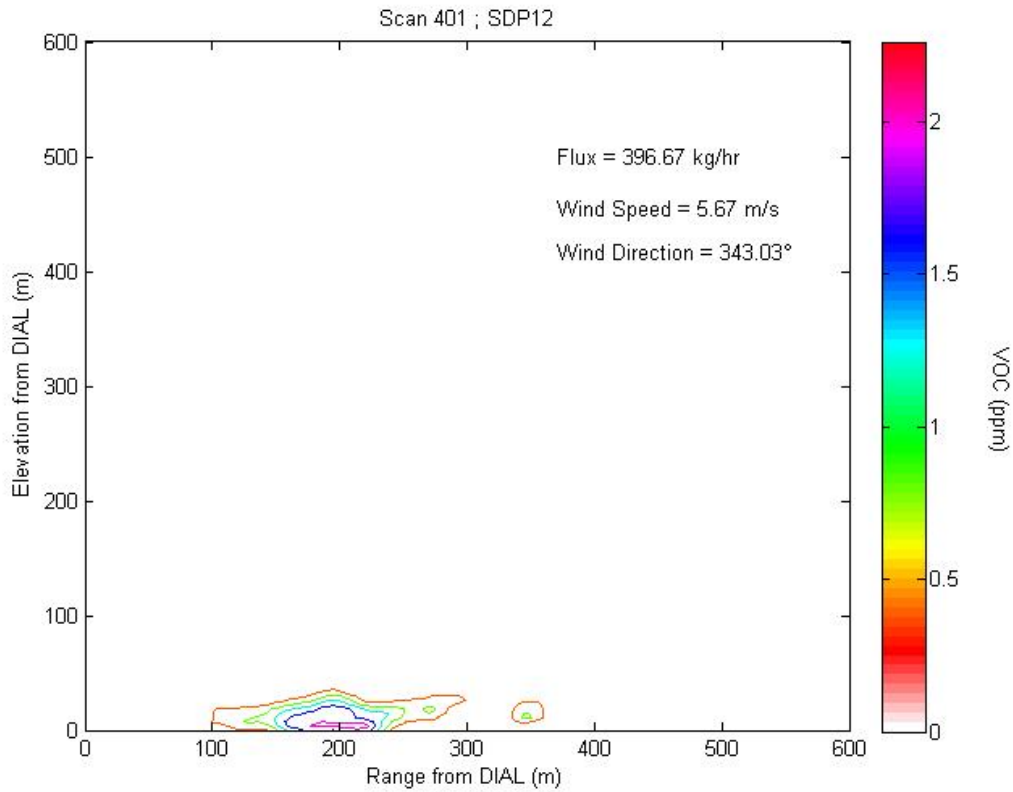
Figure 2.17a1 Contour plot of concentration profile for Scan 401 representing LOS1.
