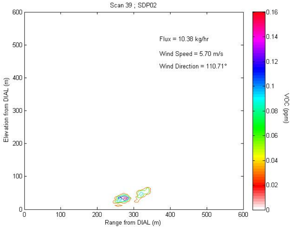
Figure 2.2a1 Contour plot of concentration profile for Scan 39 representing LOS1.
