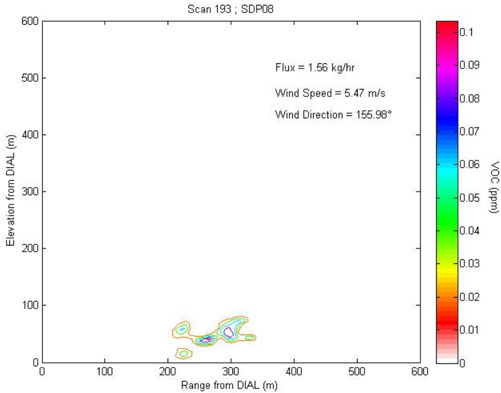
Figure 2.8b1 Contour plot of concentration profile for Scan 193 representing LOS4.
