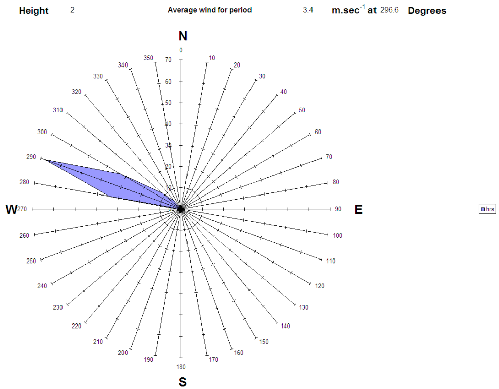
Figure A3.23 Wind rose for 5 th February during measurements from SDP21, 10:50 - 14:11
