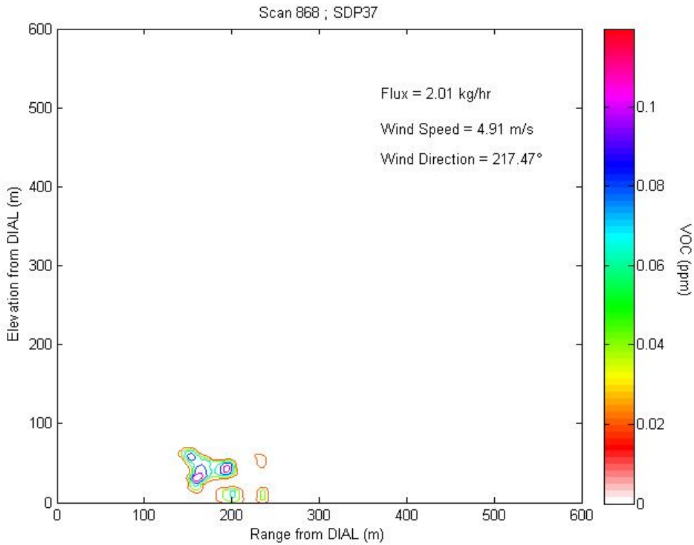
Figure 2.27b1 Contour plot of concentration profile for Scan 868 representing LOS3.
