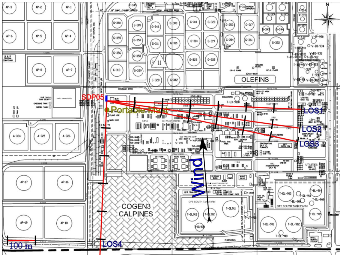
Figure 2.5 Measurement configuration for location SDP05 on 18 th of January.
