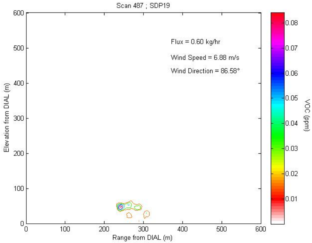
Figure 2.20a1 Contour plot of concentration profile for Scan 487 representing LOS1.
