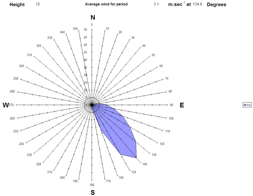
Figure A3.14 Wind rose for 26 th January during measurements from SDP13, 12:43 - 16:47
