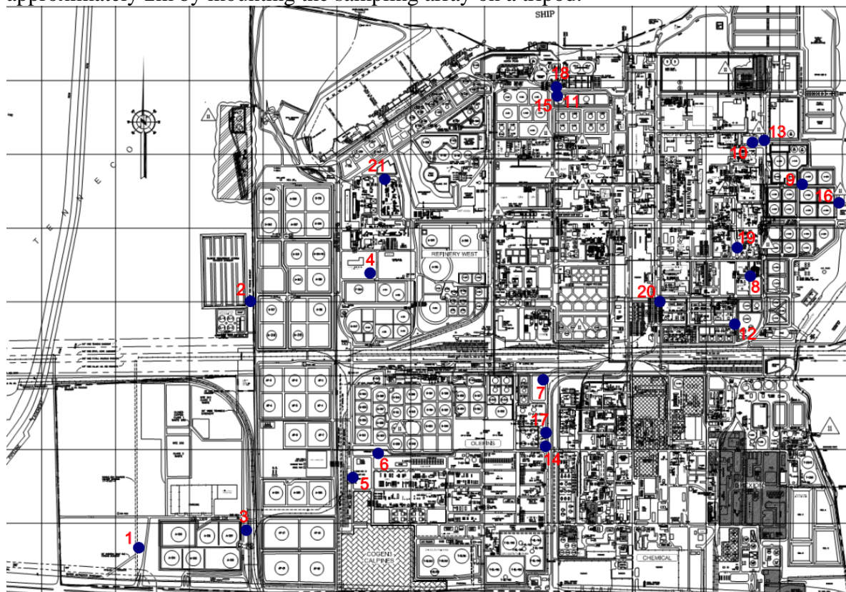
Figure A2.1 Pumped sample tube locations
