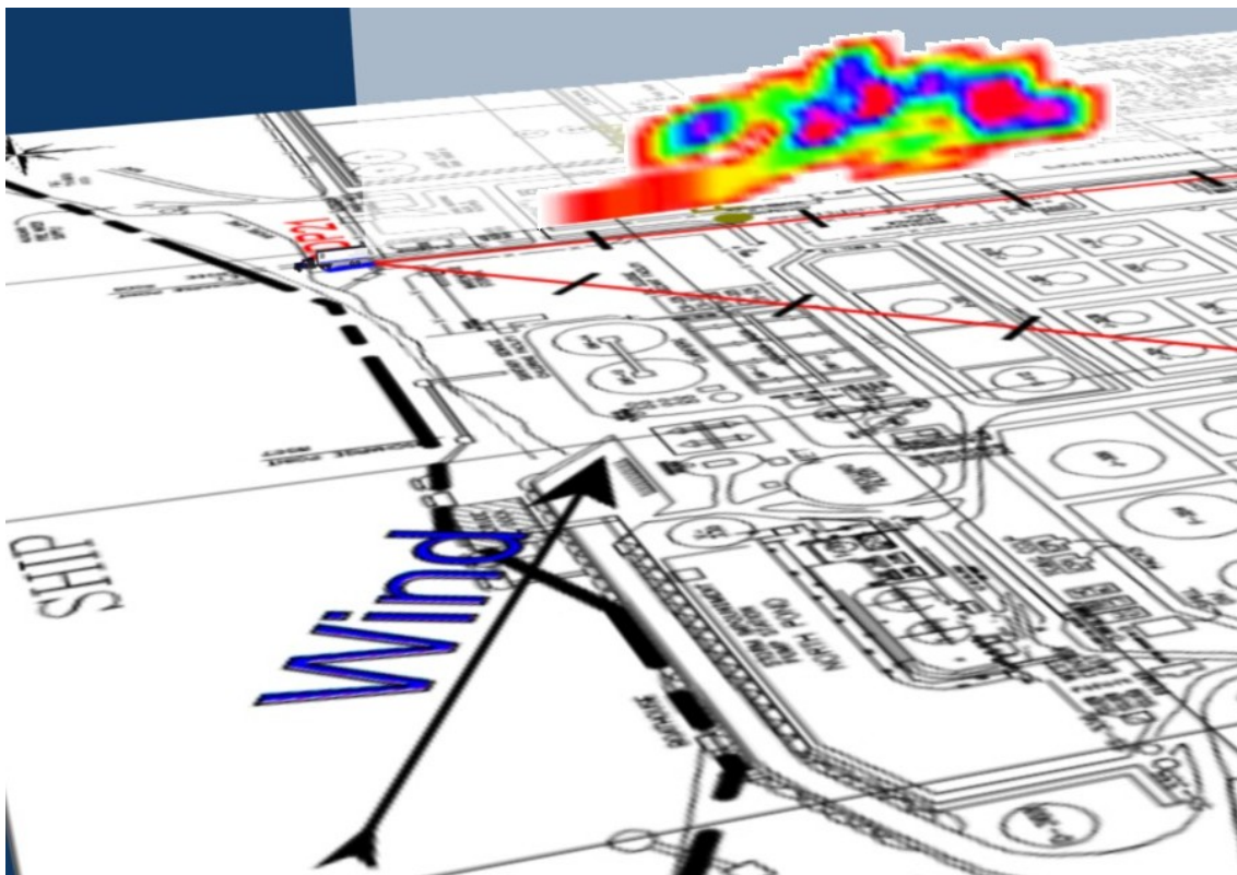
Figure 2.22b2 Visualisation of emission rate measured for Scan 532 representing LOS2.
