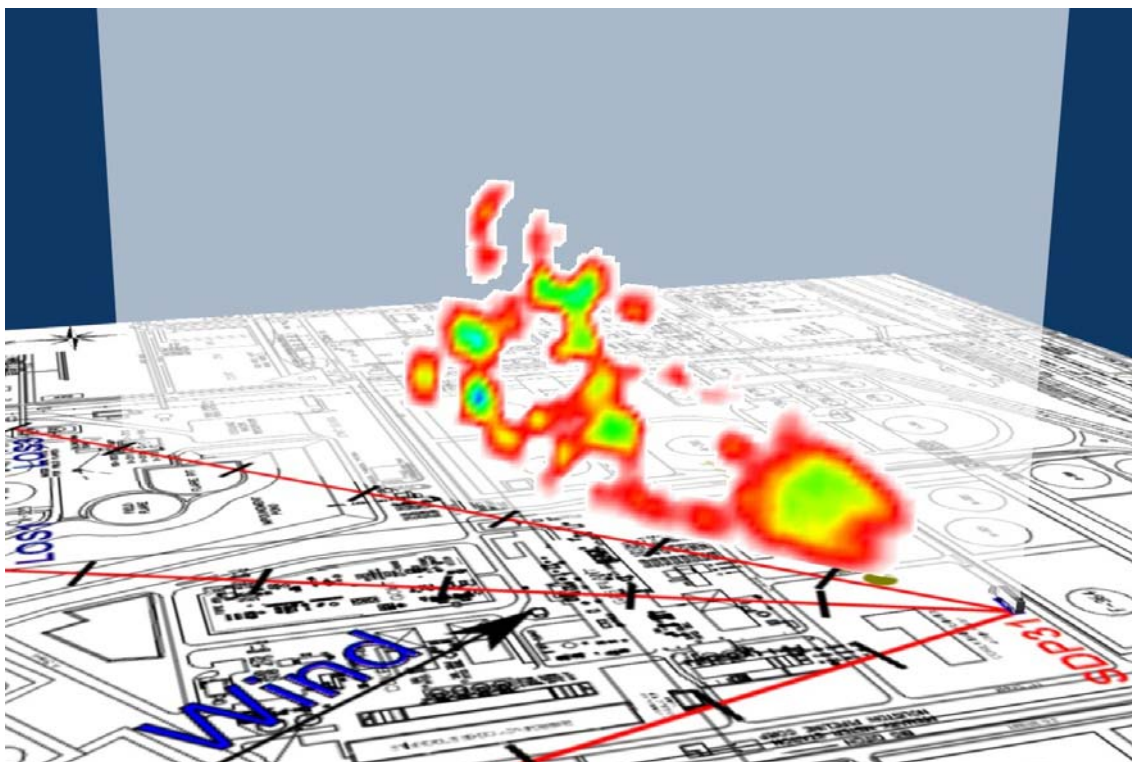
Figure 3.10a2 Visualisation of emission rate measured for Scan 745 representing LOS3.
