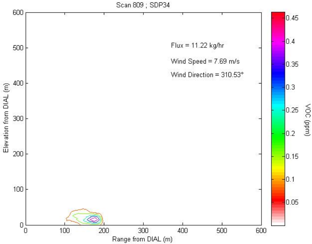
Figure 2.24a1 Contour plot of concentration profile for Scan 809 representing LOS1.
