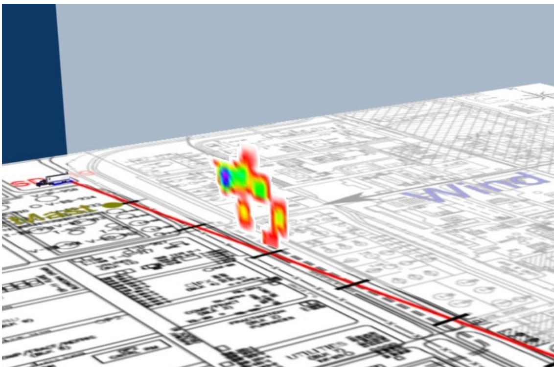
Figure 2.20a2 Visualisation of emission rate measured for Scan 487 representing LOS1.
