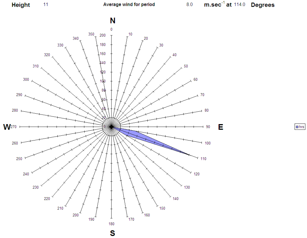
Figure A3.16 Wind rose for 28 th January during measurements from SDP15, 11:23 - 16:41
