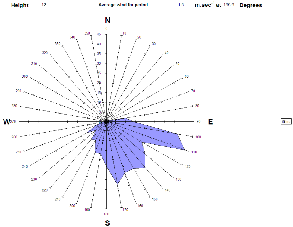
Figure A3.28 Wind rose for 10 th February during measurements from SDP26, 9:55 - 17:05
