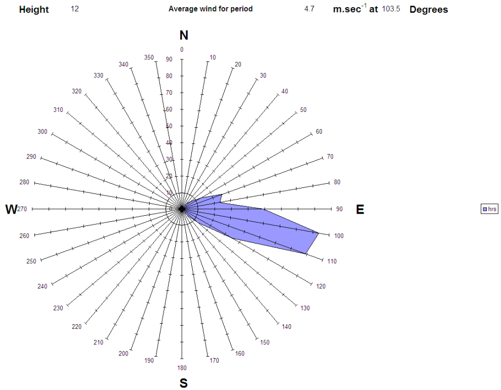
Figure A3.21 Wind rose for 3 rd February during measurements from SDP19, 10:30 - 16:54
