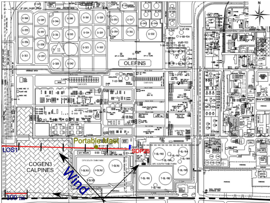
Figure 3.4 Measurement configuration for location SDP26 on 10 th of February.
