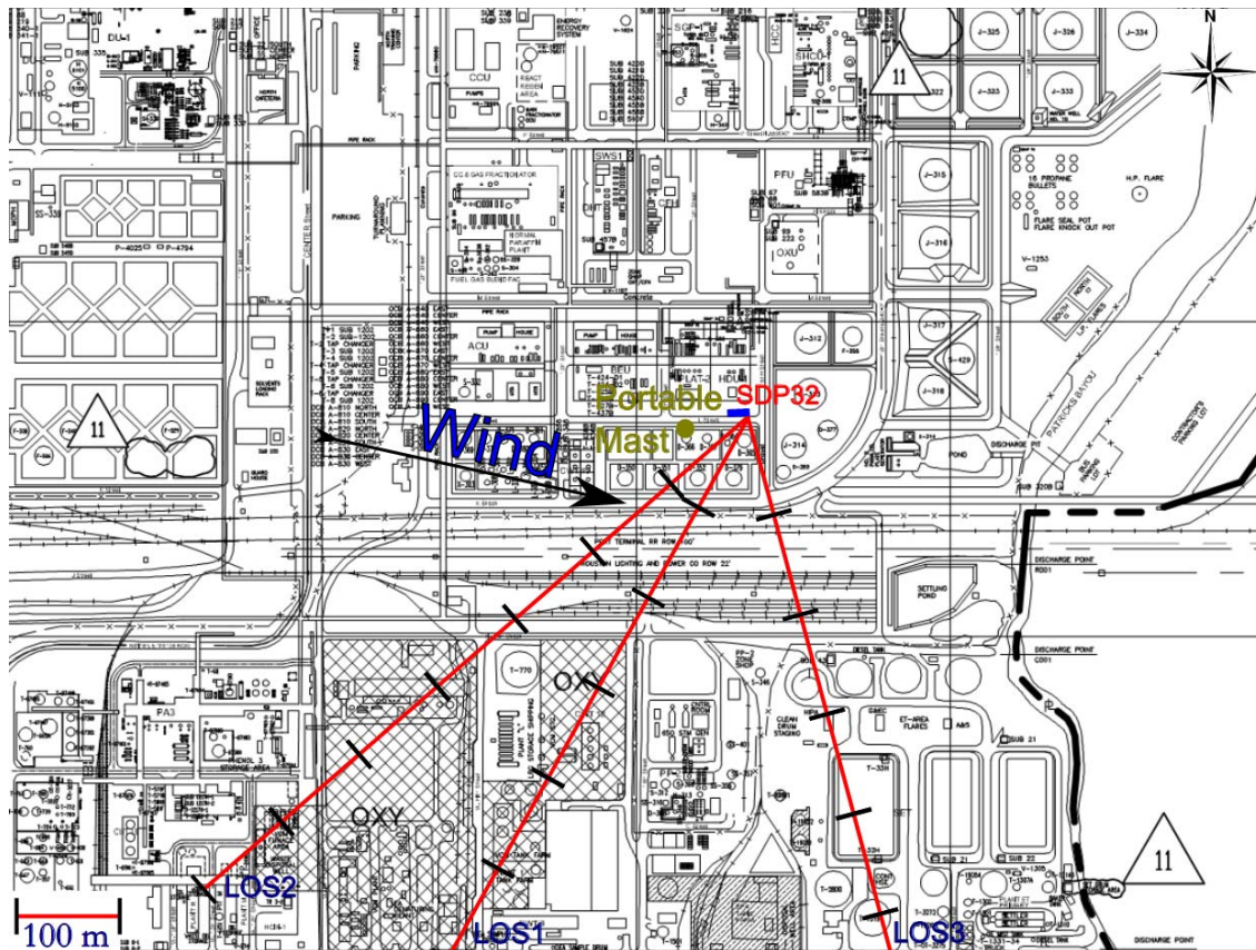
Figure 3.11 Measurement configuration for location SDP32 on 22 nd of March.
