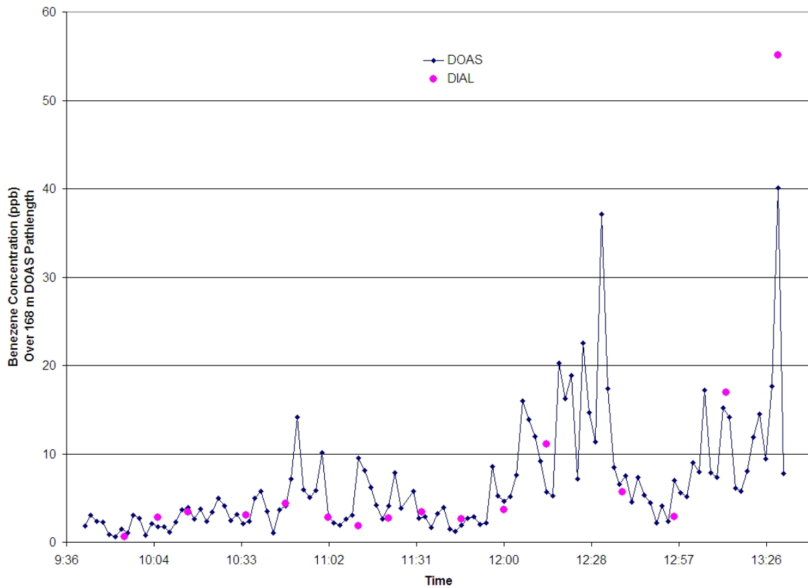
Figure 5.2 DIAL and DOAS measurements comparison on the 10 th of February until 13:30.
