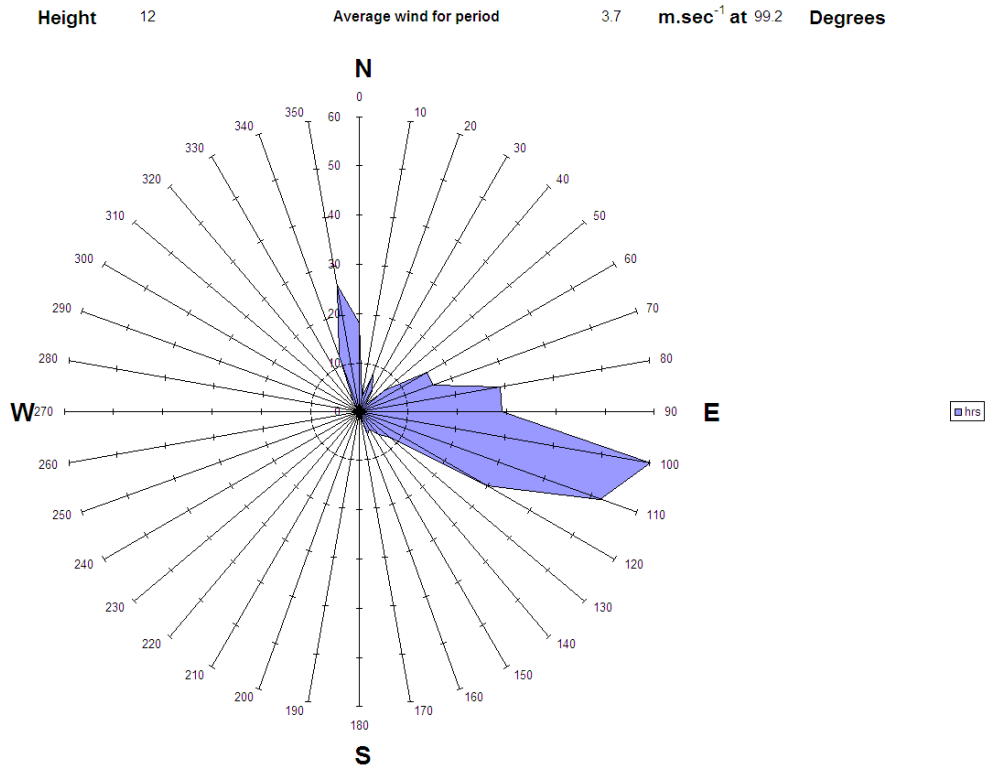
Figure A3.22 Wind rose for 4 th February during measurements from SDP20, 10:17 - 16:50
