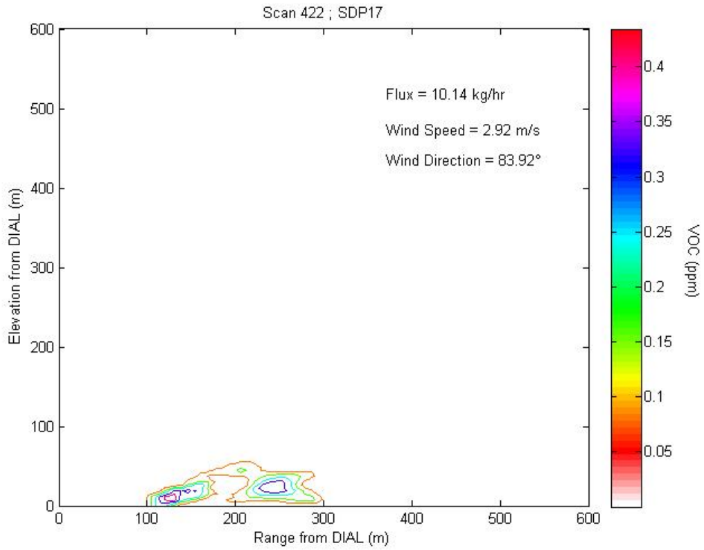
Figure 2.18a1 Contour plot of concentration profile for Scan 422 representing LOS1.
