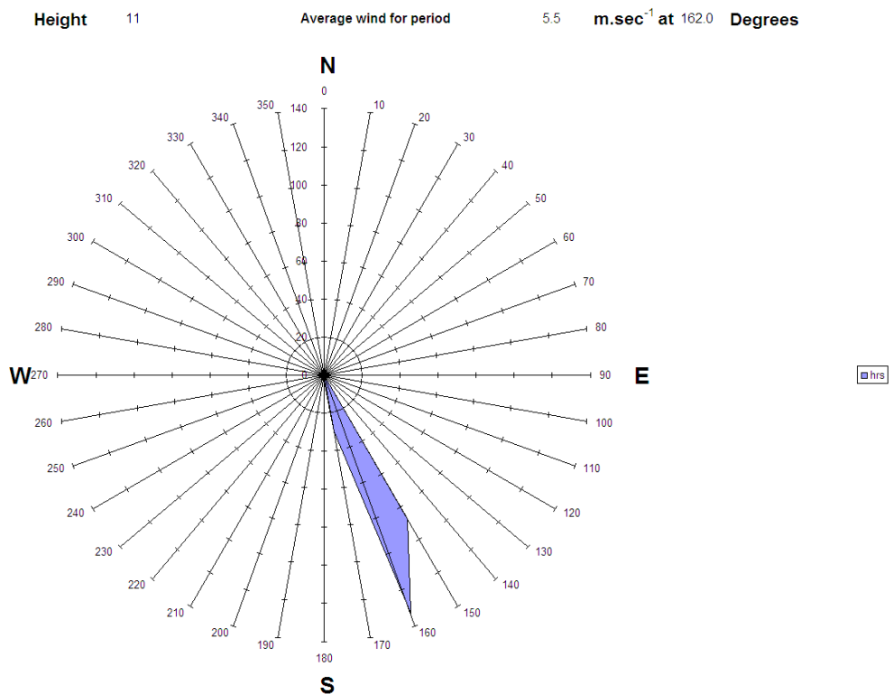
Figure A3.9 Wind rose for 20 th January during measurements from SDP8, 11:57 - 17:06
