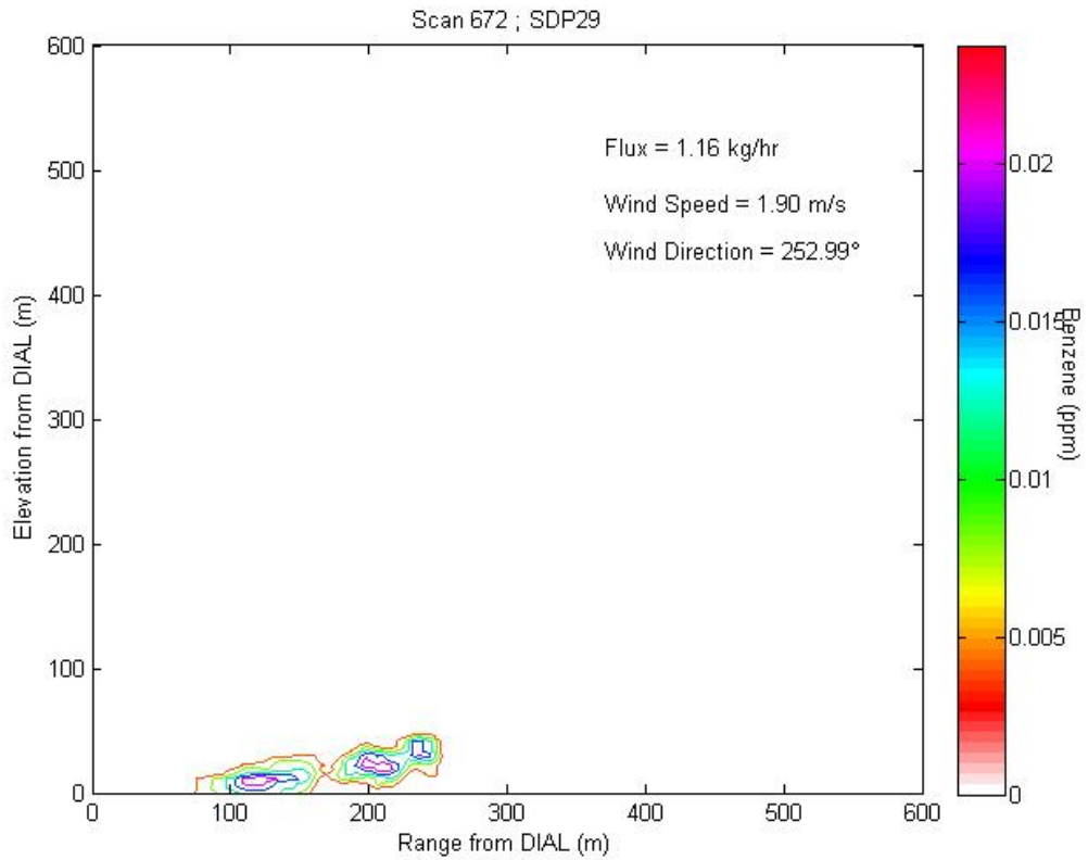
Figure 3.7b1 Contour plot of concentration profile for Scan 672 representing LOS3.
