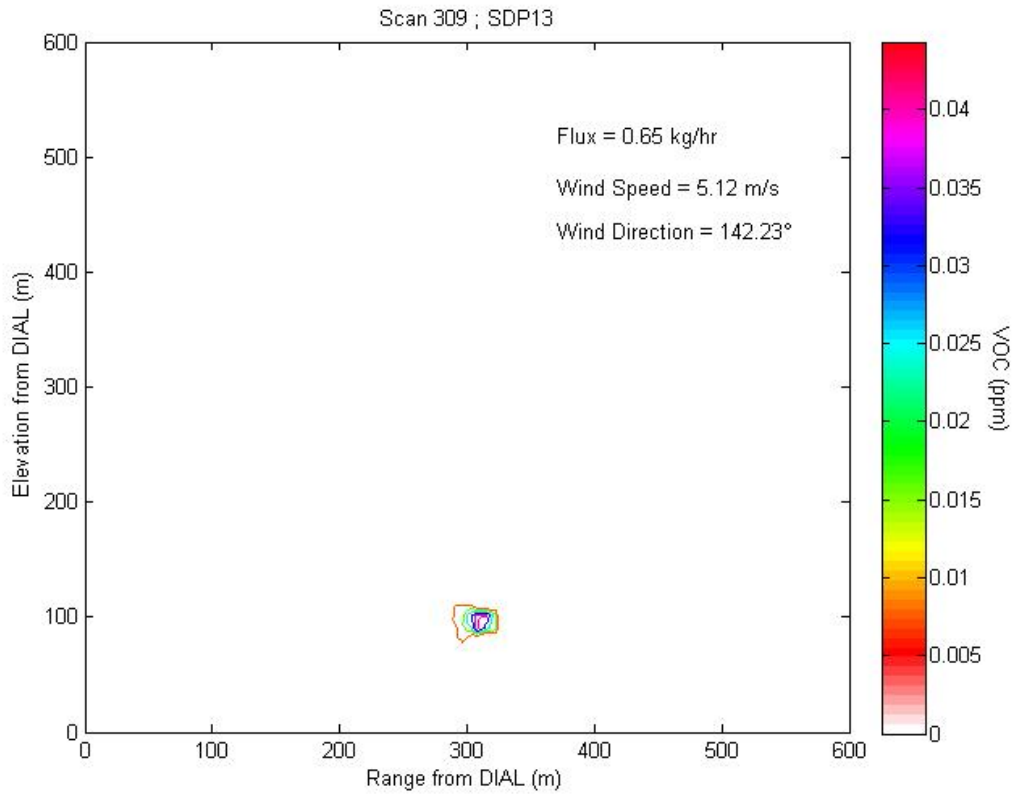
Figure 2.13a1 Contour plot of concentration profile for Scan 309 representing LOS2.
