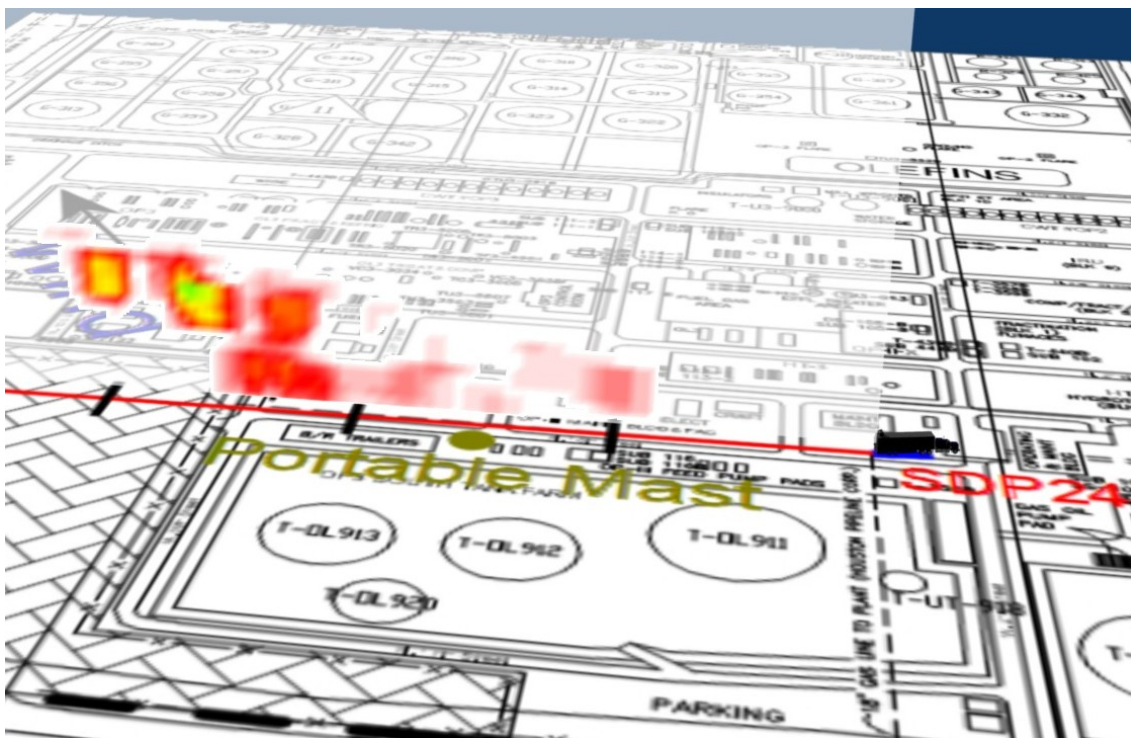
Figure 3.2a2 Visualisation of emission rate measured for Scan 555 representing LOS1.
