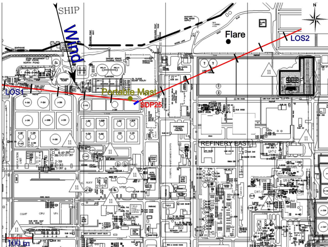
Figure 3.3 Measurement configuration for location SDP25 on 9 th of February.
