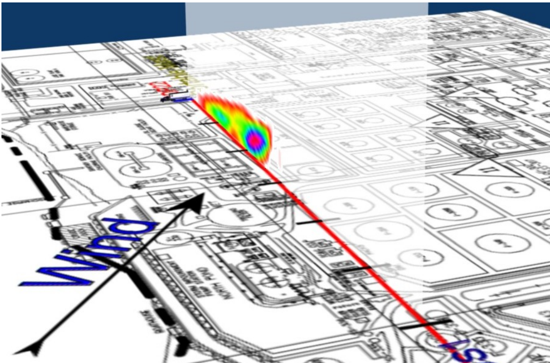
Figure 2.23a2 Visualisation of emission rate measured for Scan 537 representing LOS1.
