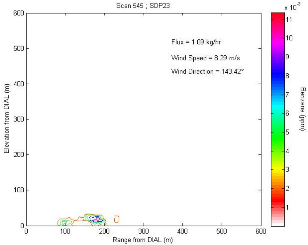
Figure 3.1a1 Contour plot of concentration profile for Scan 545 representing LOS1.
