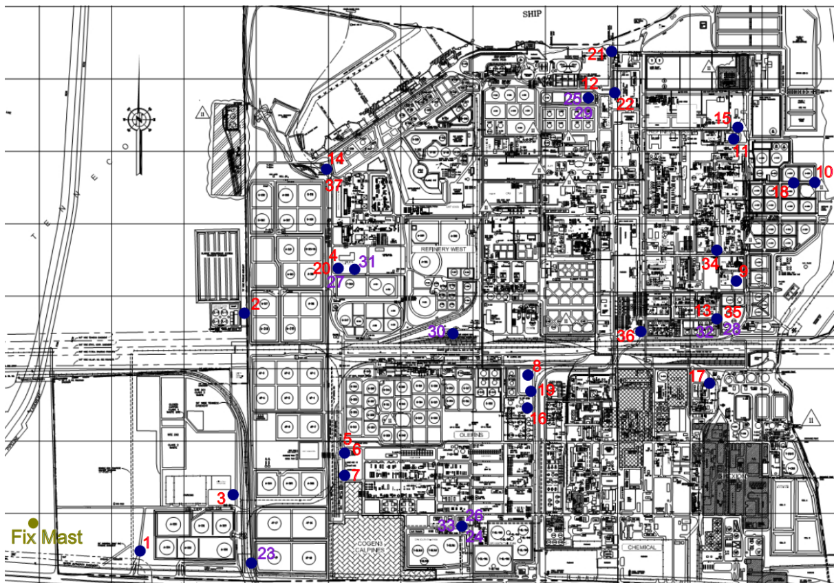
Figure 1.2 DIAL measurement locations and location of fixed meteorological mast. The blue dots represent the DIAL measurement locations and the red and purple numeric labels for each dot indicate the type of measurement (red for VOC and purple for benzene).
