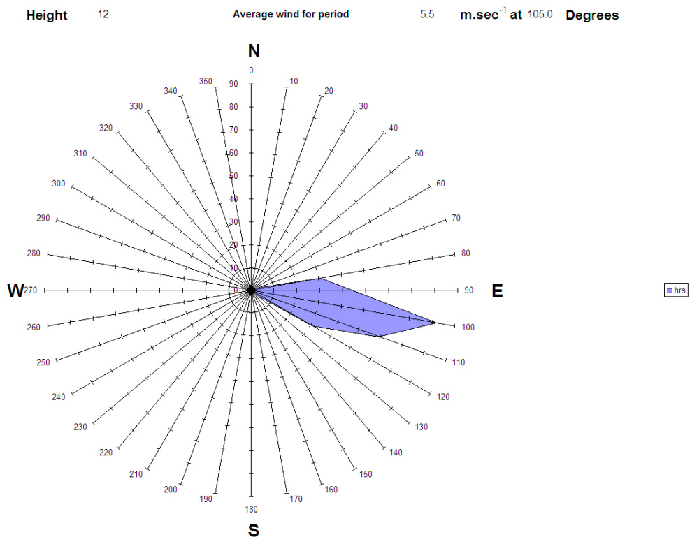
Figure A3.3 Wind rose for 14 th January during measurements from SDP2, 12:32 - 17:04
