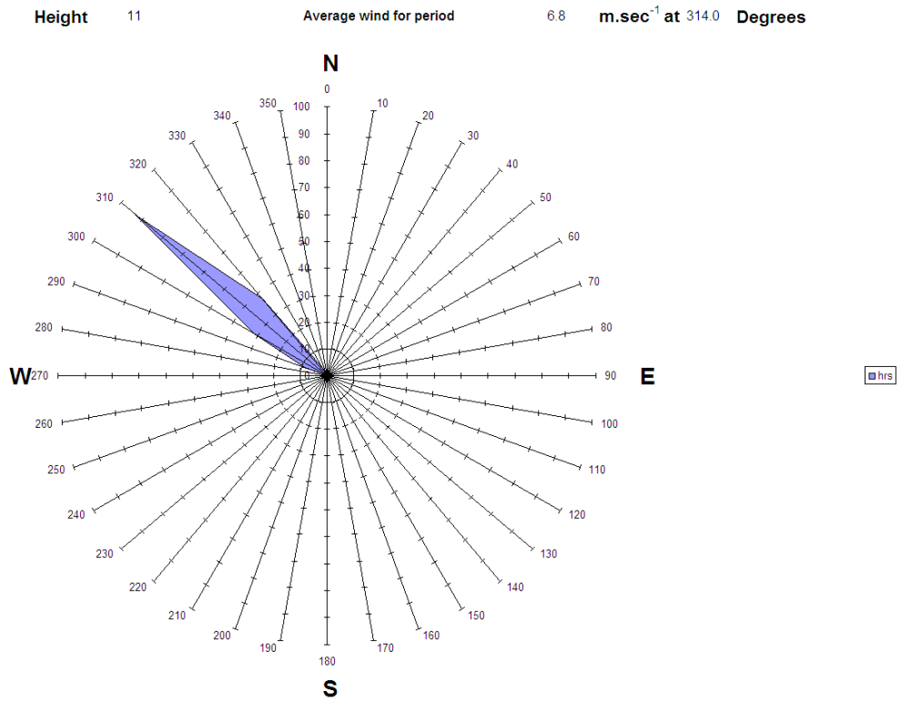
Figure A3.17 Wind rose for 29 th January during measurements from SDP16, 14:01 - 16:56
