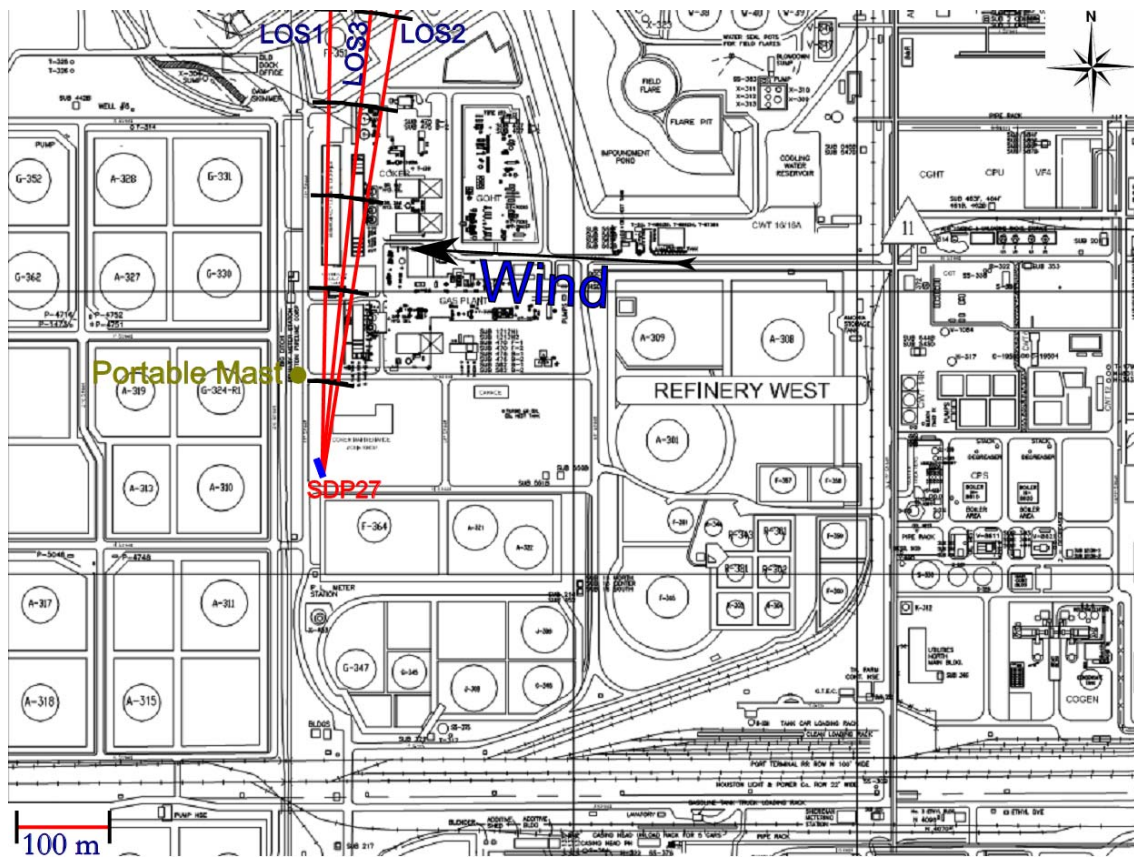
Figure 3.5 Measurement configuration for location SDP27 on 11 th of February.
