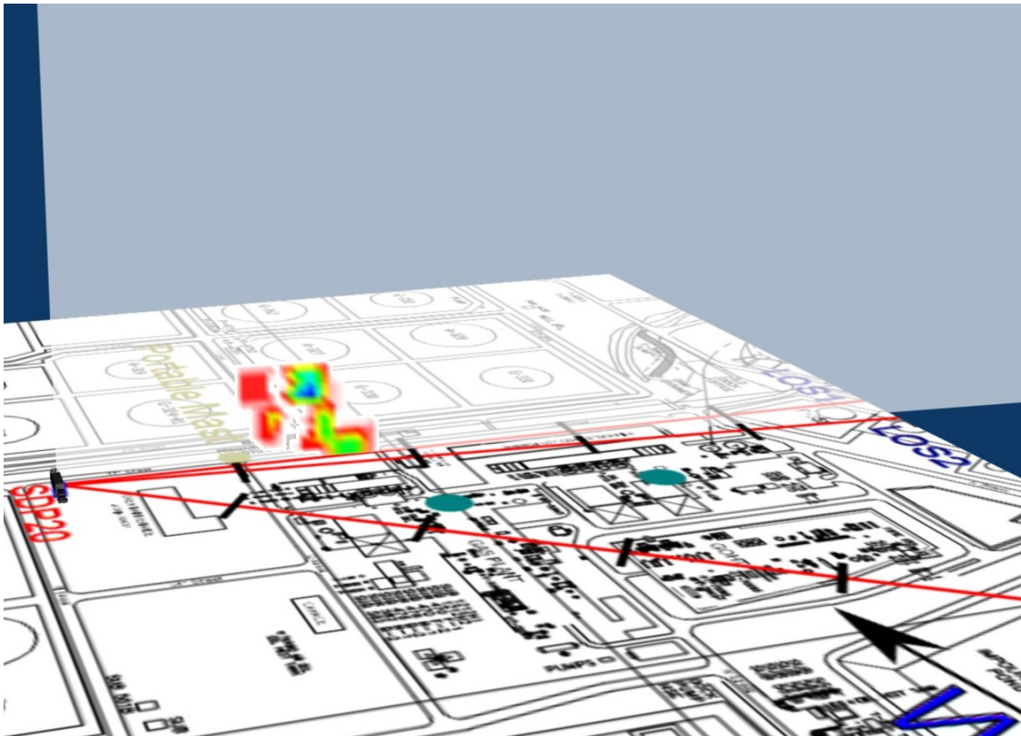
Figure 2.21a2 Visualisation of emission rate measured for Scan 513 representing LOS2.
