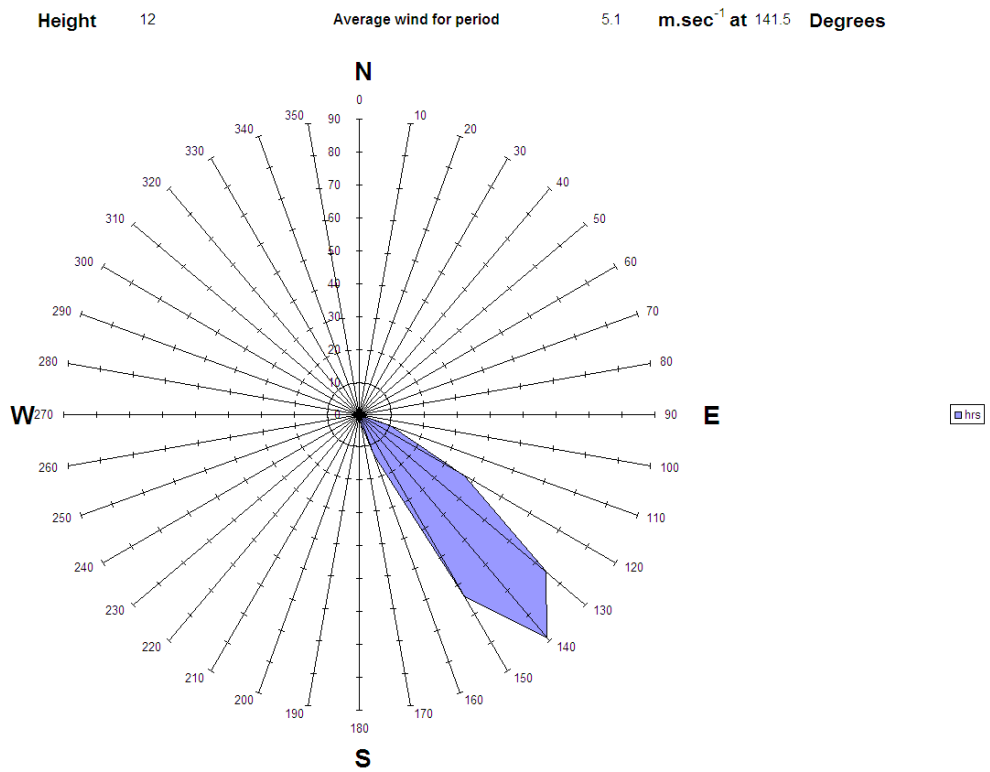
Figure A3.11 Wind rose for 22 nd January during measurements from SDP10, 12:07 - 17:30
