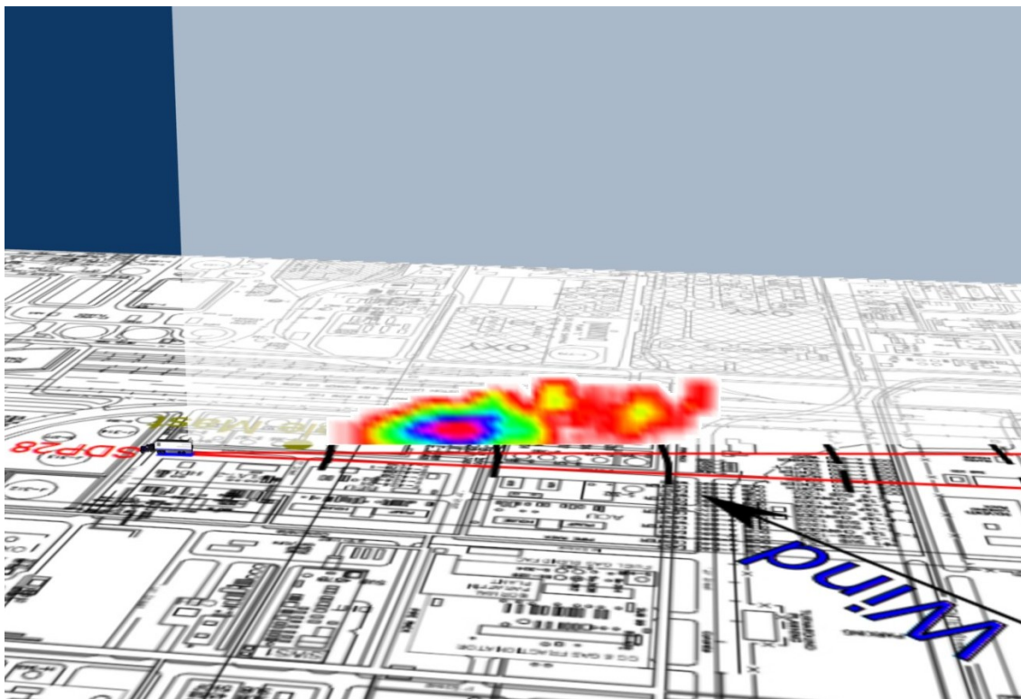
Figure 3.6b2 Visualisation of emission rate measured for Scan 658 representing LOS2.
