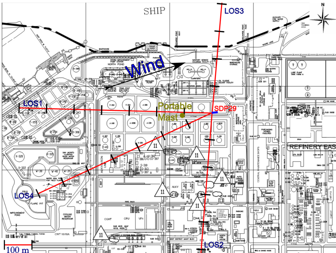
Figure 3.7 Measurement configuration for location SDP29 on 13 th of February.
