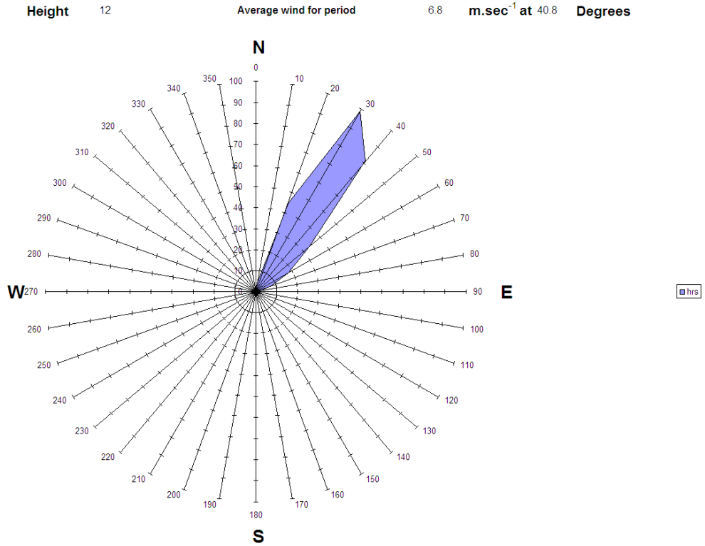
Figure A3.4 Wind rose for 15 th January during measurements from SDP3, 11:35 - 16:50
