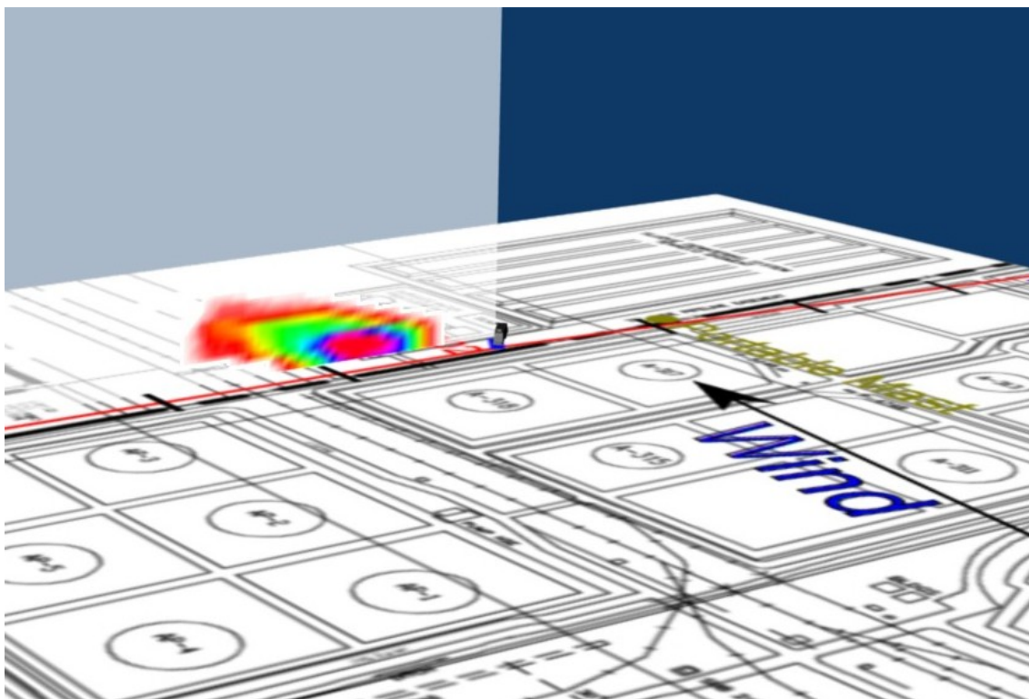
Figure 2.2c2 Visualisation of emission rate measured for Scan 52 representing LOS2.
