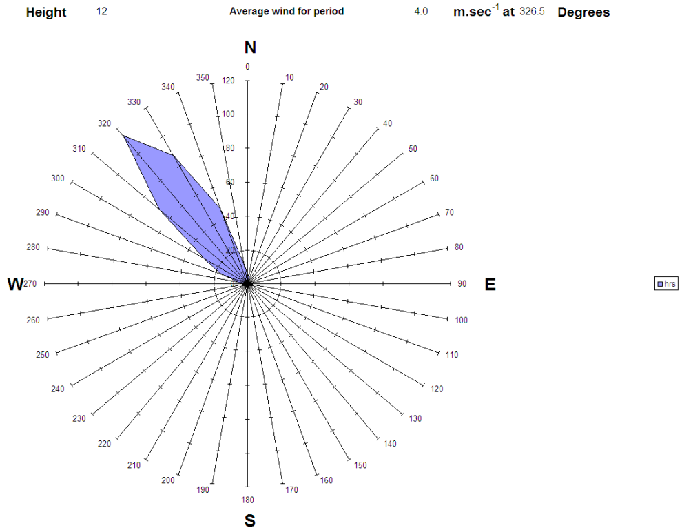
Figure A3.34 Wind rose for 17 th February during measurements from SDP31, 10:06 - 16:54
