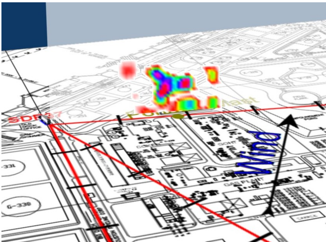
Figure 2.27b2 Visualisation of emission rate measured for Scan 868 representing LOS3.
