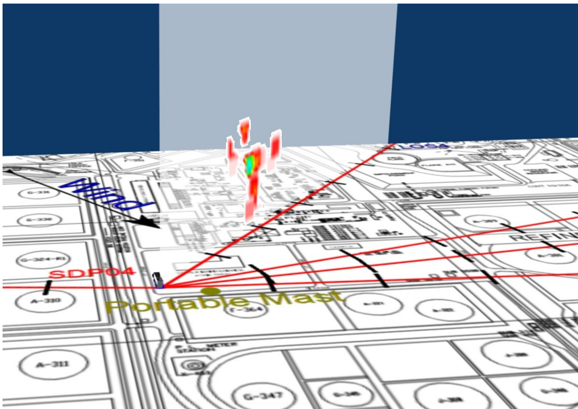
Figure 2.4b2 Visualisation of emission rate measured for Scan 108 representing LOS4.
