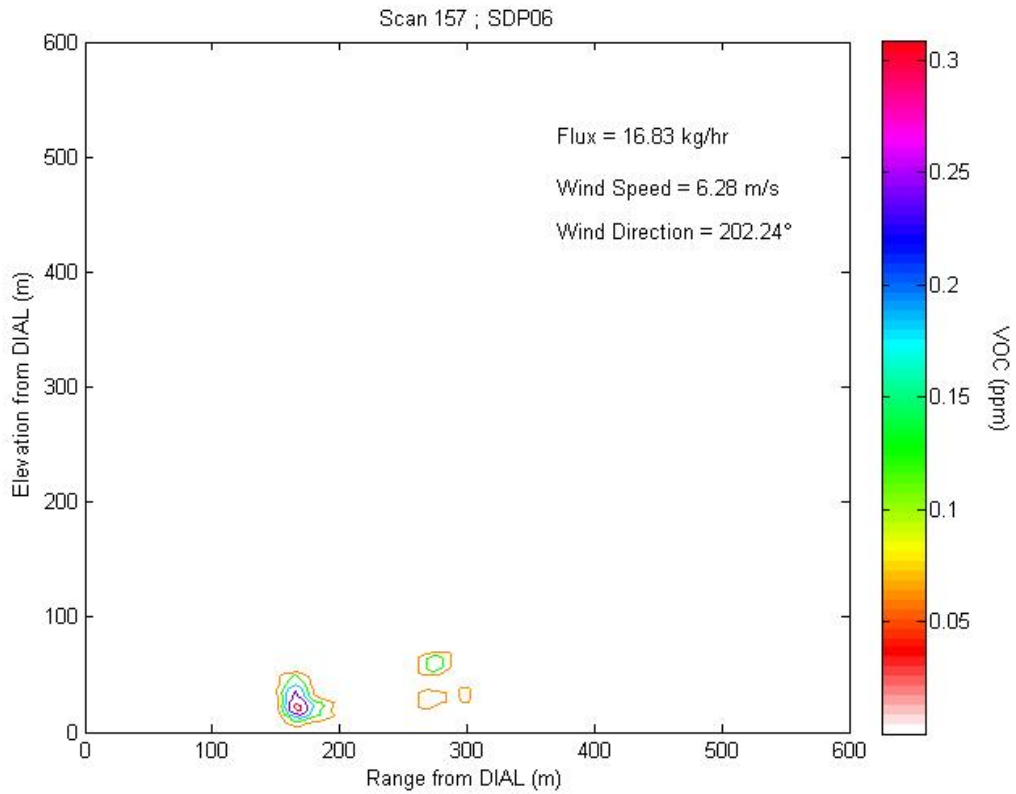
Figure 2.6b1 Contour plot of concentration profile for Scan 157 representing LOS3.
