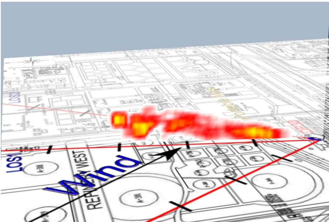
Figure 3.9a2 Visualisation of emission rate measured for Scan 714 representing LOS1.
