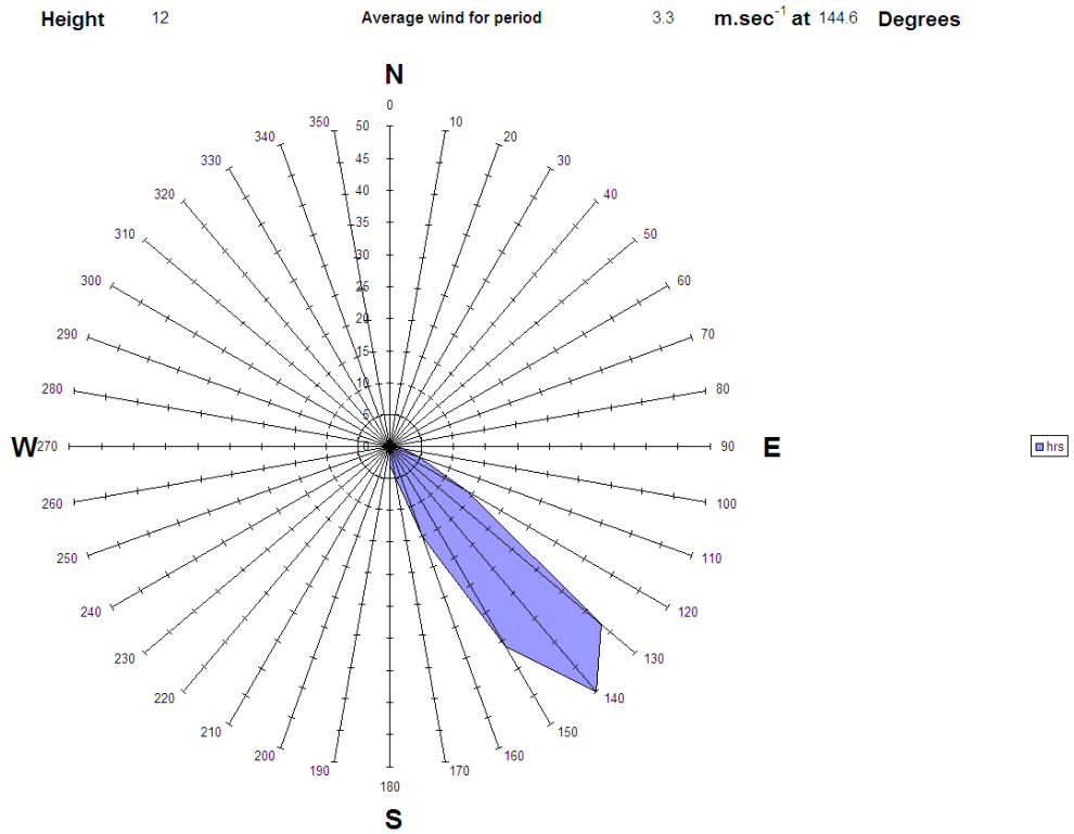
Figure A3.26 Wind rose for 8 th February during measurements from SDP24, 14:15 - 17:23
