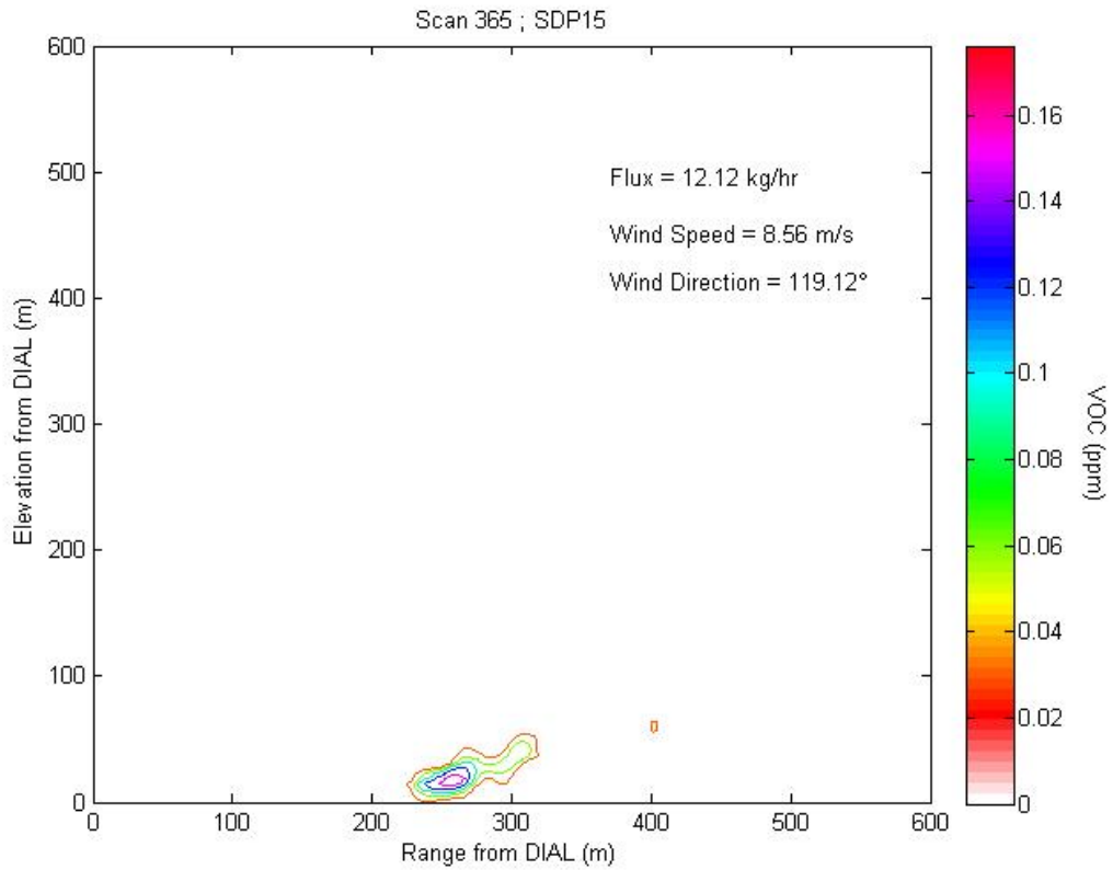
Figure 2.15a1 Contour plot of concentration profile for Scan 365 representing LOS2.
