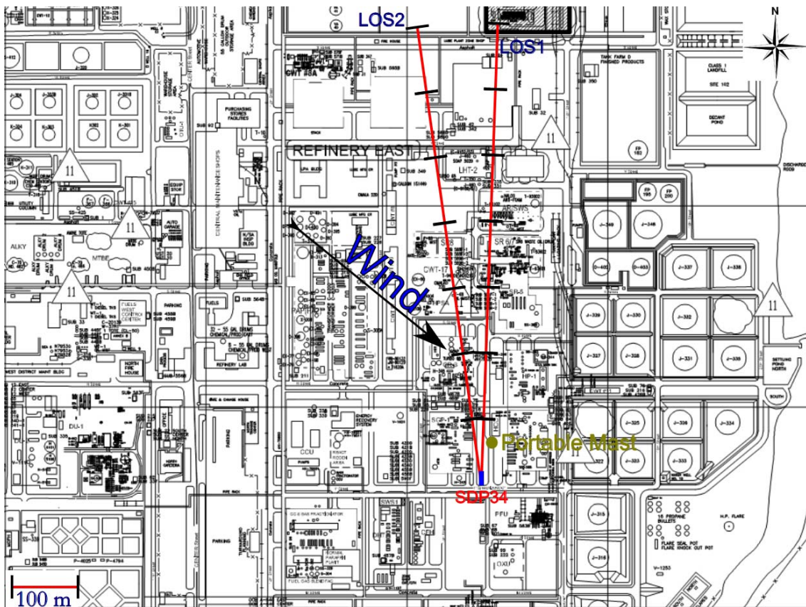
Figure 2.24 Measurement configuration for location SDP34 on 25 th of March.
