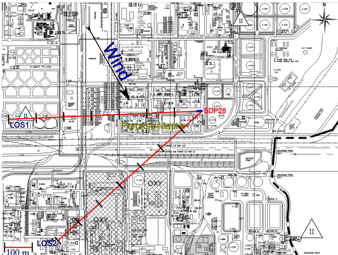
Figure 3.6 Measurement configuration for location SDP28 on 12 th of February.
