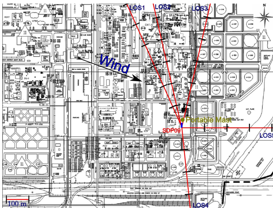
Figure 2.9 Measurement configuration for location SDP09 on 21 st of January.
