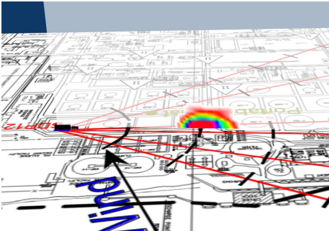
Figure 2.17b2 Visualisation of emission rate measured for Scan 405 representing LOS2.
