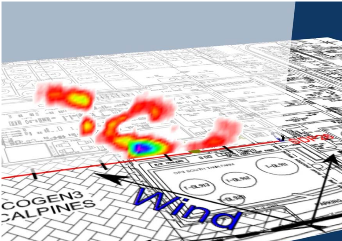
Figure 3.4a2 Visualisation of emission rate measured for Scan 614 representing LOS1.
