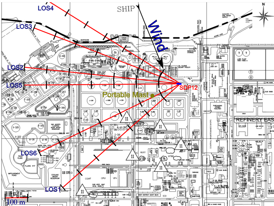
Figure 2.17 Measurement configuration for location SDP12 on 30 th of January.
