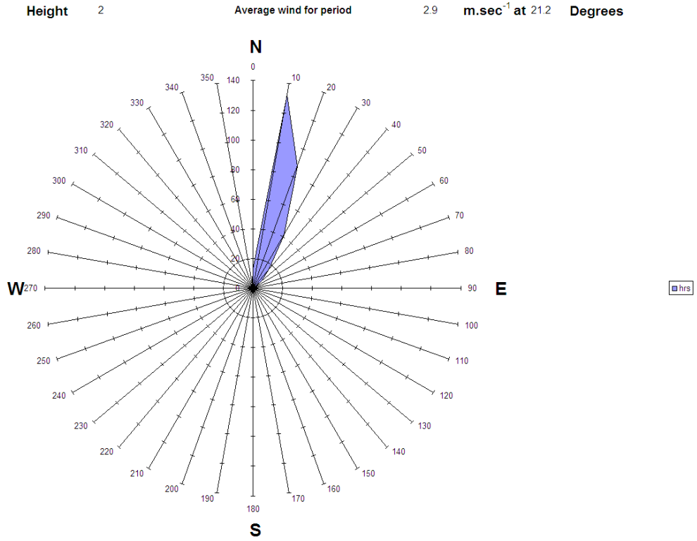
Figure A3.20 Wind rose for 2 nd February during measurements from SDP18, 10:54 - 17:05
