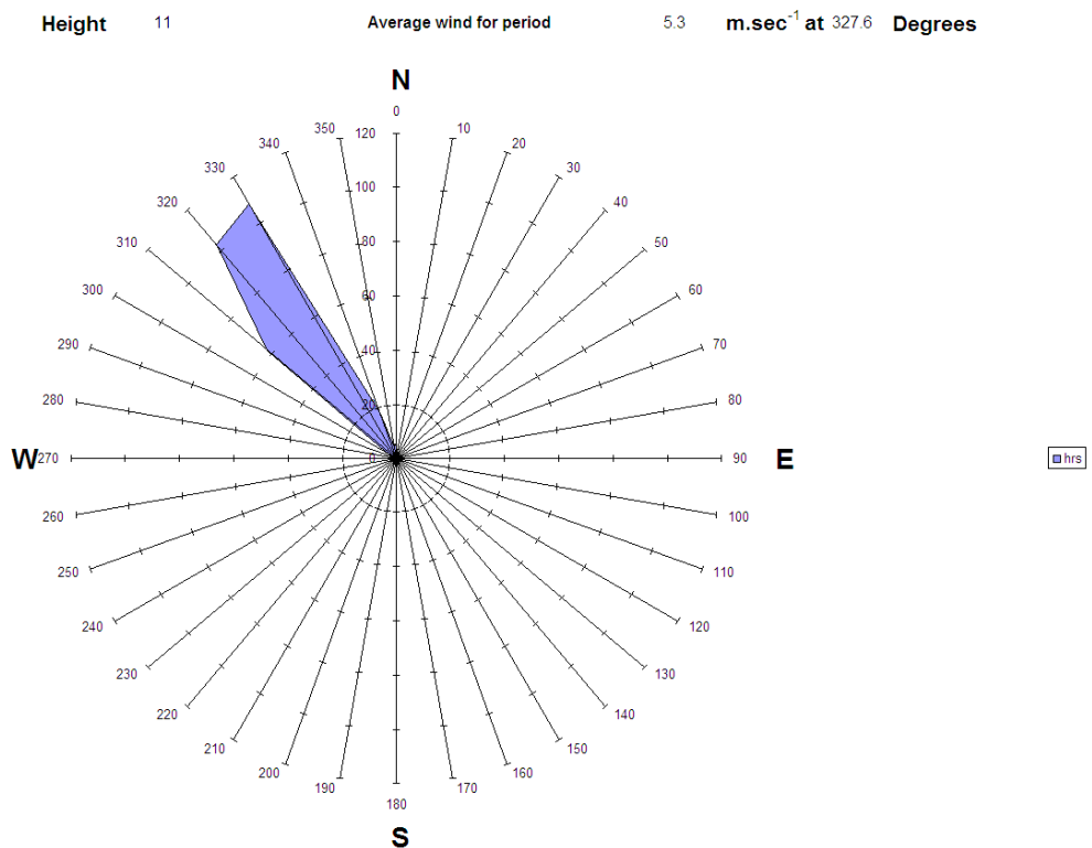
Figure A3.5 Wind rose for 16 th January during measurements from SDP4, 10:58 - 17:13
