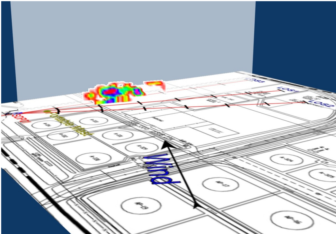
Figure 2.1a2 Visualisation of emission rate measured for Scan 12 representing LOS1.
