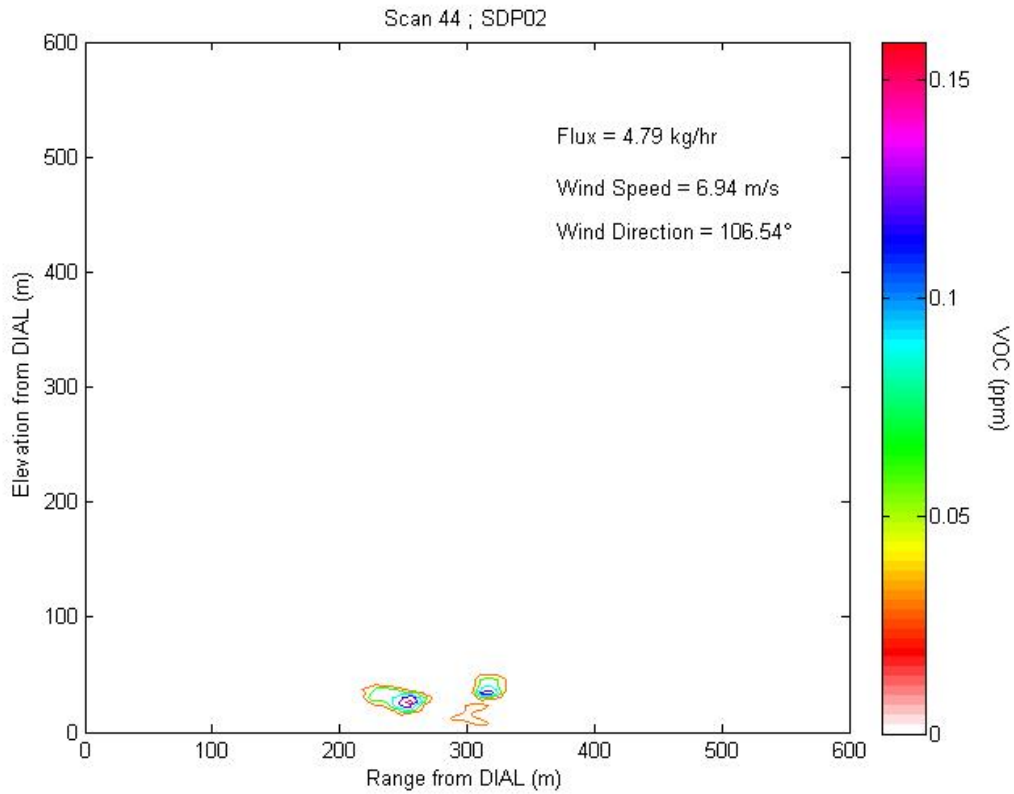
Figure 2.2b1 Contour plot of concentration profile for Scan 44 representing LOS2.
