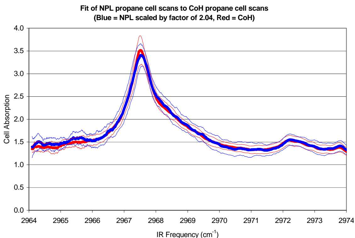
Figure 4.1 NPL reference standard absorption scaled by a factor of 2.04 (blue line) compared with the absorption from an unknown propane mixture (red line).
