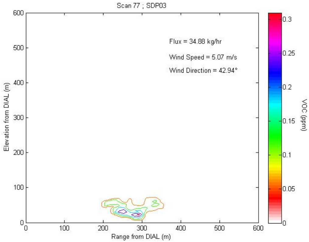
Figure 2.3c1 Contour plot of concentration profile for Scan 77 representing LOS3.
