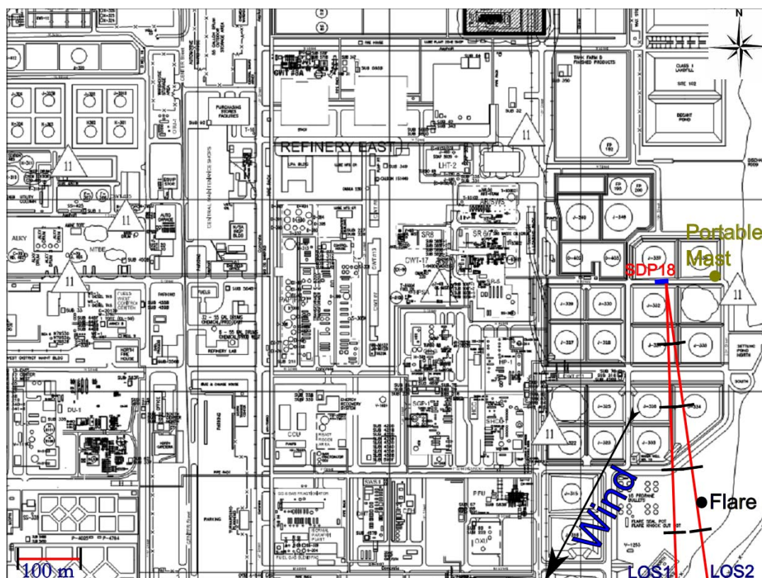
Figure 2.19 Measurement configuration for location SDP18 on 2 nd of February.
