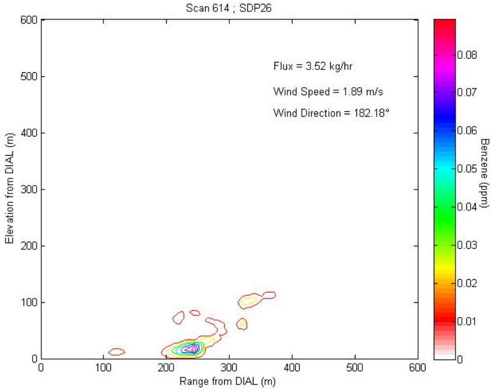
Figure 3.4a1 Contour plot of concentration profile for Scan 614 representing LOS1.
