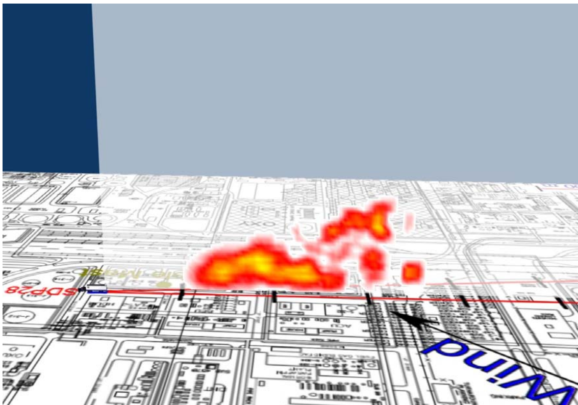
Figure 3.6a2 Visualisation of emission rate measured for Scan 647 representing LOS1.
