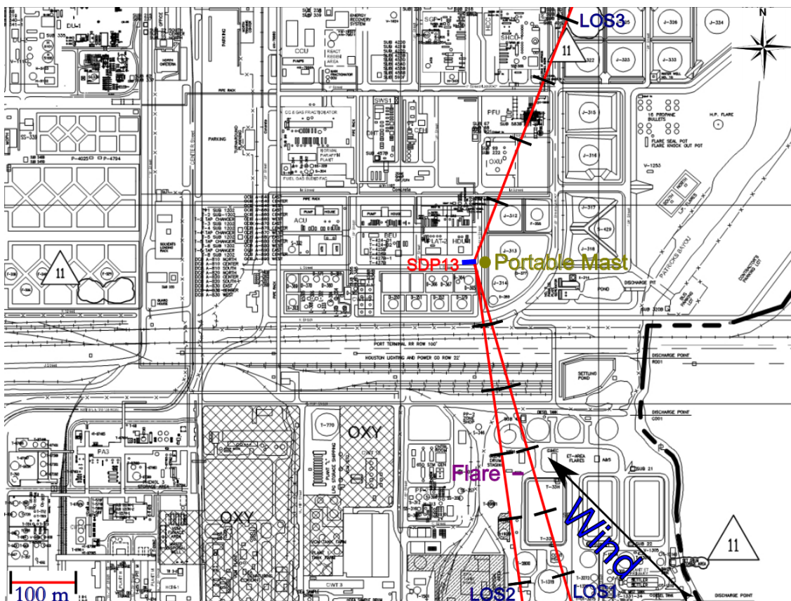
Figure 2.13 Measurement configuration for location SDP13 on 26 th of January.
