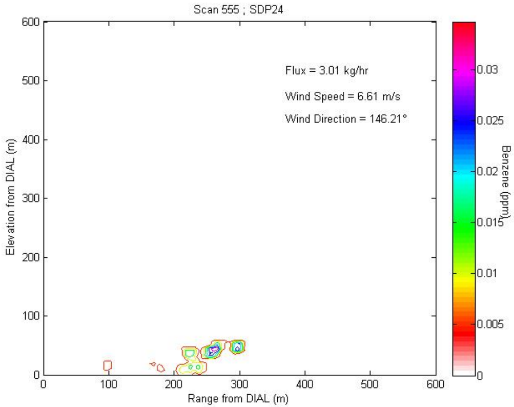
Figure 3.2a1 Contour plot of concentration profile for Scan 555 representing LOS1.
