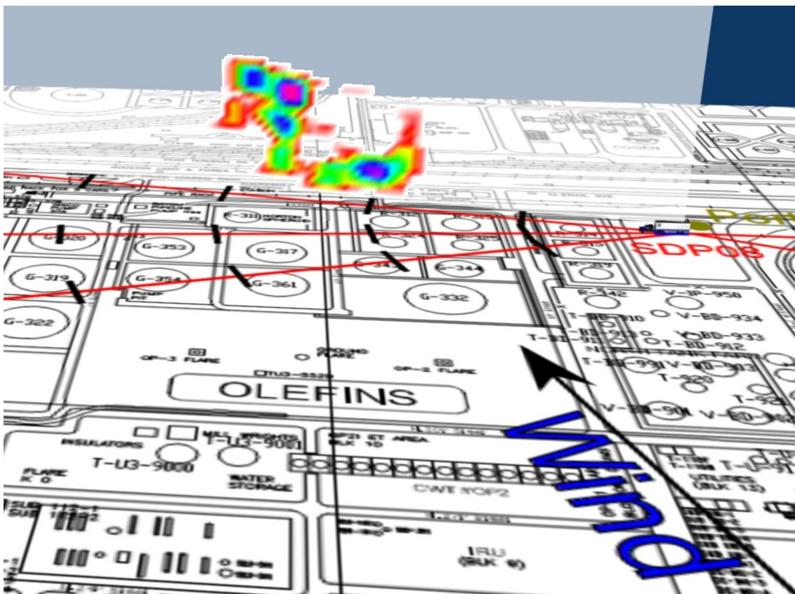
Figure 2.8a2 Visualisation of emission rate measured for Scan 176 representing LOS1.
