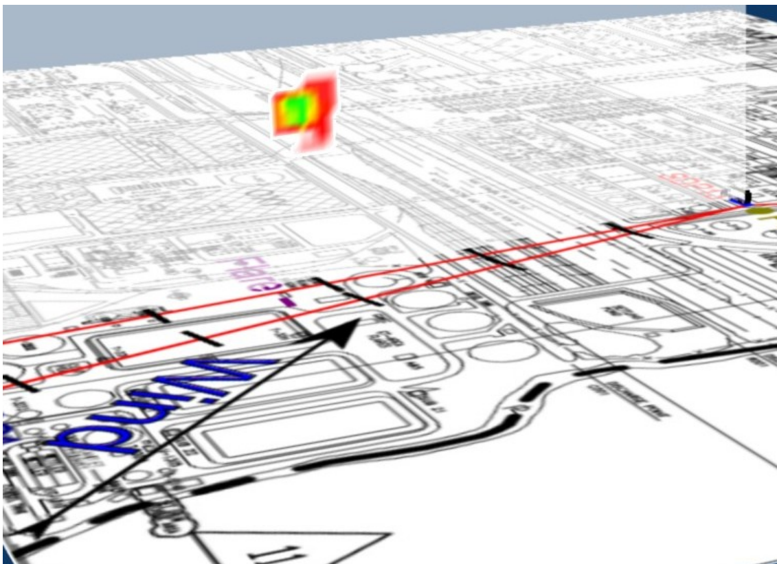
Figure 2.13a2 Visualisation of emission rate measured for Scan 309 representing LOS2.
