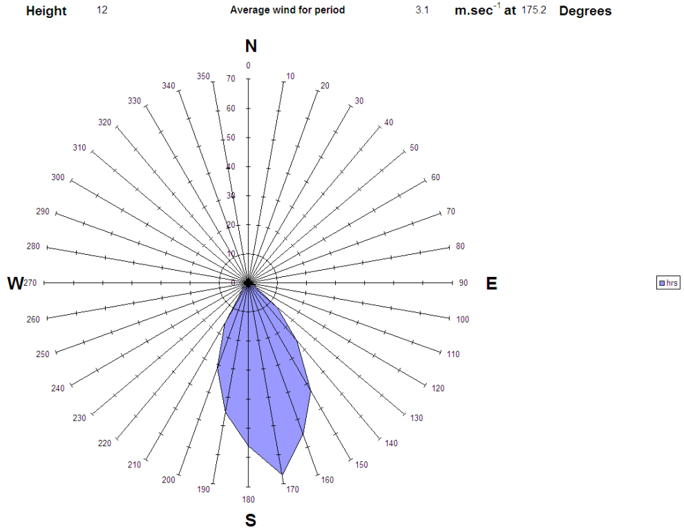
Figure A3.36 Wind rose for 23 rd March during measurements from SDP33, 10:18 - 17:05
