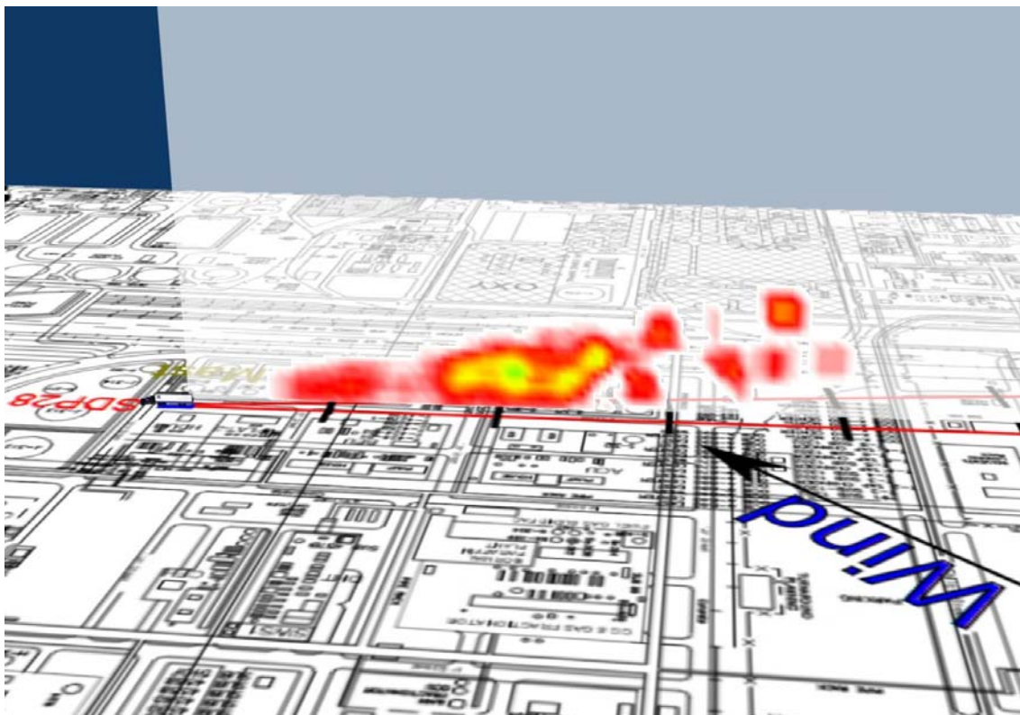
Figure 3.8a2 Visualisation of emission rate measured for Scan 693 representing LOS1.
