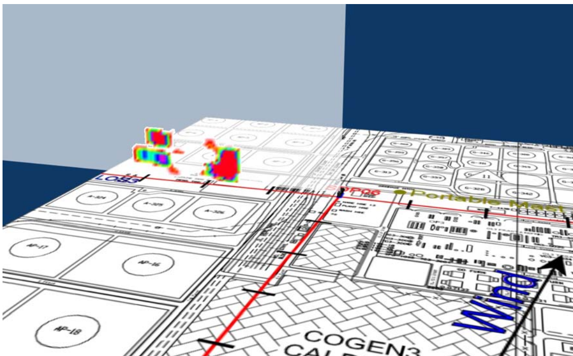
Figure 2.6b2 Visualisation of emission rate measured for Scan 157 representing LOS3.
