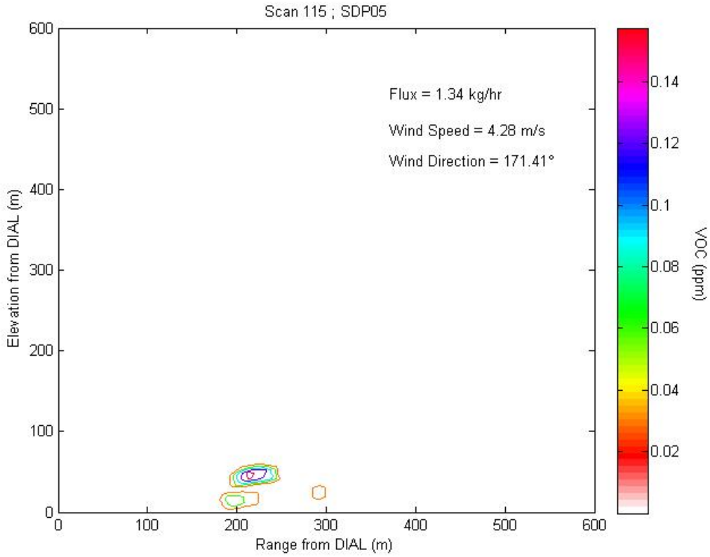
Figure 2.5a1 Contour plot of concentration profile for Scan 115 representing LOS1.
