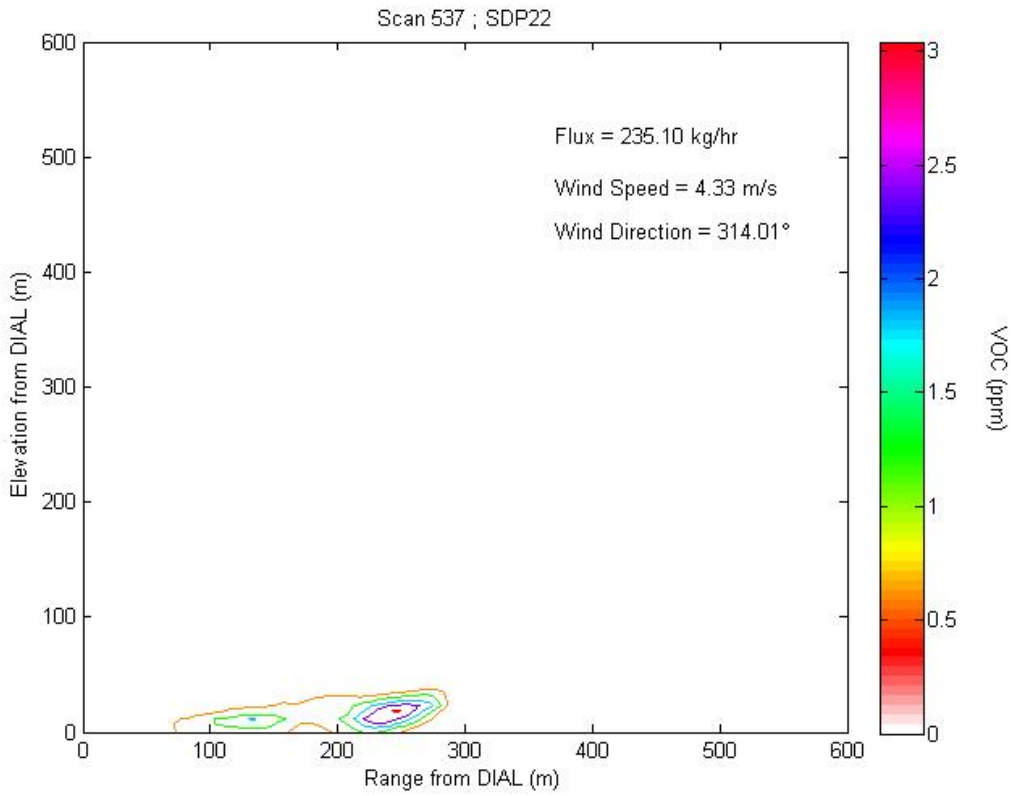
Figure 2.23a1 Contour plot of concentration profile for Scan 537 representing LOS1.
