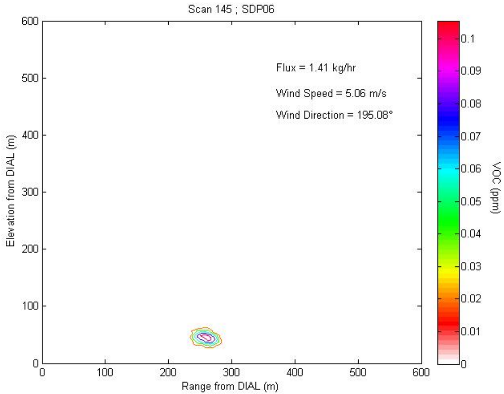
Figure 2.6a1 Contour plot of concentration profile for Scan 145 representing LOS1.
