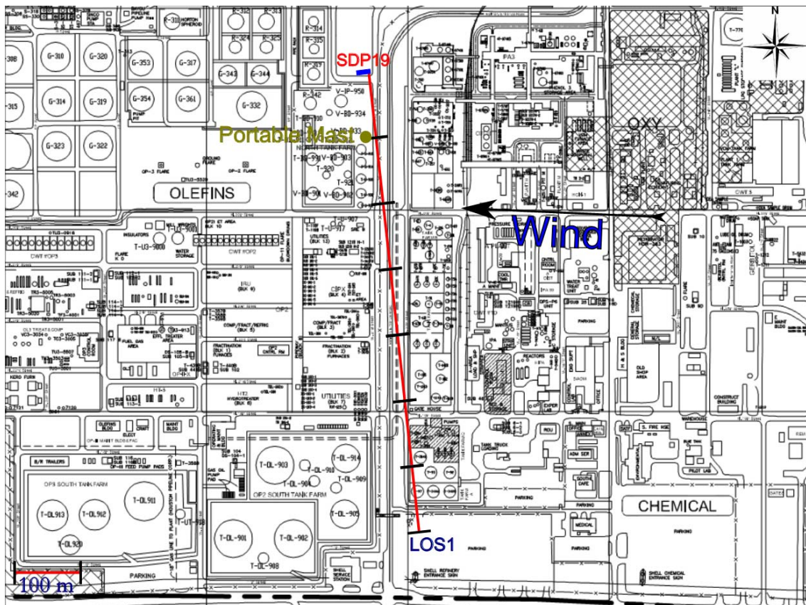
Figure 2.20 Measurement configuration for location SDP19 on 3 rd of February.
