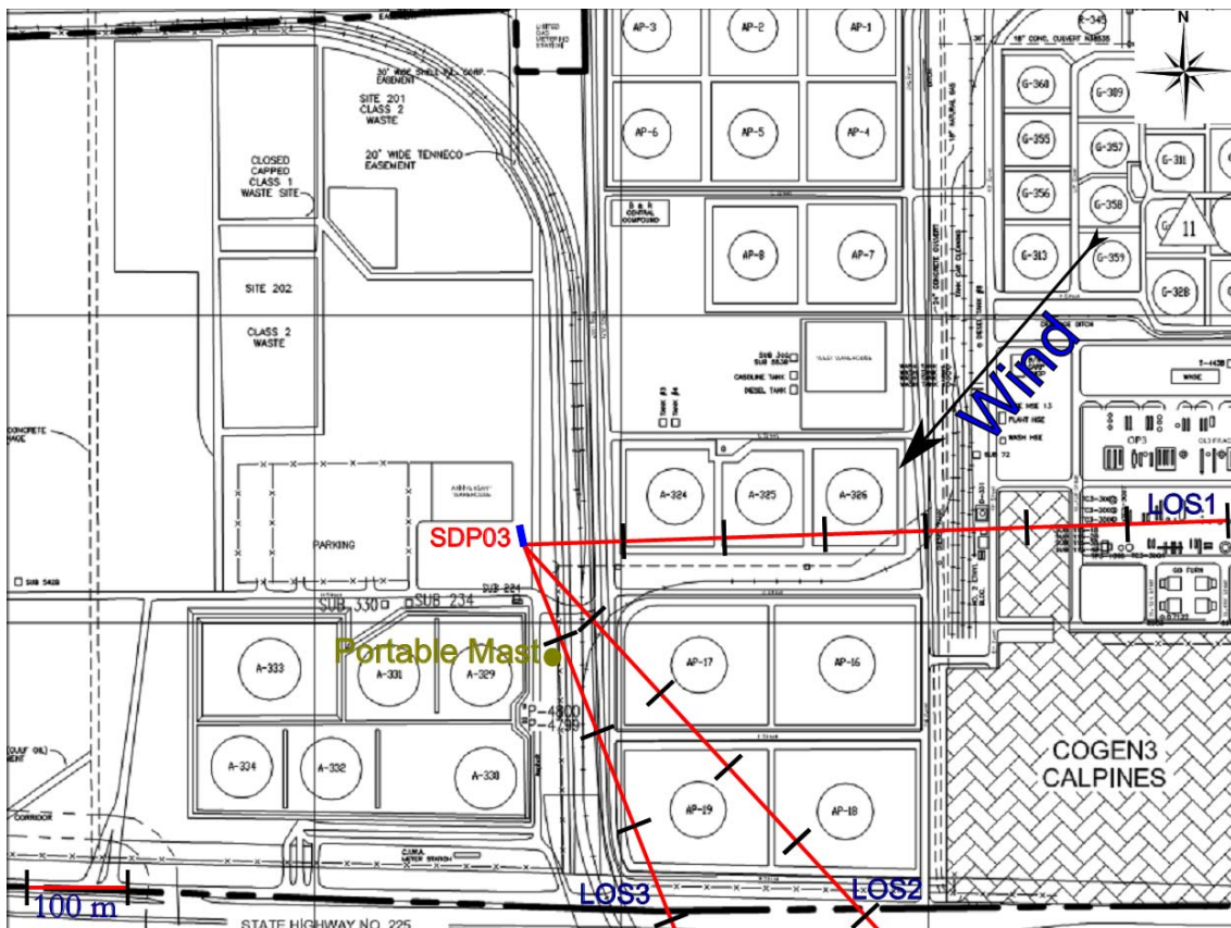
Figure 2.3 Measurement configuration for location SDP03 on 15 th of January.
