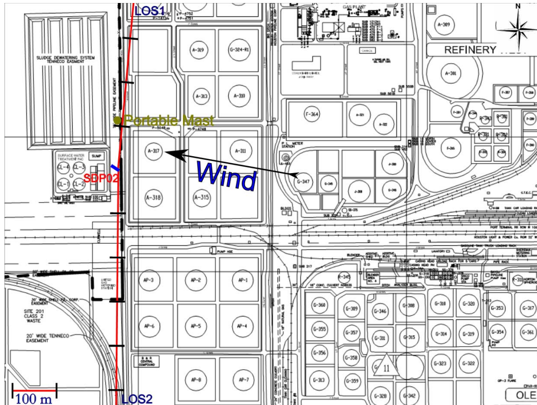
Figure 2.2 Measurement configuration for location SDP02 on 14 th of January.
