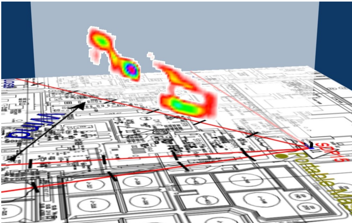
Figure 2.15b2 Visualisation of emission rate measured for Scan 366 representing LOS3.
