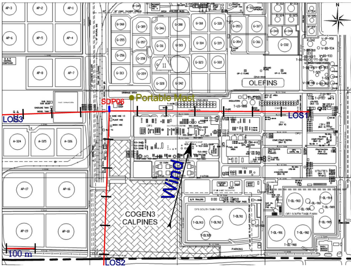
Figure 2.6 Measurement configuration for location SDP06 on 19 th of January.
