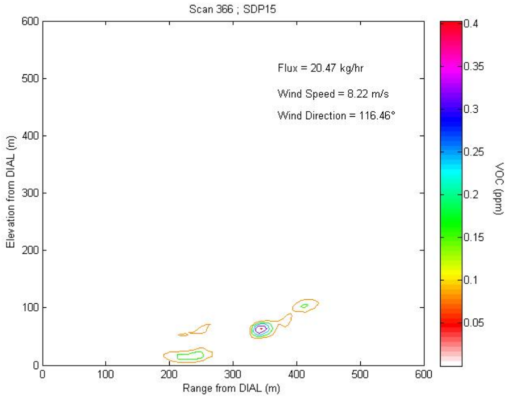
Figure 2.15b1 Contour plot of concentration profile for Scan 366 representing LOS3.
