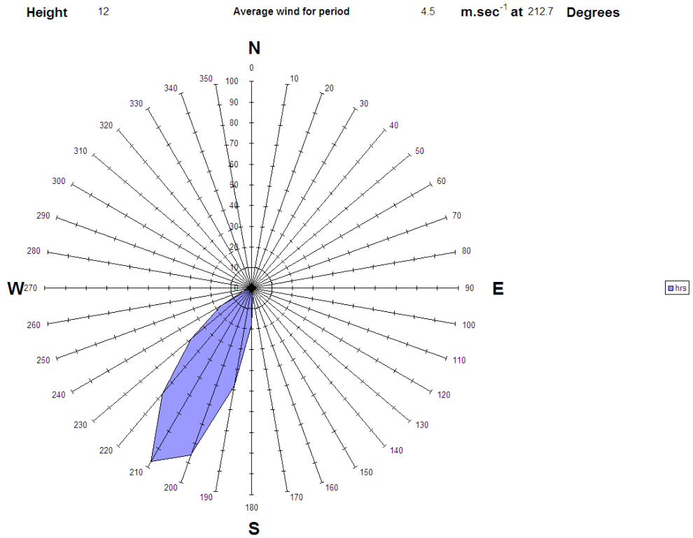
Figure A3.40 Wind rose for 27 th March during measurements from SDP37, 9:58 - 16:51
