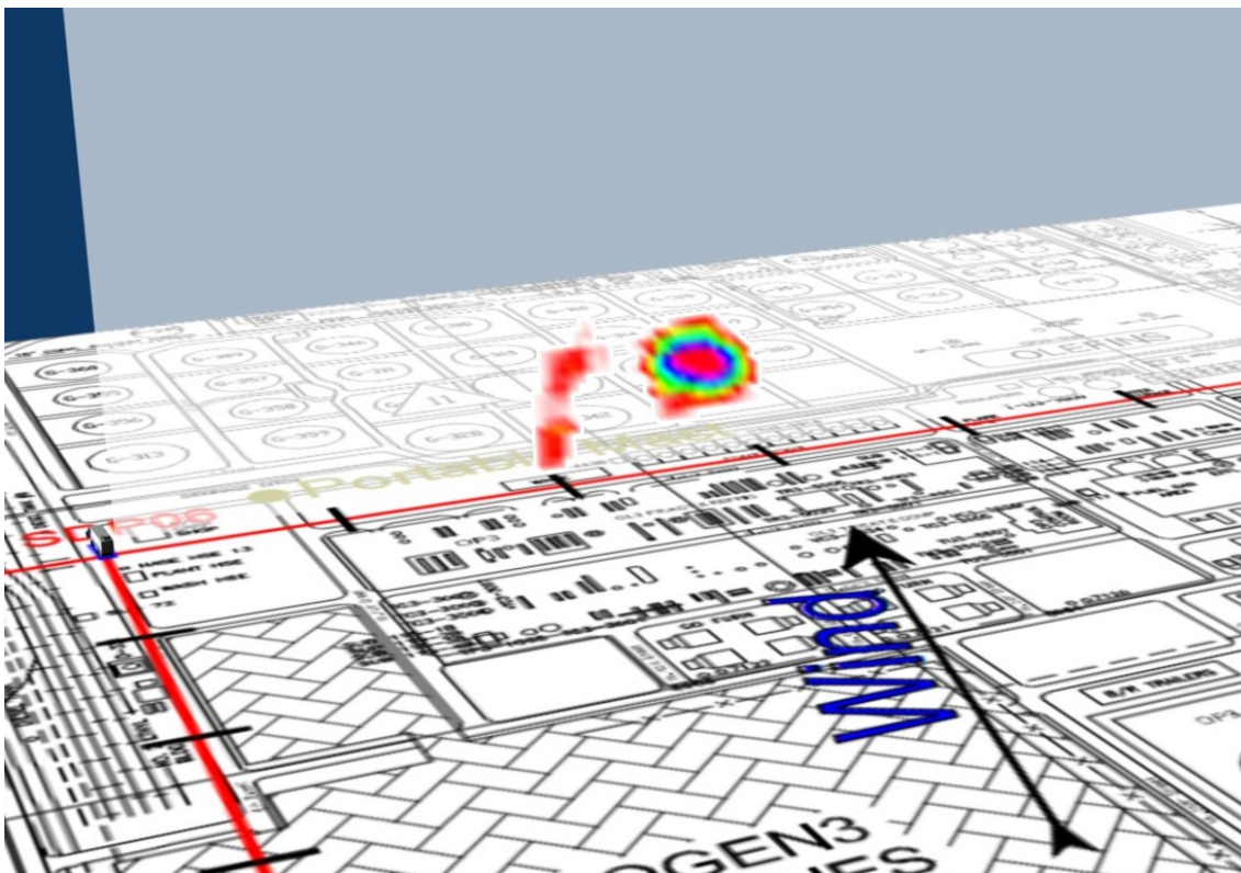
Figure 2.6a2 Visualisation of emission rate measured for Scan 145 representing LOS1.
