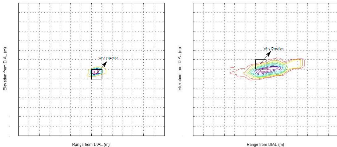
Figure A1.2 Illustration of the emission rate calculation approach
