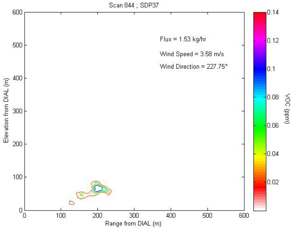
Figure 2.27a1 Contour plot of concentration profile for Scan 844 representing LOS1.
