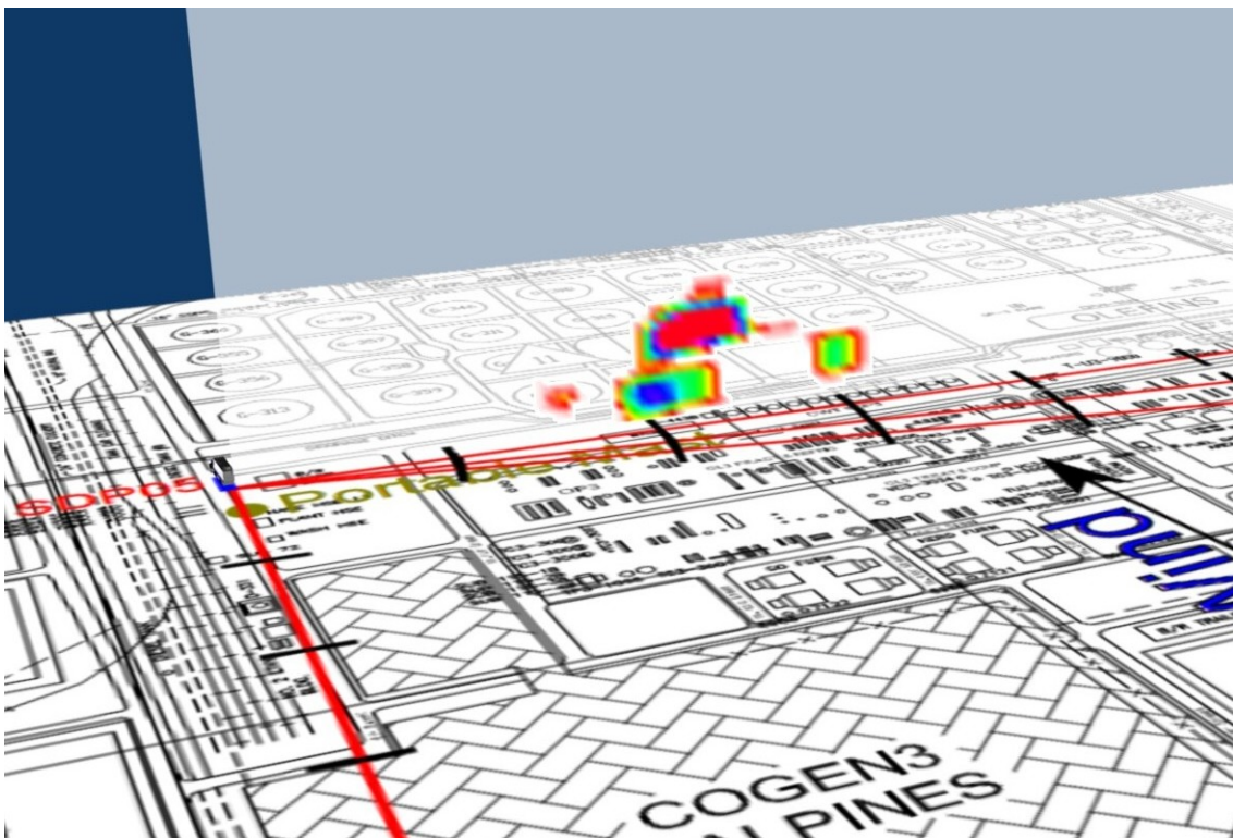
Figure 2.5a2 Visualisation of emission rate measured for Scan 115 representing LOS1.
