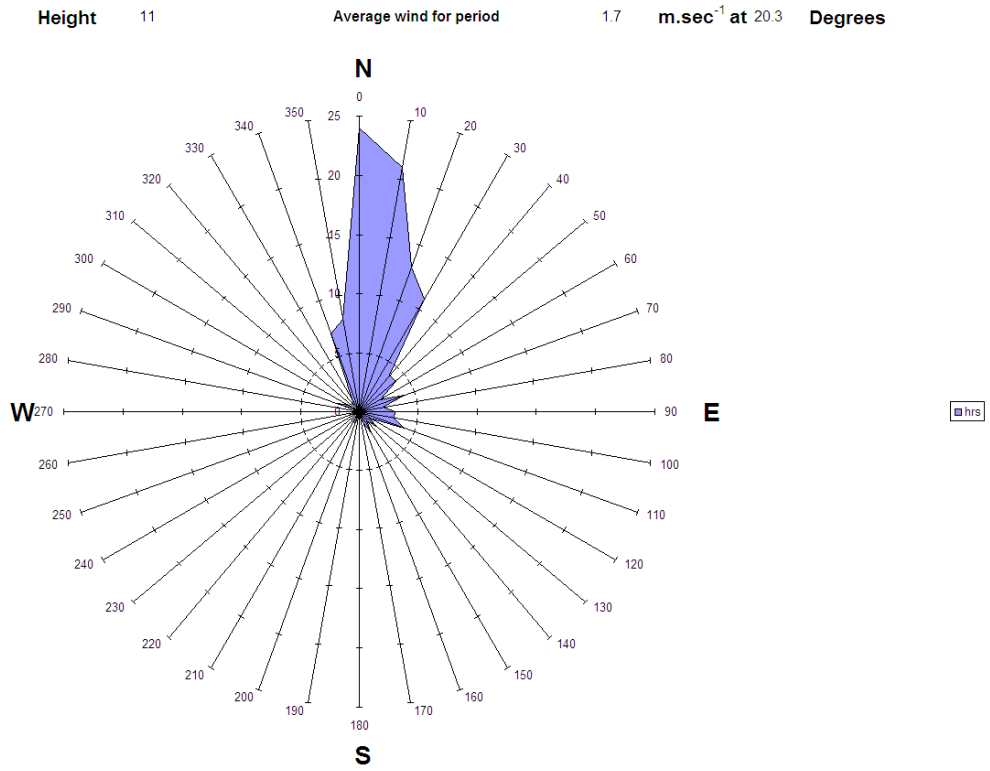
Figure A3.38 Wind rose for 26 th March during measurements from SDP35, 10:53 - 13:33
