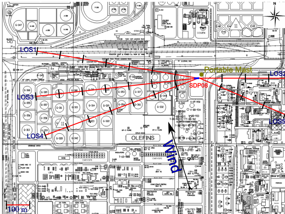
Figure 2.8 Measurement configuration for location SDP08 on 20 th of January.
