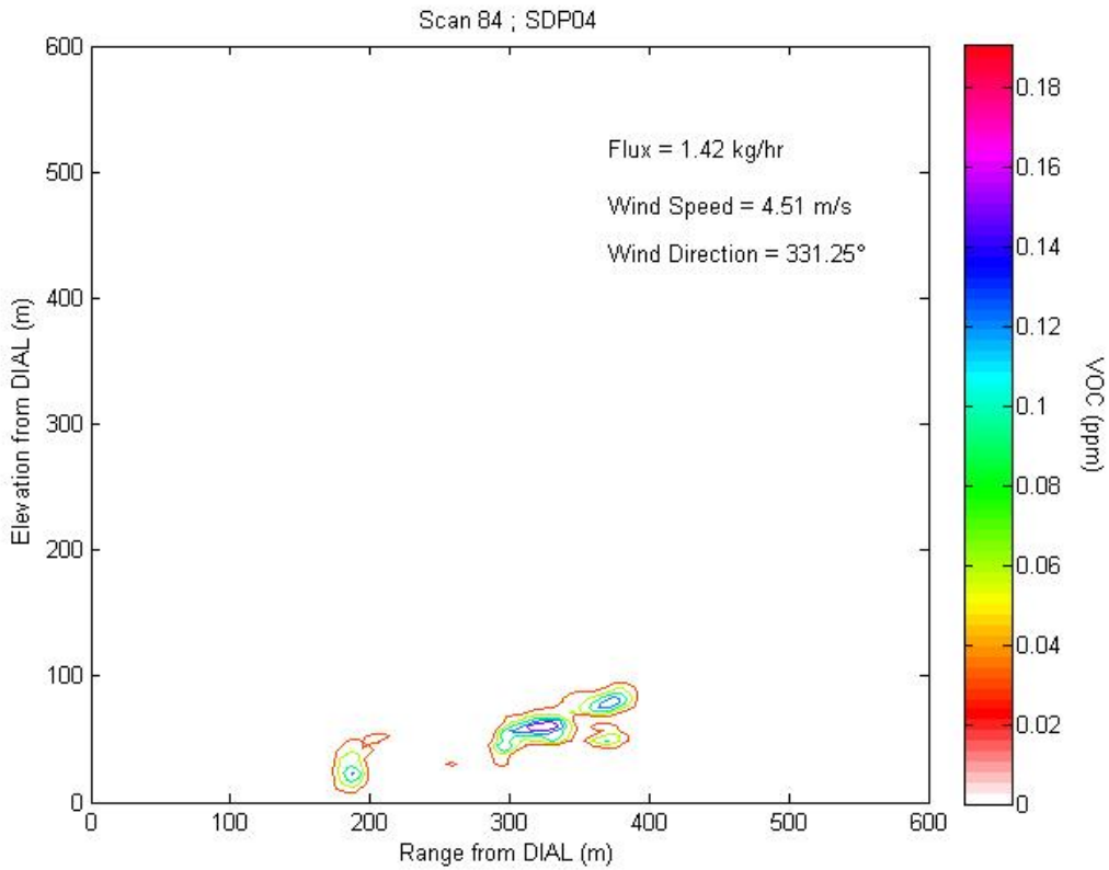
Figure 2.4a1 Contour plot of concentration profile for Scan 84 representing LOS1.
