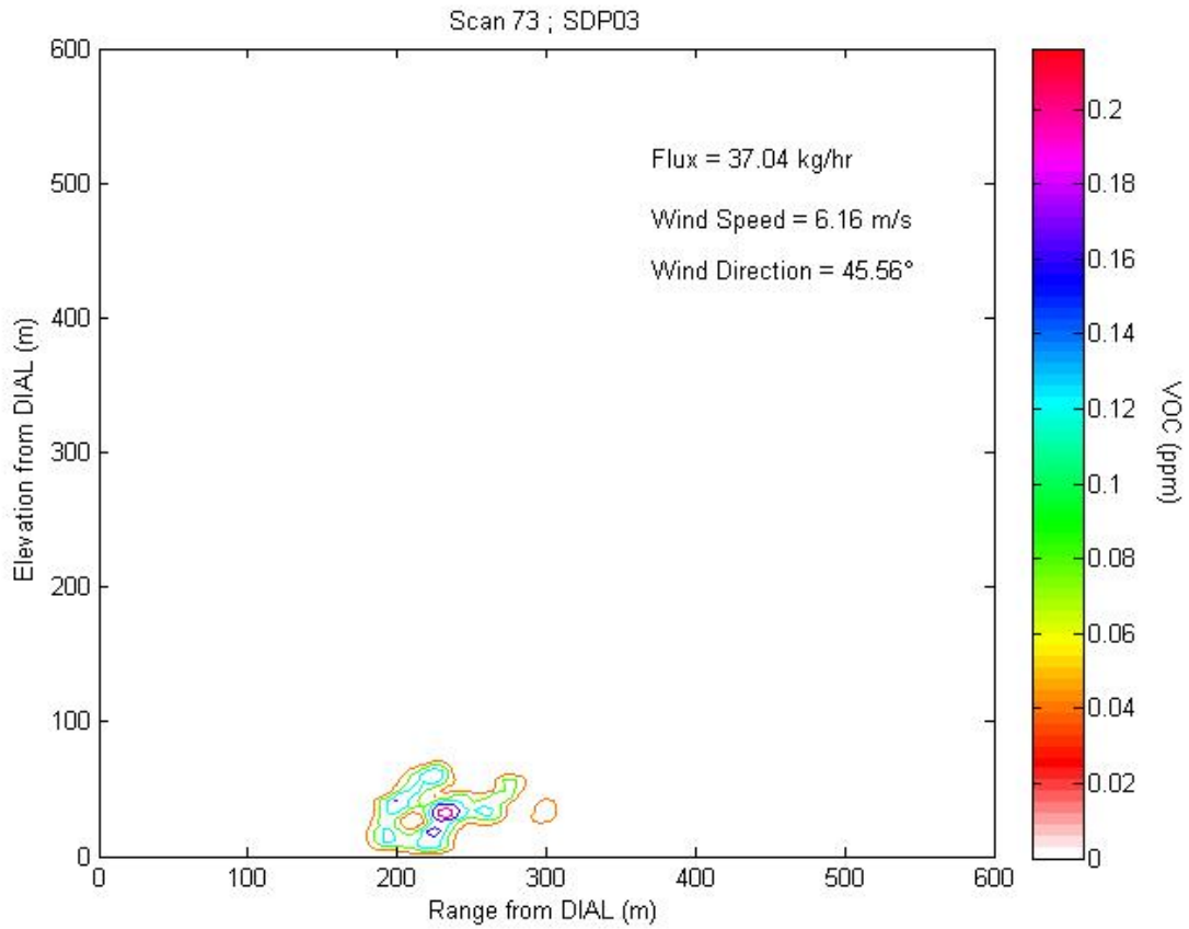
Figure 2.3b1 Contour plot of concentration profile for Scan 73 representing LOS2.
