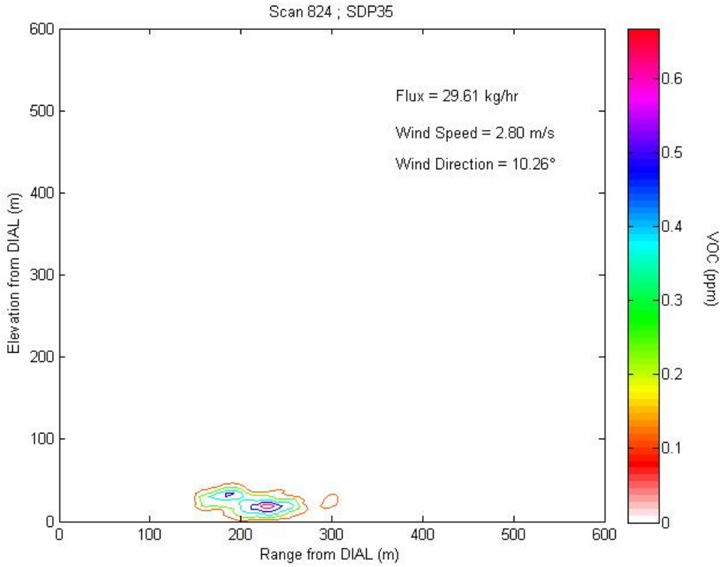
Figure 2.25a1 Contour plot of concentration profile for Scan 824 representing LOS1.
