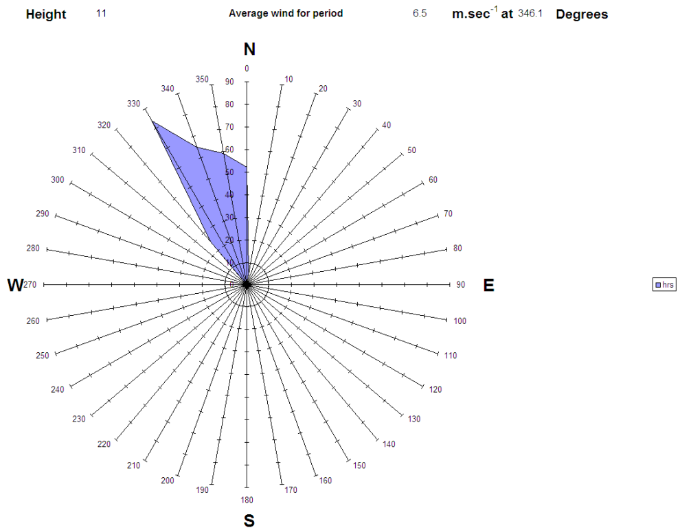
Figure A3.27 Wind rose for 9 th February during measurements from SDP25, 10:42 - 16:57
