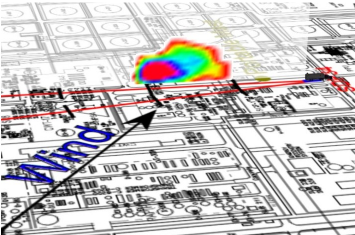
Figure 2.24a2 Visualisation of emission rate measured for Scan 809 representing LOS1.
