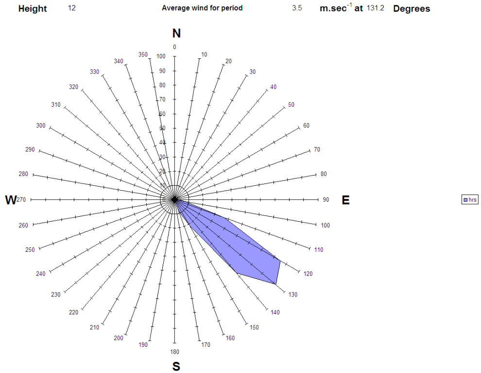
Figure A3.12 Wind rose for 23 rd January during measurements from SDP11, 10:57 - 17:06
