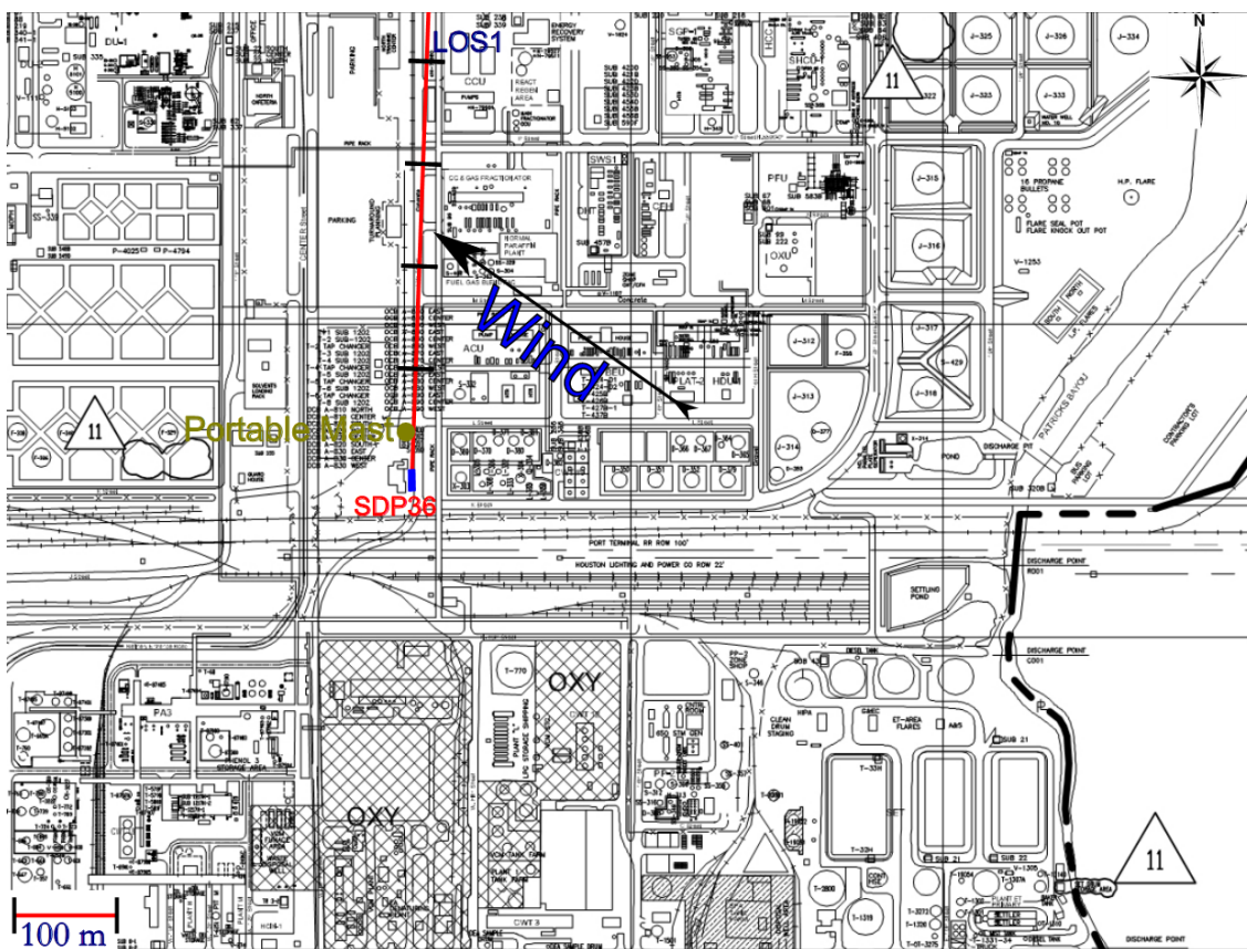
Figure 2.26 Measurement configuration for location SDP36 on 26 th of March.
