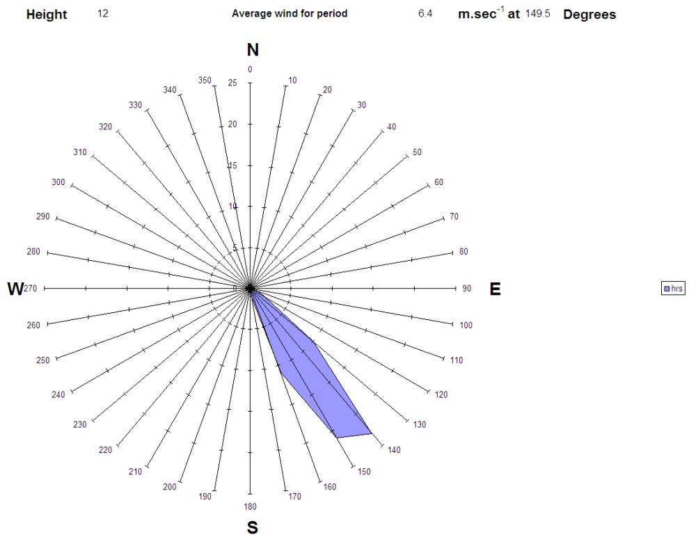
Figure A3.25 Wind rose for 8 th February during measurements from SDP23, 10:55 - 12:07
