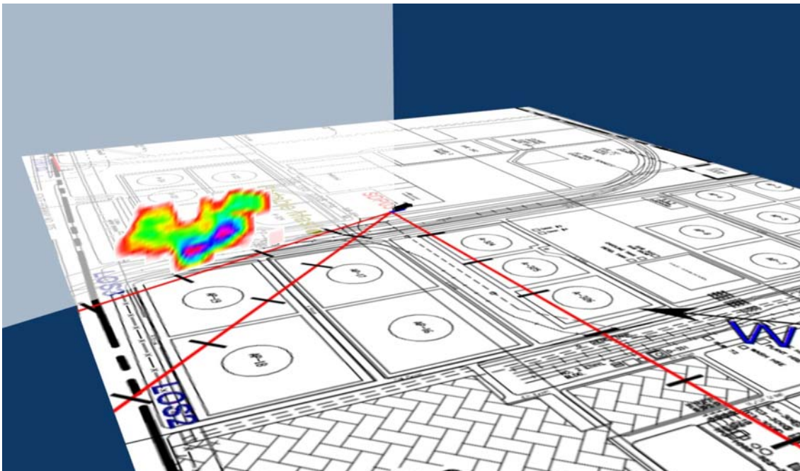
Figure 2.3c2 Visualisation of emission rate measured for Scan 77 representing LOS3.
