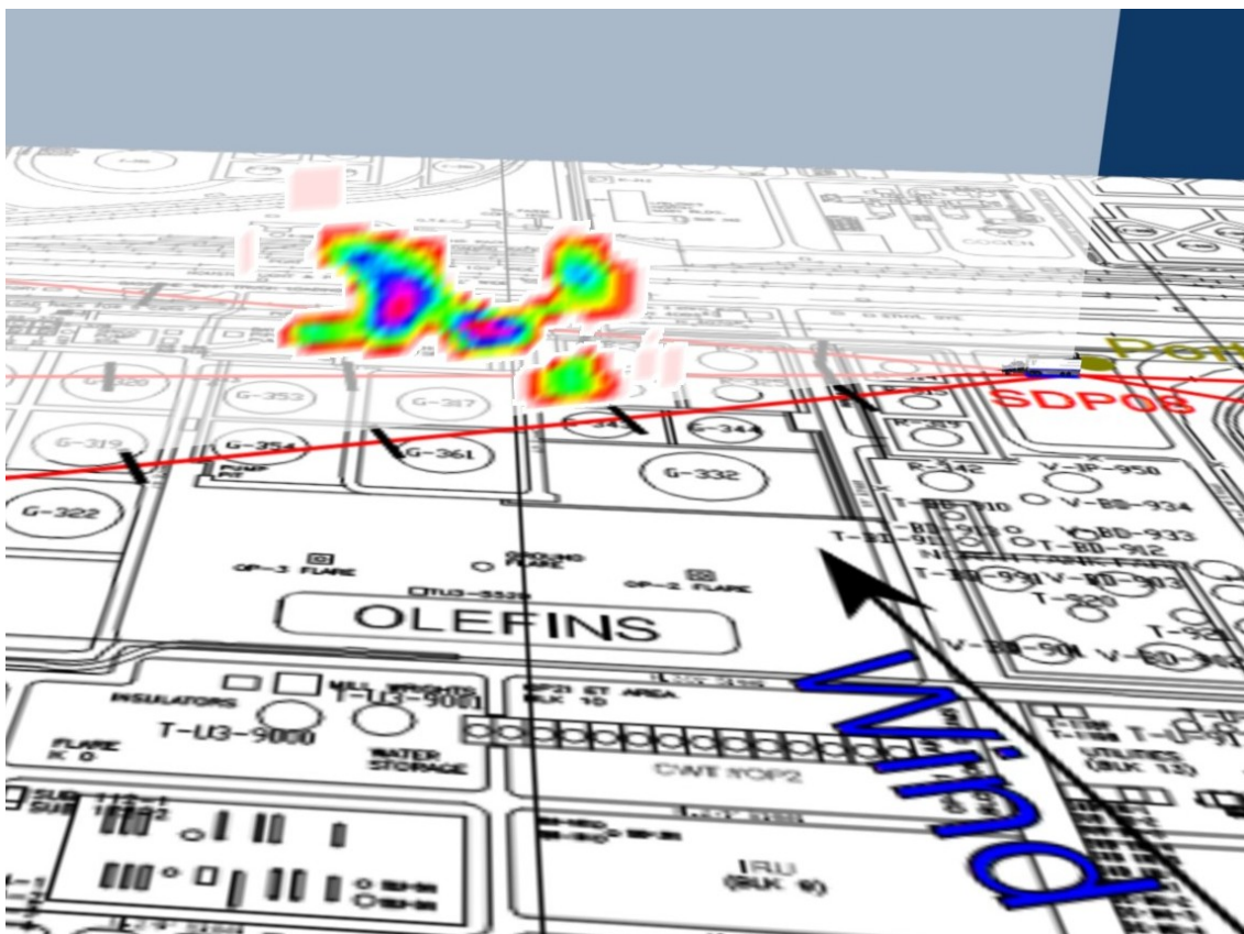
Figure 2.8b2 Visualisation of emission rate measured for Scan 193 representing LOS4.
