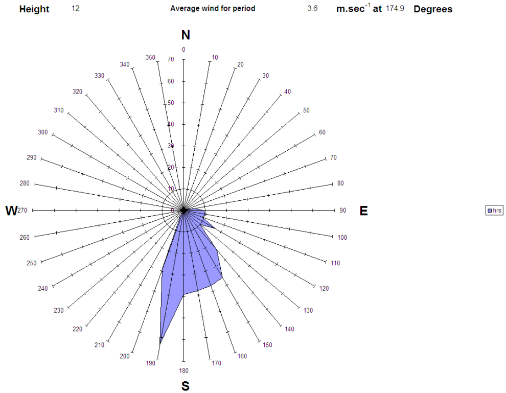
Figure A3.6 Wind rose for 18 th January during measurements from SDP5, 10:46 - 16:50
