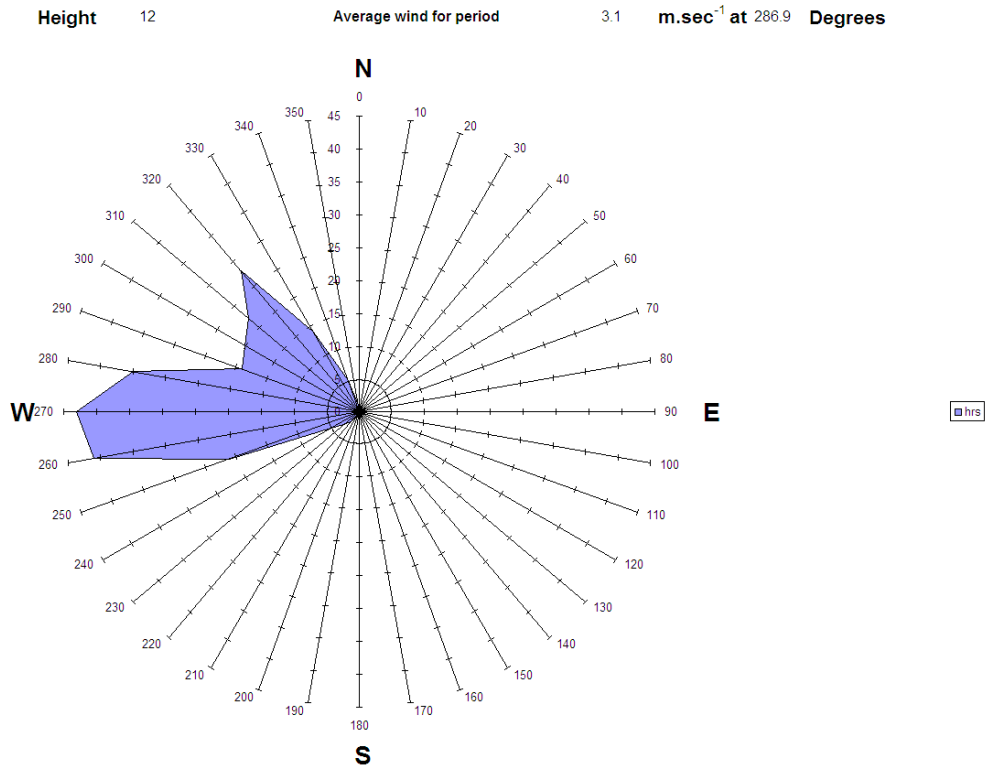
Figure A3.10 Wind rose for 21 st January during measurements from SDP9, 11:57 - 16:55
