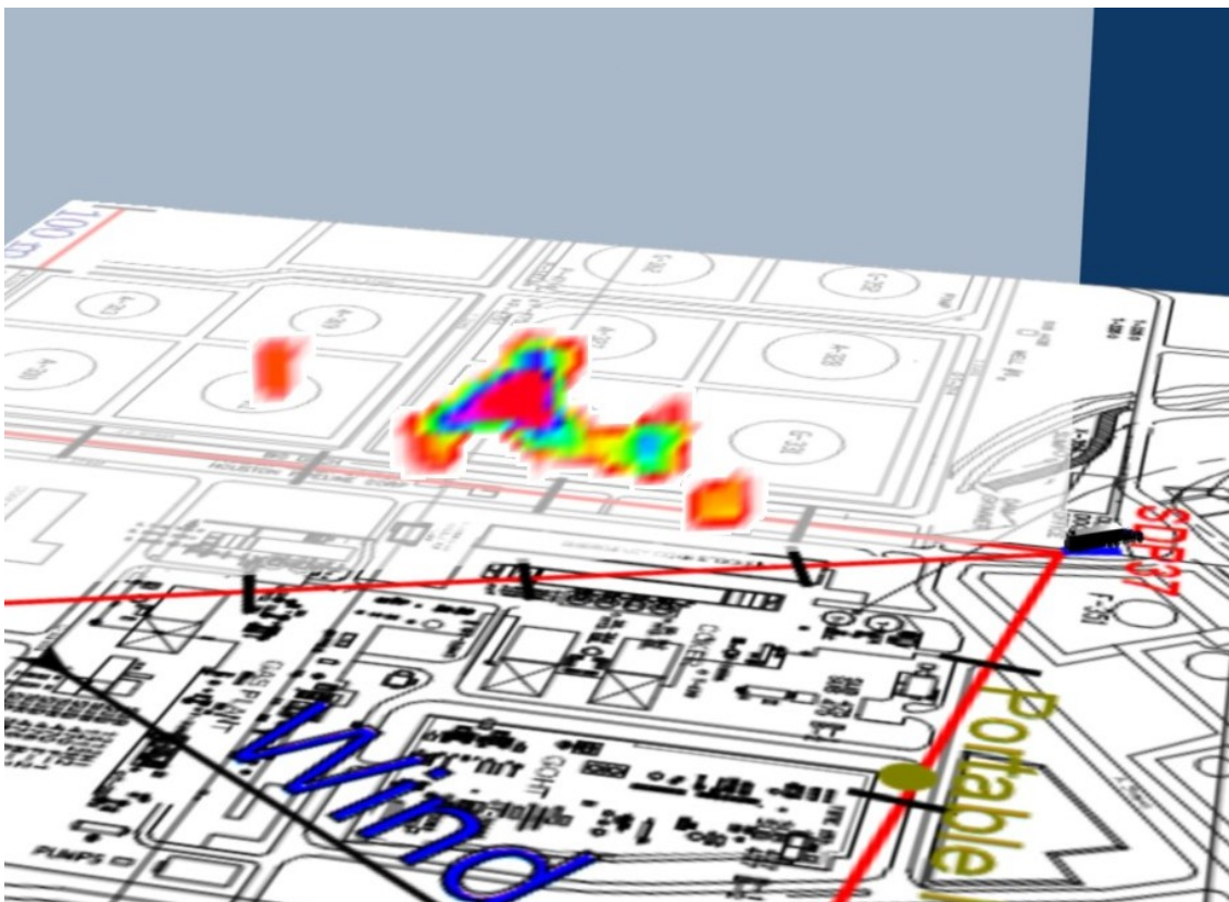
Figure 2.27a2 Visualisation of emission rate measured for Scan 844 representing LOS1.
