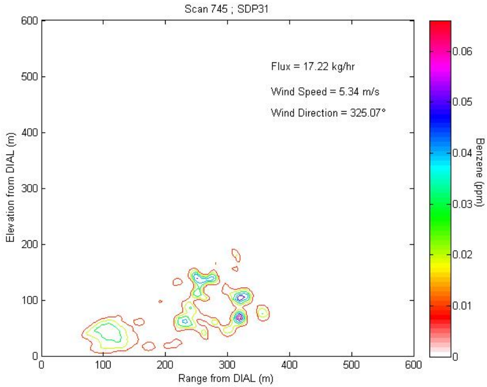
Figure 3.10a1 Contour plot of concentration profile for Scan 745 representing LOS3.
