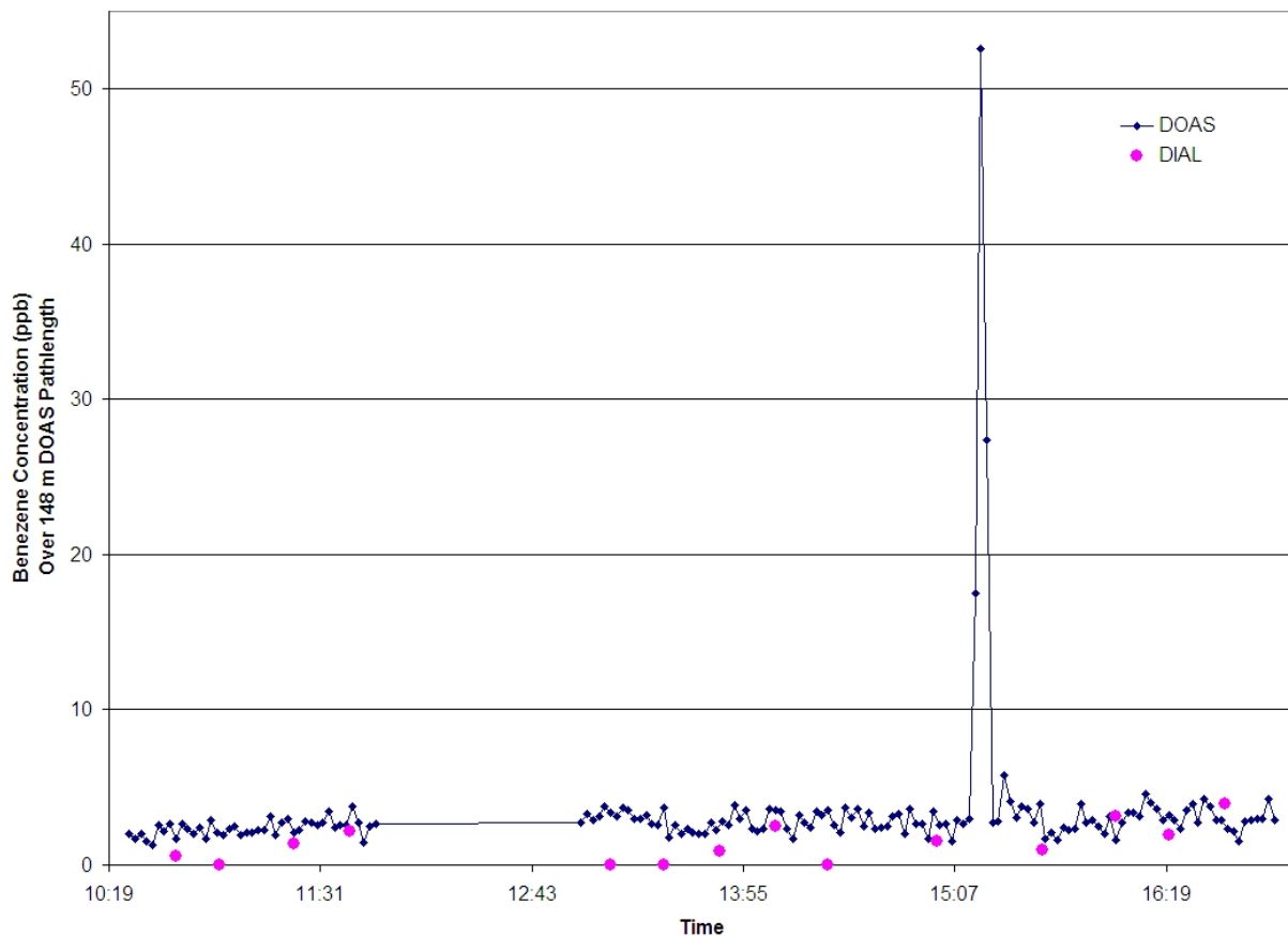
Figure 5.4 DIAL and DOAS measurements comparison on the 9 th of February.
