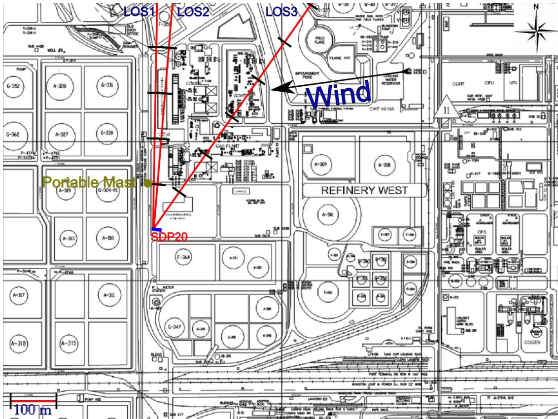
Figure 2.21 Measurement configuration for location SDP20 on 4 th of February.
