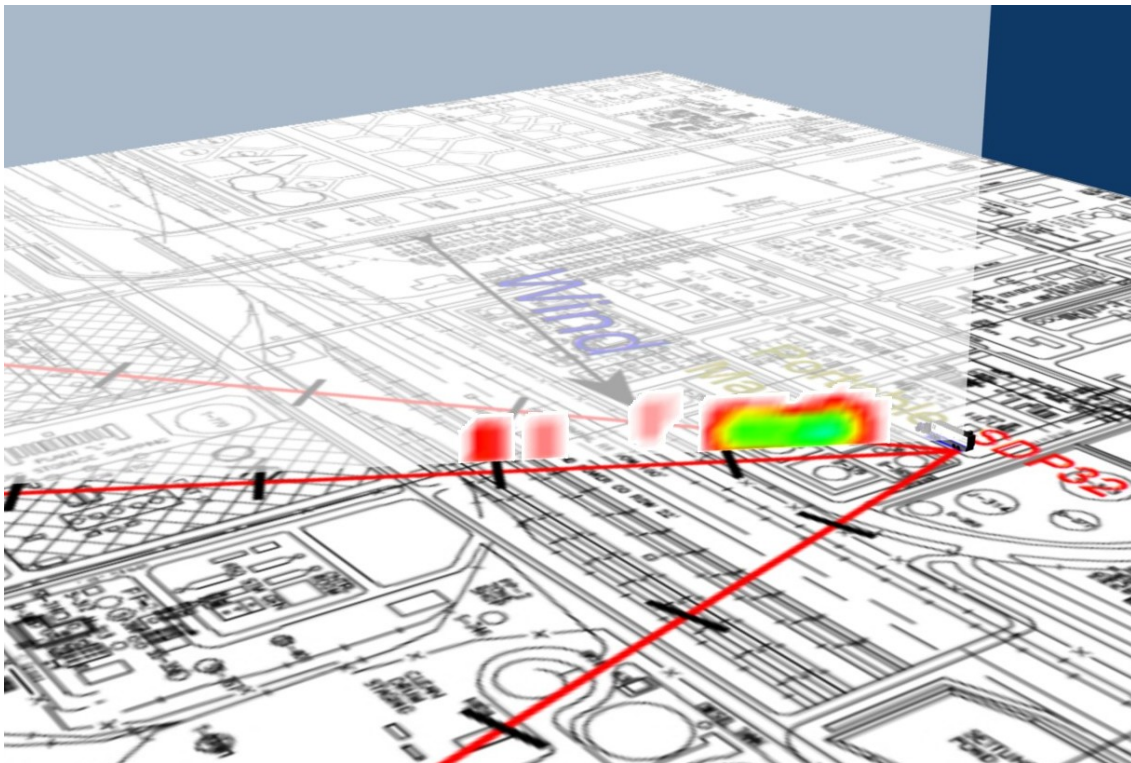
Figure 3.11a2 Visualisation of emission rate measured for Scan 768 representing LOS1.
