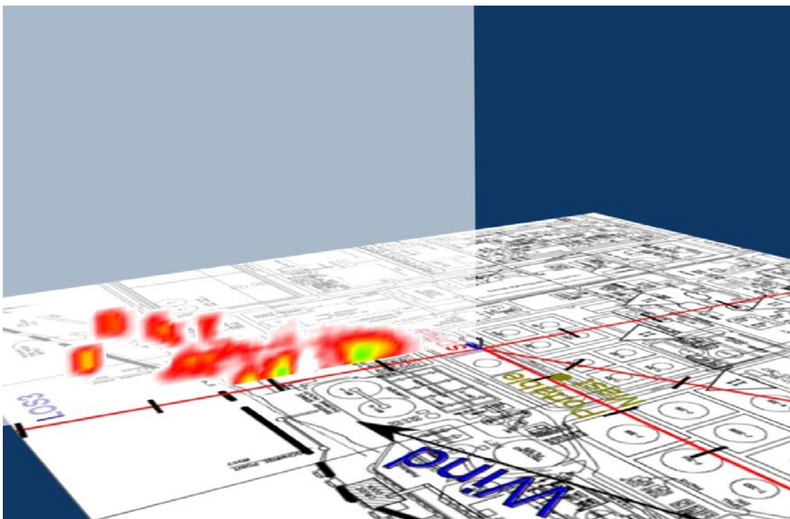
Figure 3.7b2 Visualisation of emission rate measured for Scan 672 representing LOS3.
