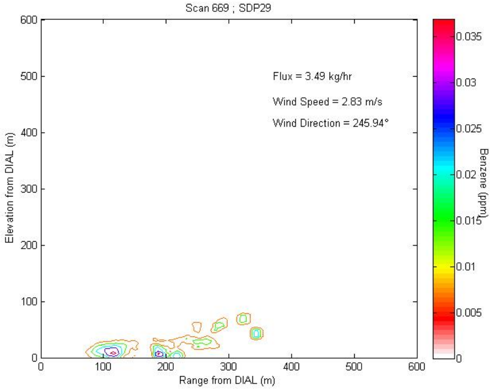
Figure 3.7a1 Contour plot of concentration profile for Scan 669 representing LOS2.
