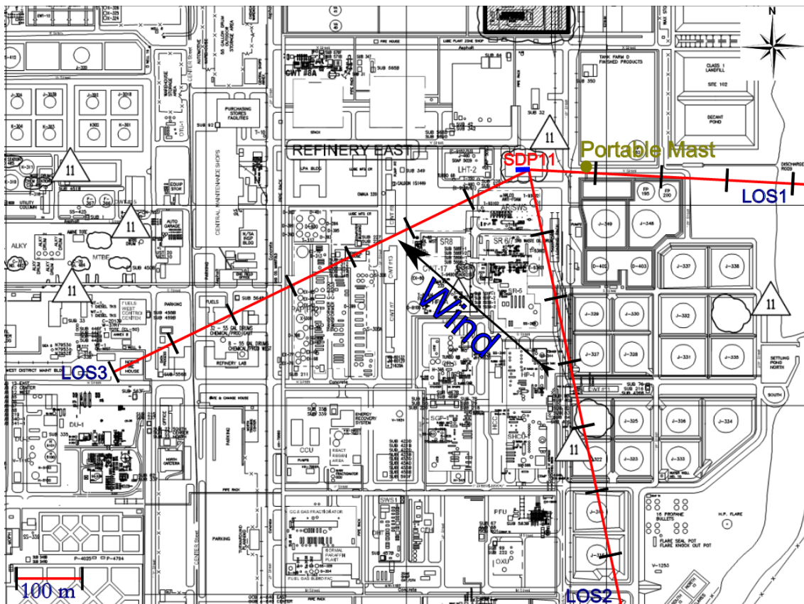
Figure 2.11 Measurement configuration for location SDP11 on 23 rd of January.
