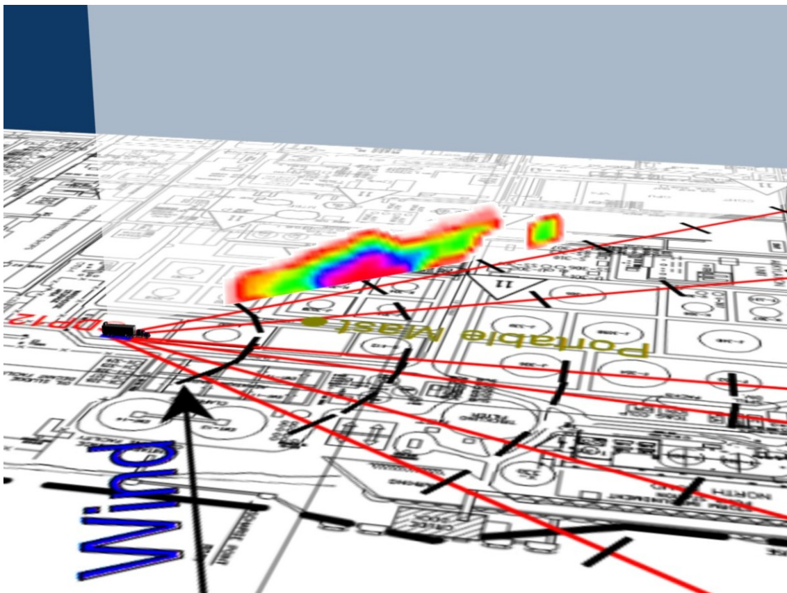
Figure 2.17a2 Visualisation of emission rate measured for Scan 401 representing LOS1.
