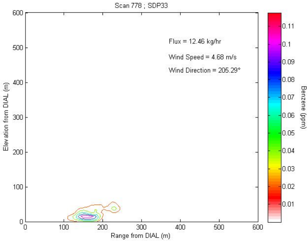
Figure 3.12a1 Contour plot of concentration profile for Scan 778 representing LOS1.
