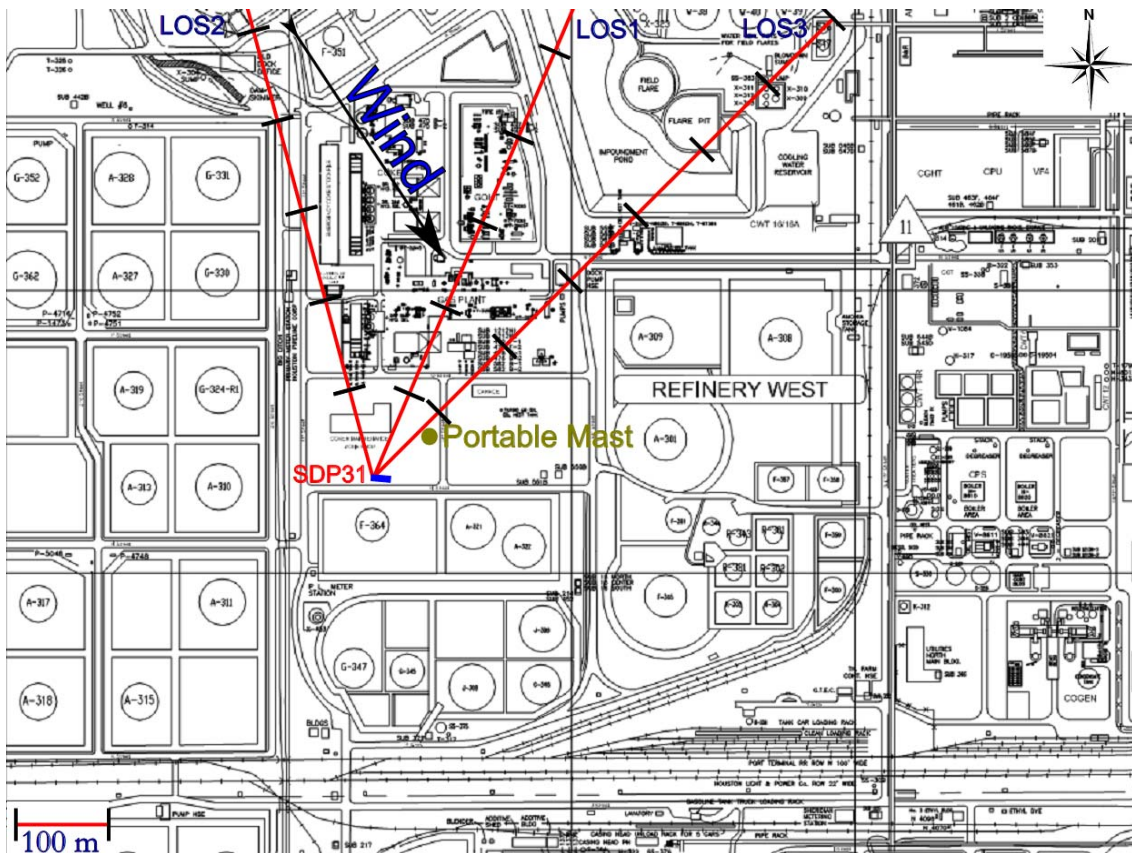
Figure 3.10 Measurement configuration for location SDP31 on 17 th of February.
