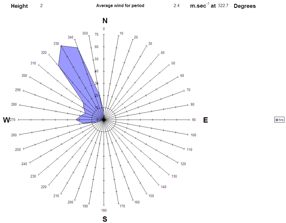
Figure A3.33 Wind rose for 16 th February during measurements from SDP30, 10:06 - 16:43
