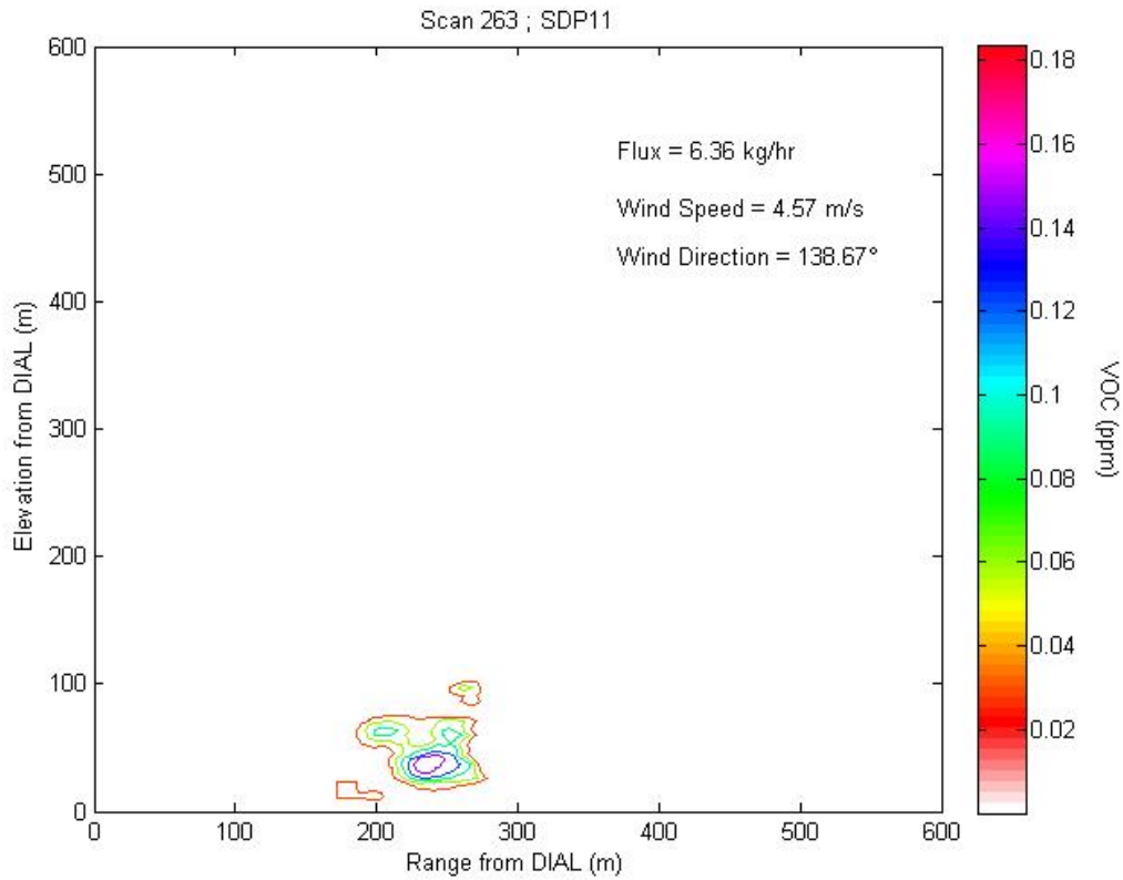
Figure 2.11a1 Contour plot of concentration profile for Scan 263 representing LOS2.
