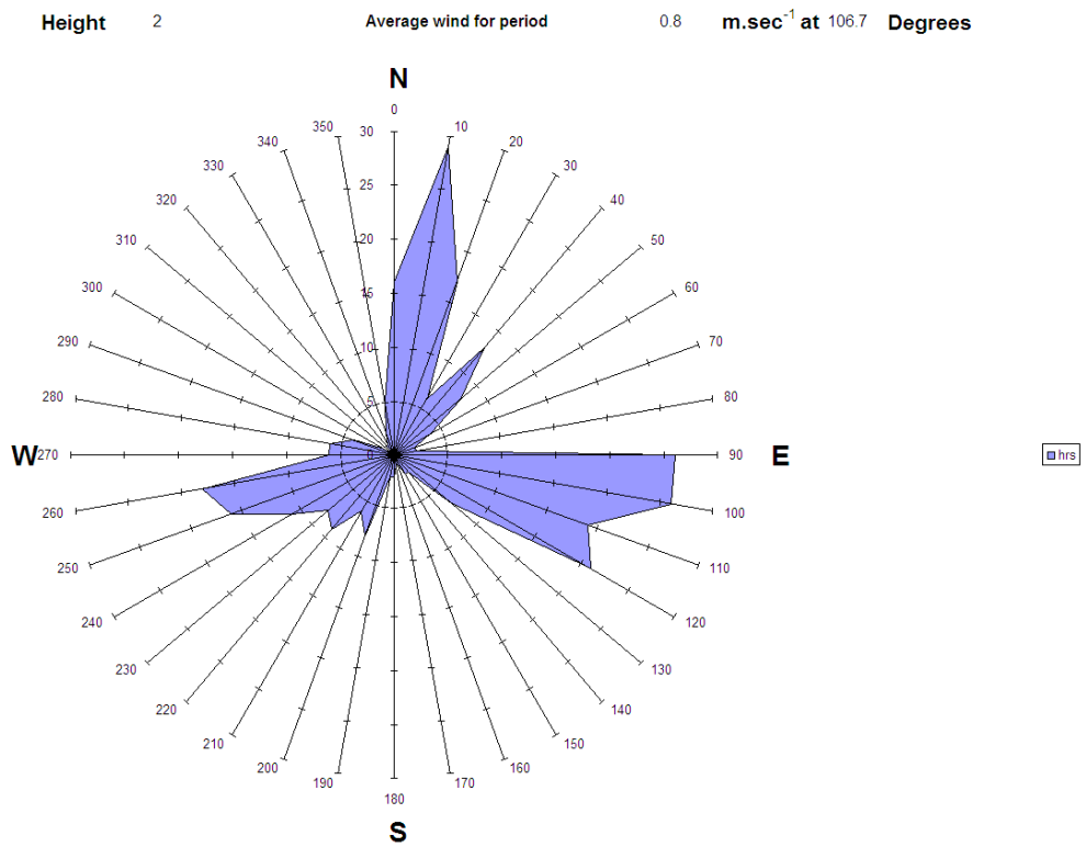
Figure A3.13 Wind rose for 25 th January during measurements from SDP12, 10:42 - 17:01
