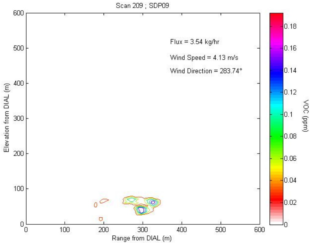
Figure 2.9a1 Contour plot of concentration profile for Scan 209 representing LOS2.
