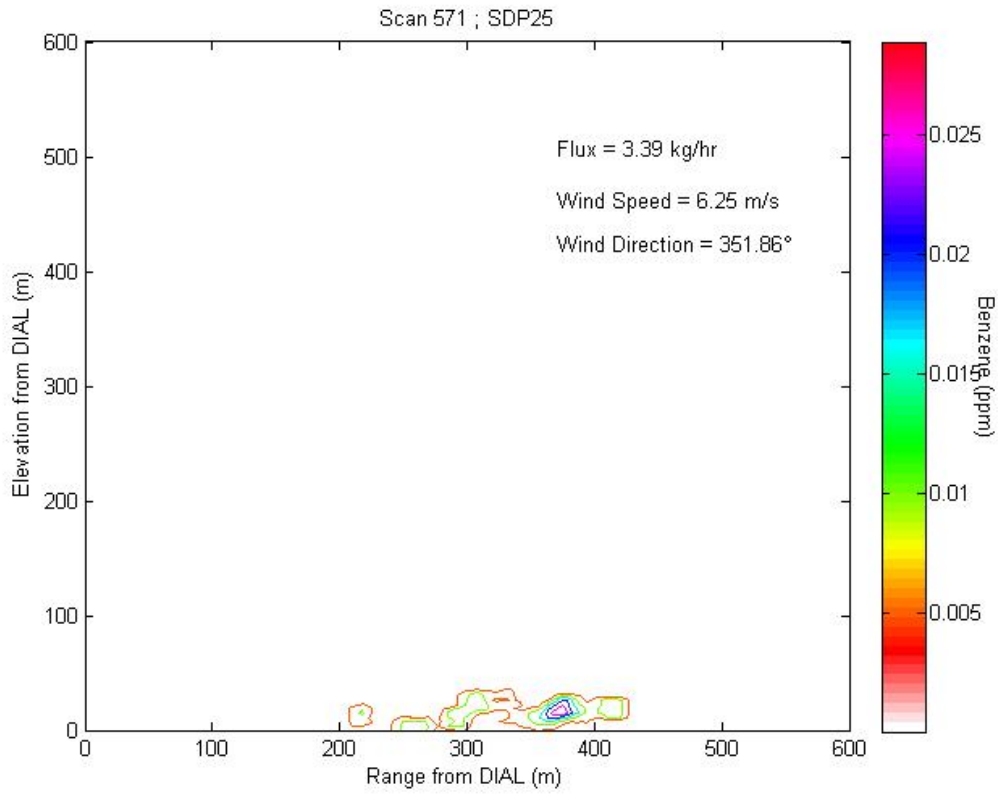
Figure 3.3a1 Contour plot of concentration profile for Scan 571 representing LOS1.
