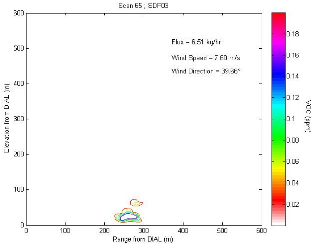
Figure 2.3a1 Contour plot of concentration profile for Scan 65 representing LOS1.
