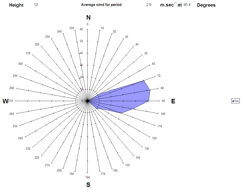
Figure A3.19 Wind rose for 1 st February during measurements from SDP17, 12:16 - 17:05
