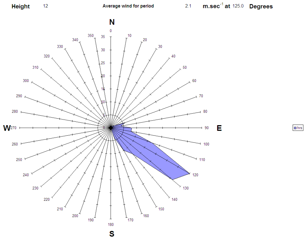
Figure A3.39 Wind rose for 26 th March during measurements from SDP36, 14:38 - 17:05
