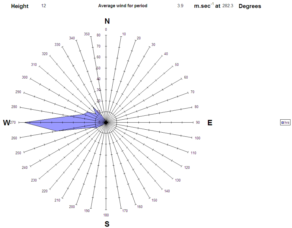
Figure A3.35 Wind rose for 22 nd March during measurements from SDP32, 12:29 - 17:24
