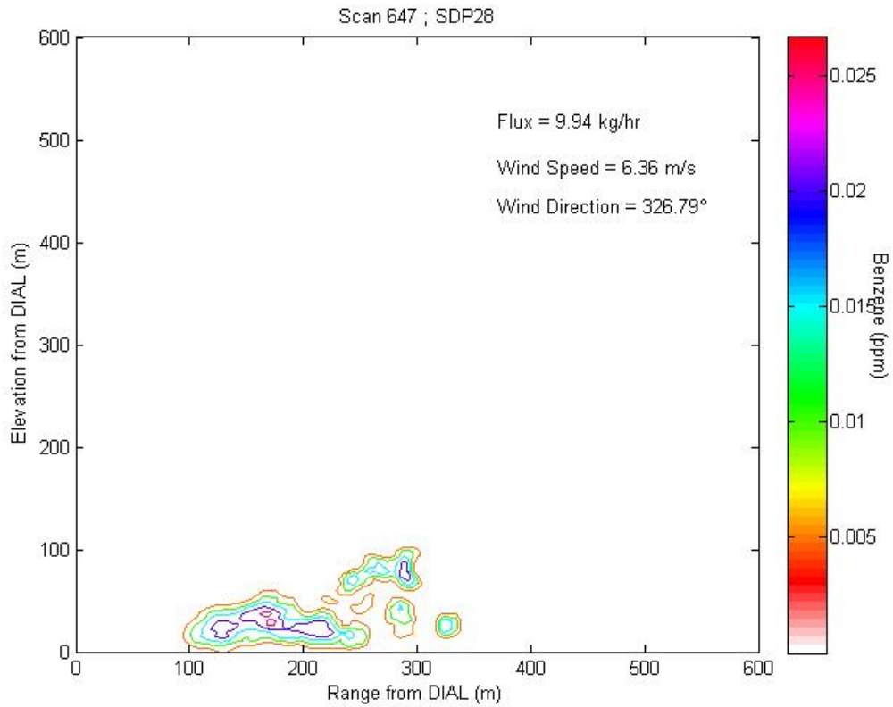
Figure 3.6a1 Contour plot of concentration profile for Scan 647 representing LOS1.
