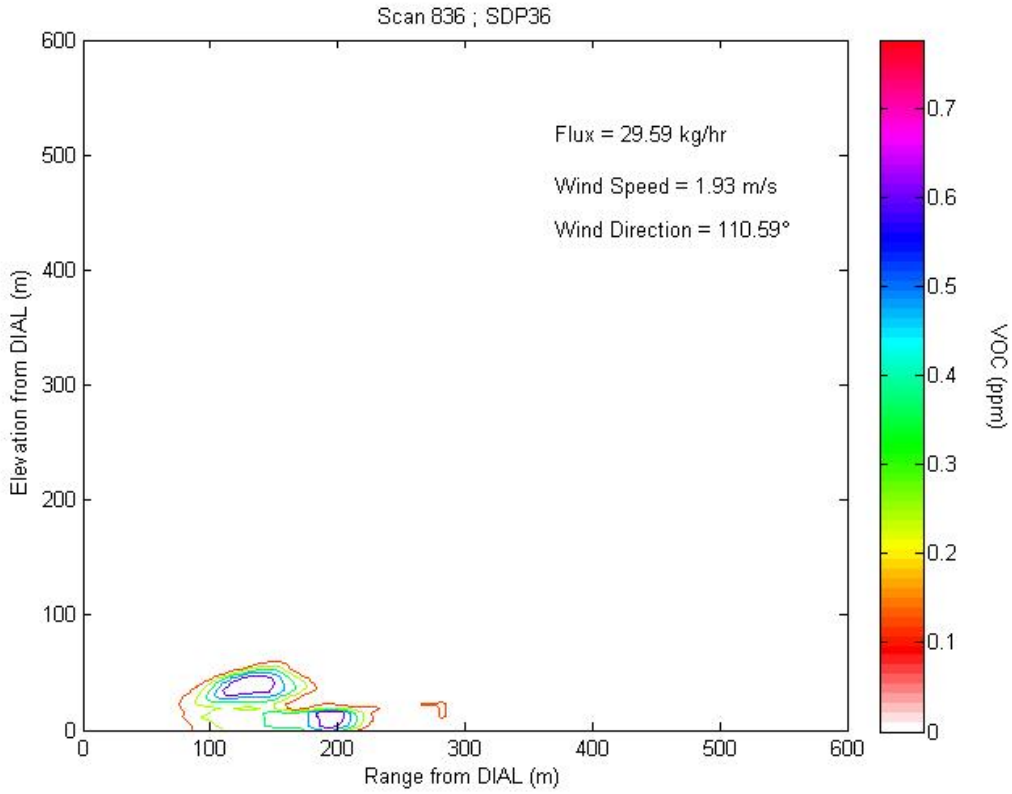
Figure 2.26a1 Contour plot of concentration profile for Scan 836 representing LOS1.
