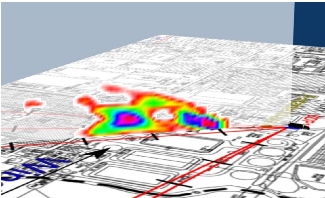
Figure 2.18a2 Visualisation of emission rate measured for Scan 422 representing LOS1.
