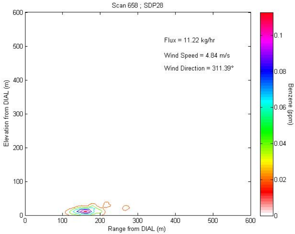
Figure 3.6b1 Contour plot of concentration profile for Scan 658 representing LOS2.
